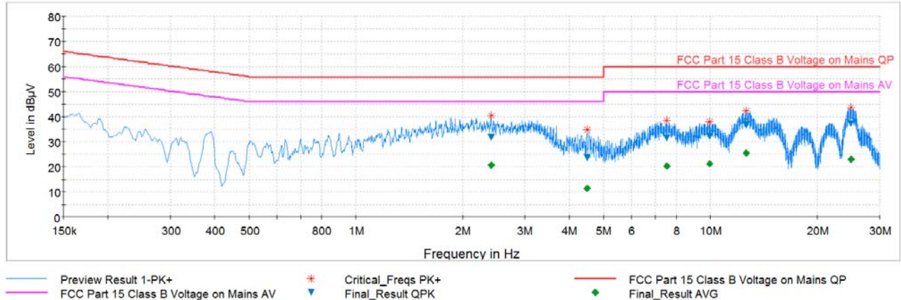
Plot 6-35. Line Conducted Plot with 802.11b (L1)
