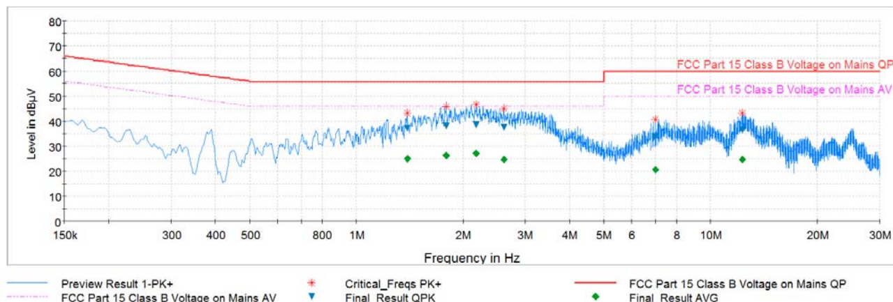
Plot 6-36. Line Conducted Plot with 802.11b (N)
