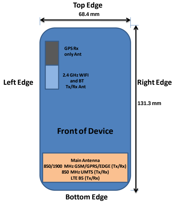
Figure F-1 DUT Antenna Locations
