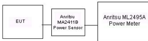
Figure 9-3 Power Measurement Setup for Bandwidths
