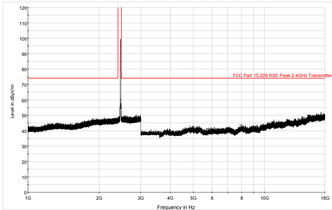
Plot 6-35. 1GHz – 18GHz Horizontal Pre-Scan Plot (802.11b – Ch. 11)
