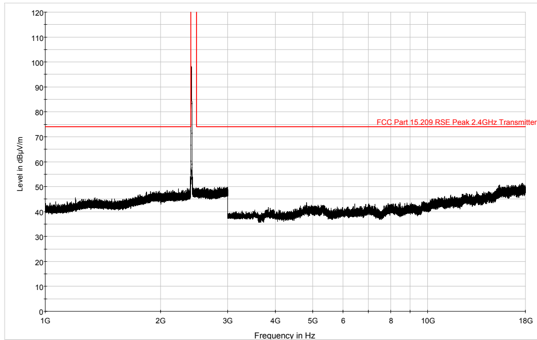
Plot 6-31. 1GHz – 18GHz Horizontal Pre-Scan Plot (802.11b – Ch. 1)
