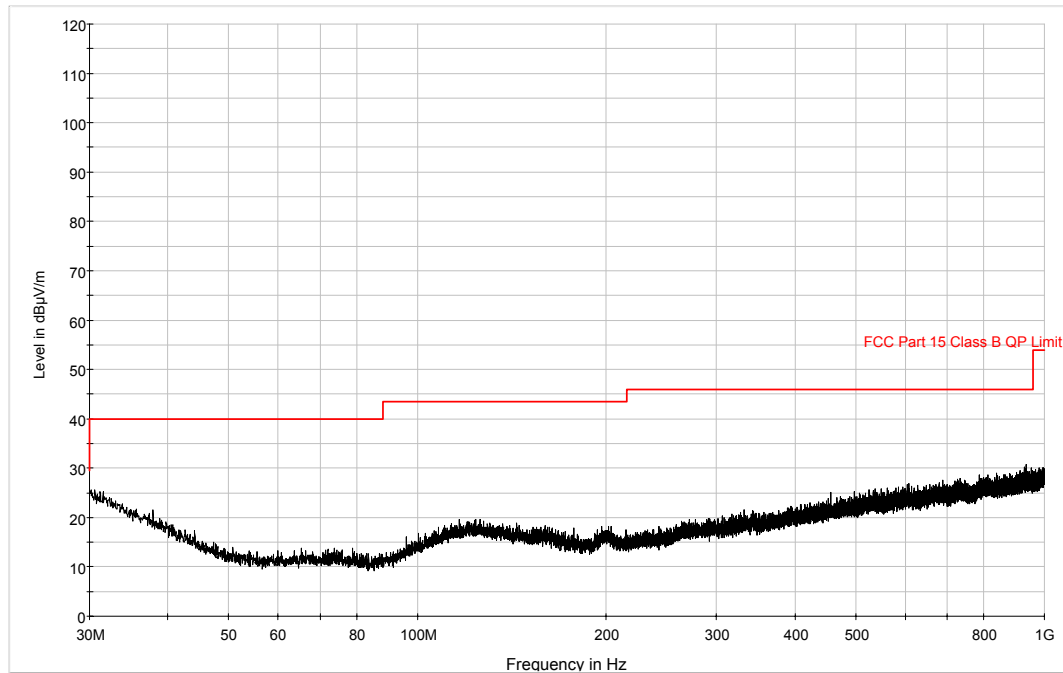
Plot 6-37. 30MHz – 1GHz Horizontal Pre-Scan Plot (802.11b – Ch. 6)
