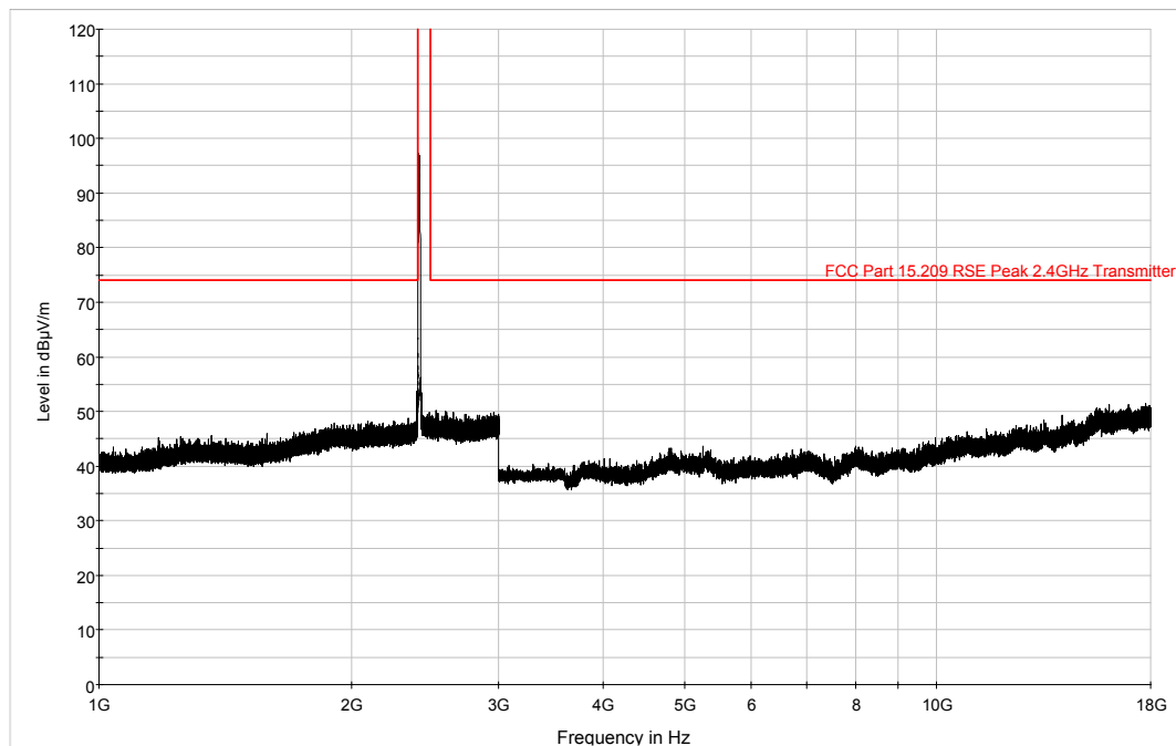
Plot 6-32. 1GHz – 18GHz Vertical Pre-Scan Plot (802.11b – Ch. 1)
