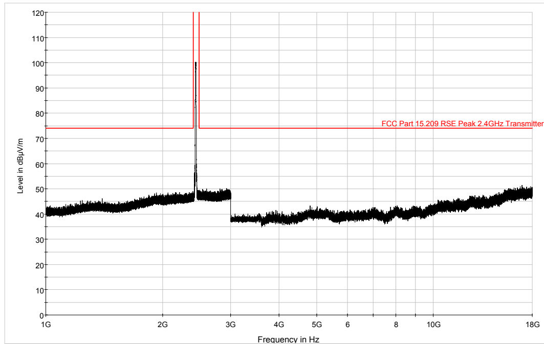
Plot 6-33. 1GHz – 18GHz Horizontal Pre-Scan Plot (802.11b – Ch. 6)
