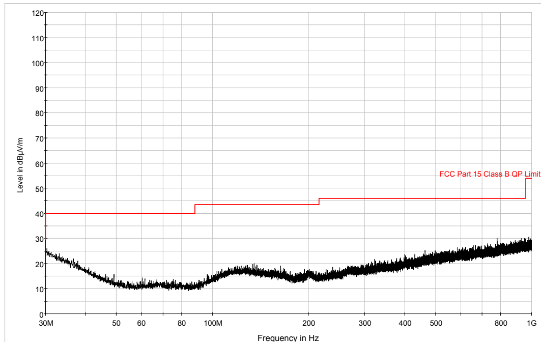
Plot 6-38. 30MHz – 1GHz Vertical Pre-Scan Plot (802.11b – Ch. 6)
