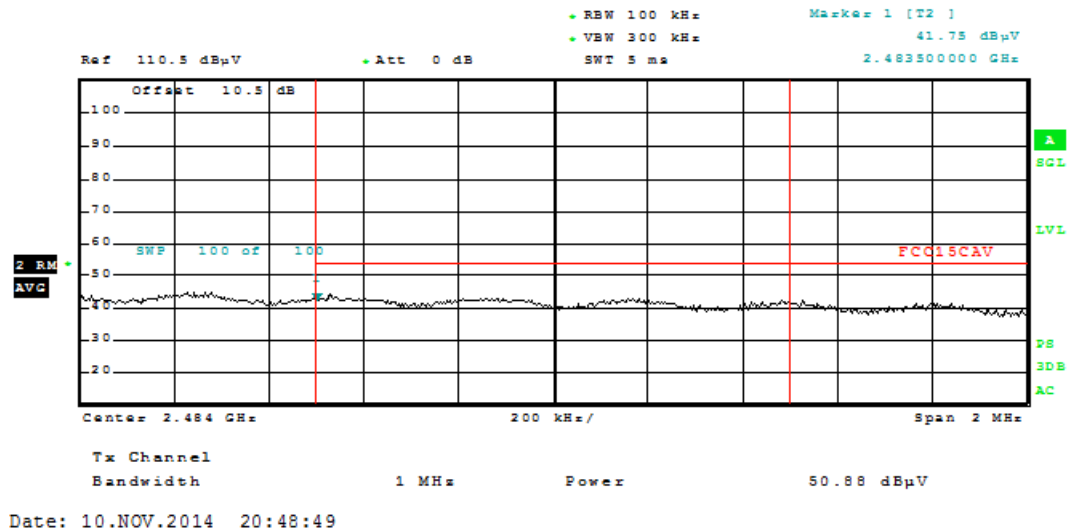
Plot 6-41. Radiated Restricted Upper Band Edge Measurement (Average)
