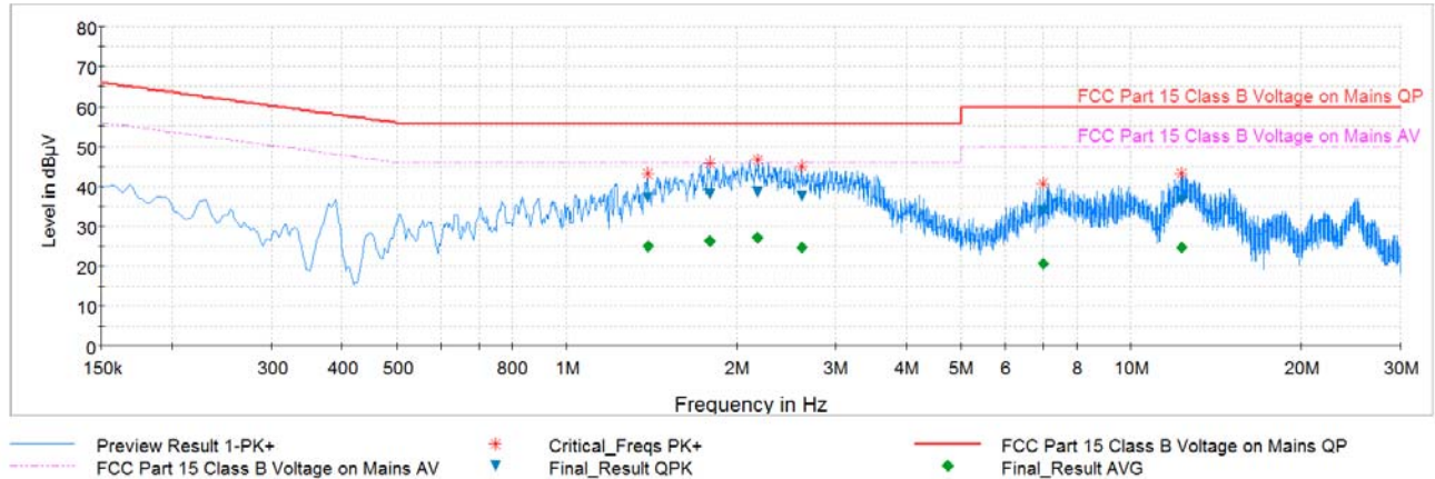
Plot 6-44. Line Conducted Plot with 802.11b (N)
