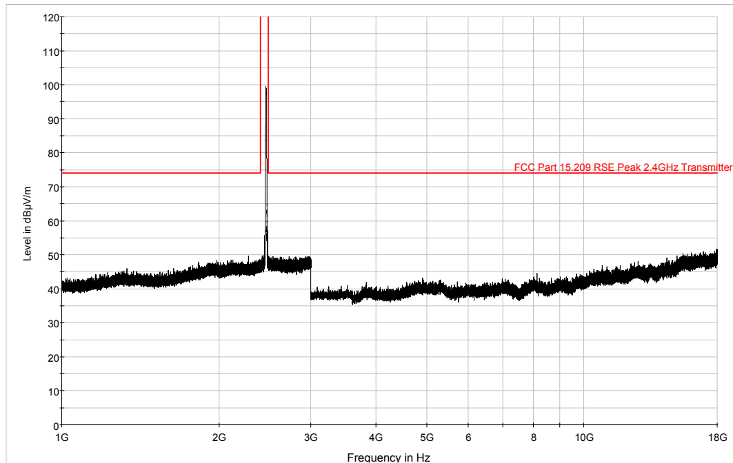
Plot 6-36. 1GHz – 18GHz Vertical Pre-Scan Plot (802.11b – Ch. 11)
