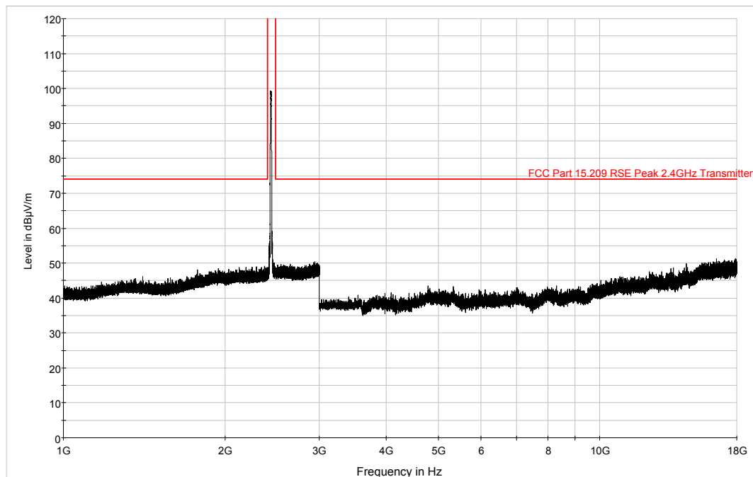
Plot 6-34. 1GHz – 18GHz Vertical Pre-Scan Plot (802.11b – Ch. 6)
