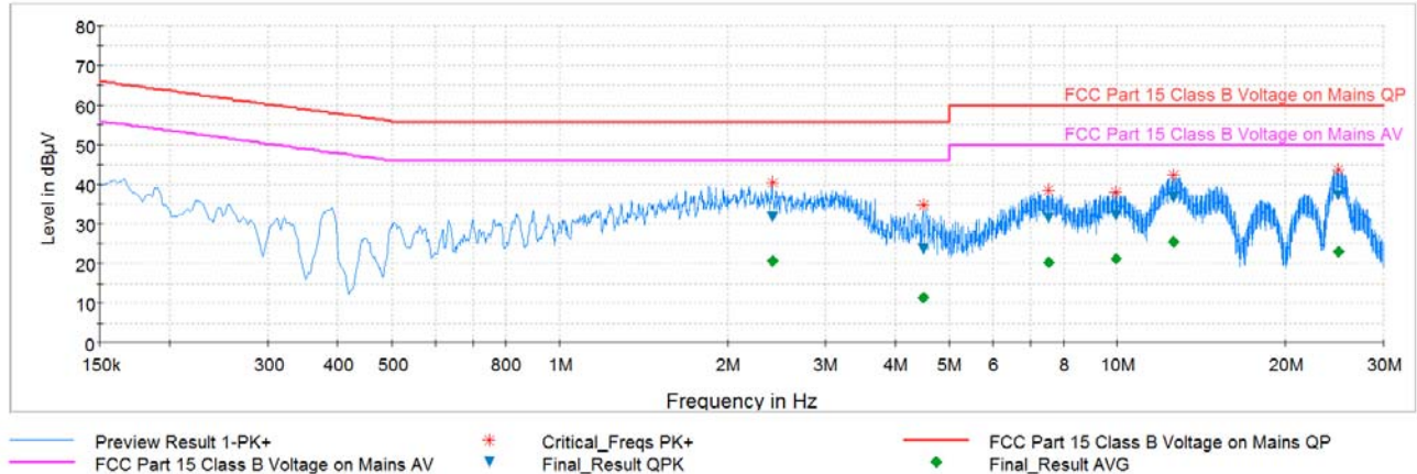
Plot 6-43. Line Conducted Plot with 802.11b (L1)
