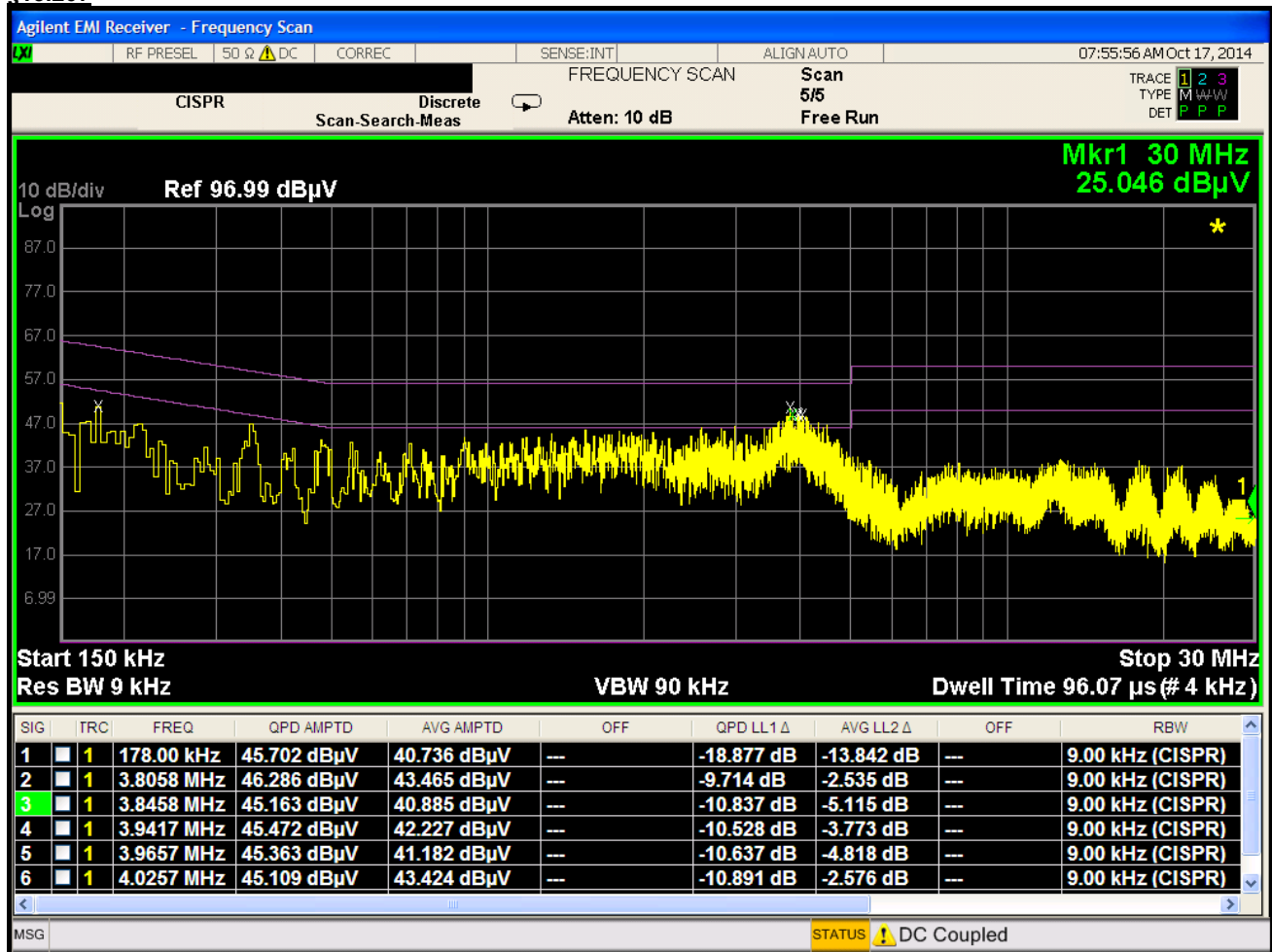
Plot 6-44. Line-Conducted Test Plot (L1)
