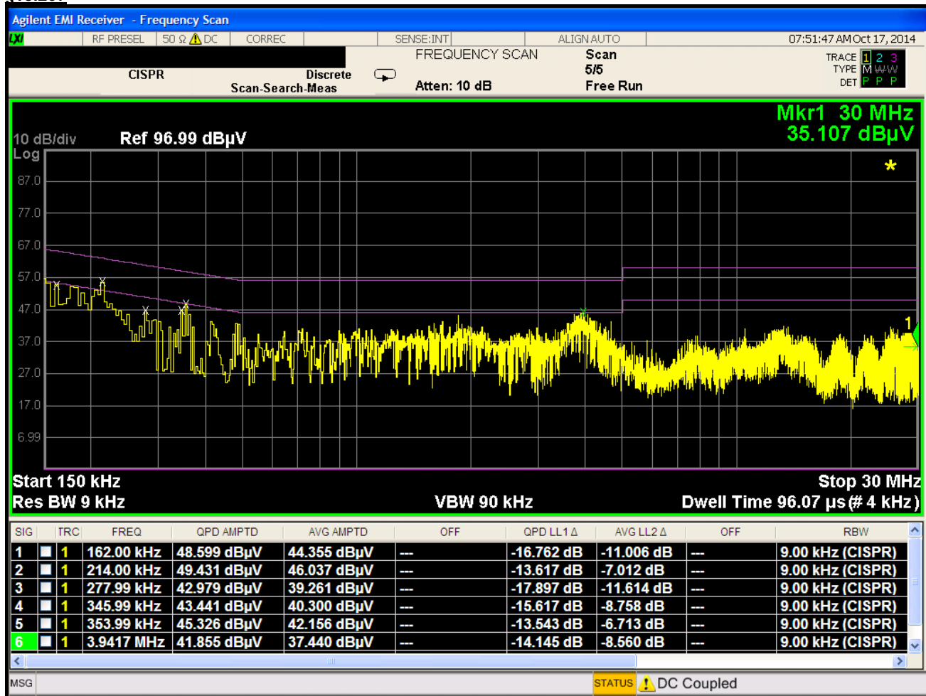
Plot 6-45. Line-Conducted Test Plot (N)
