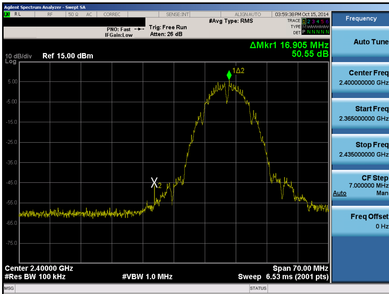
Plot 6-19. Band Edge Plot (802.11b – Ch. 1)
