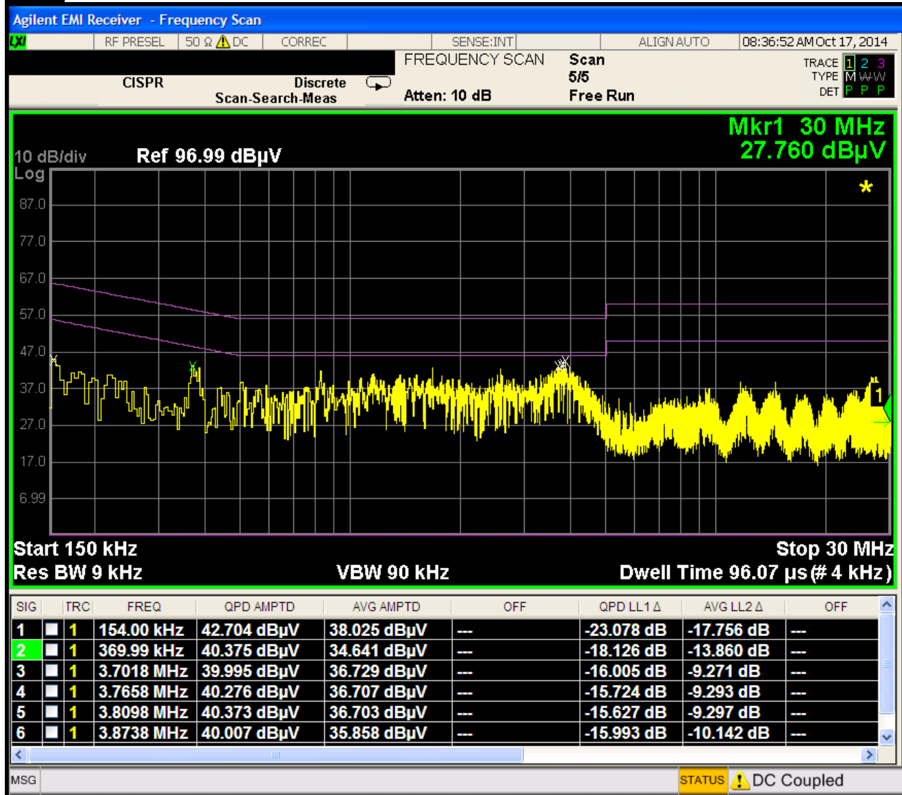
Plot 6-36. Line Conducted Plot with 802.11b (N)
