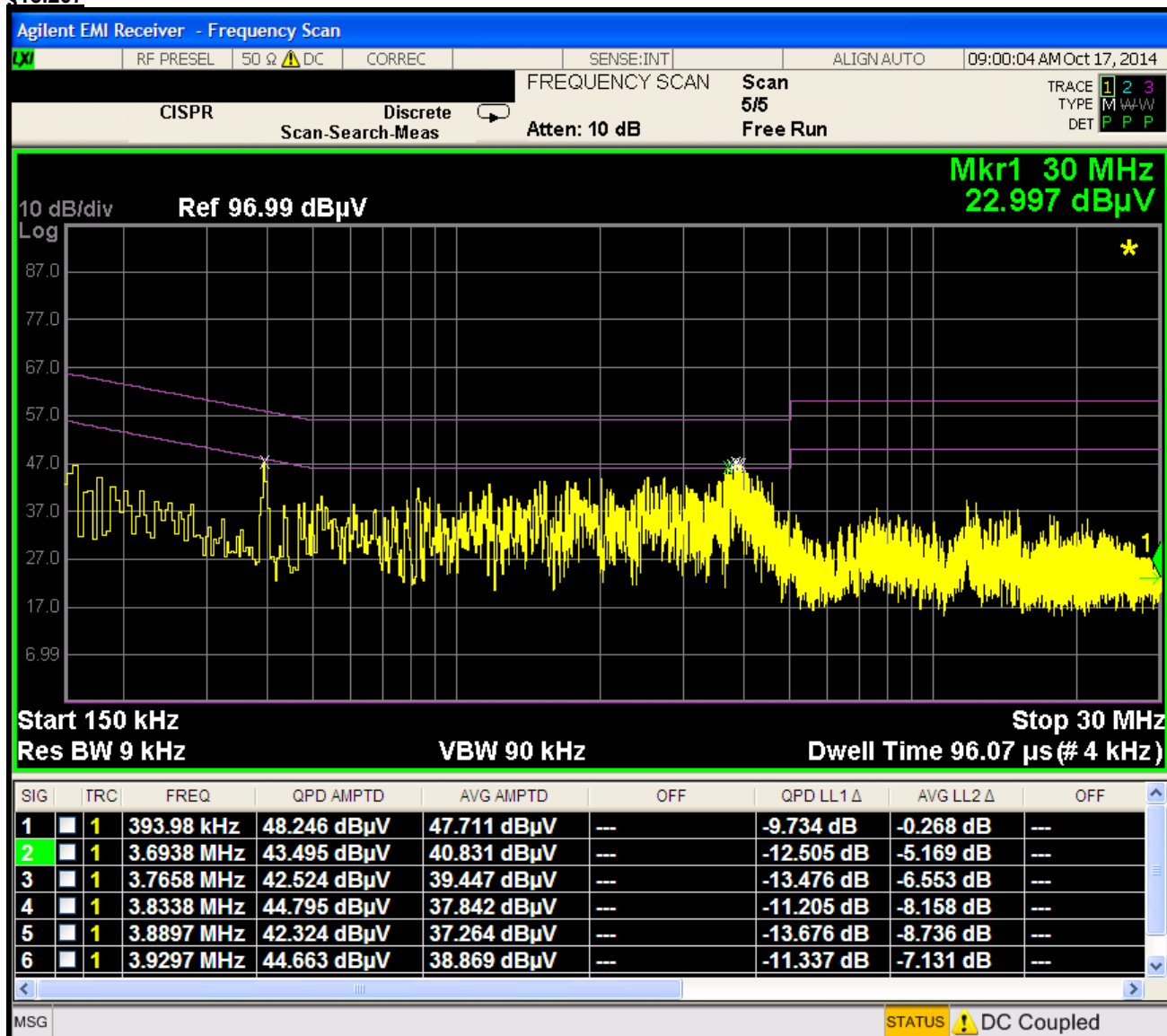
Plot 6-35. Line Conducted Plot with 802.11b (L1)
