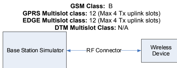
Figure 9-1 Power Measurement Setup
