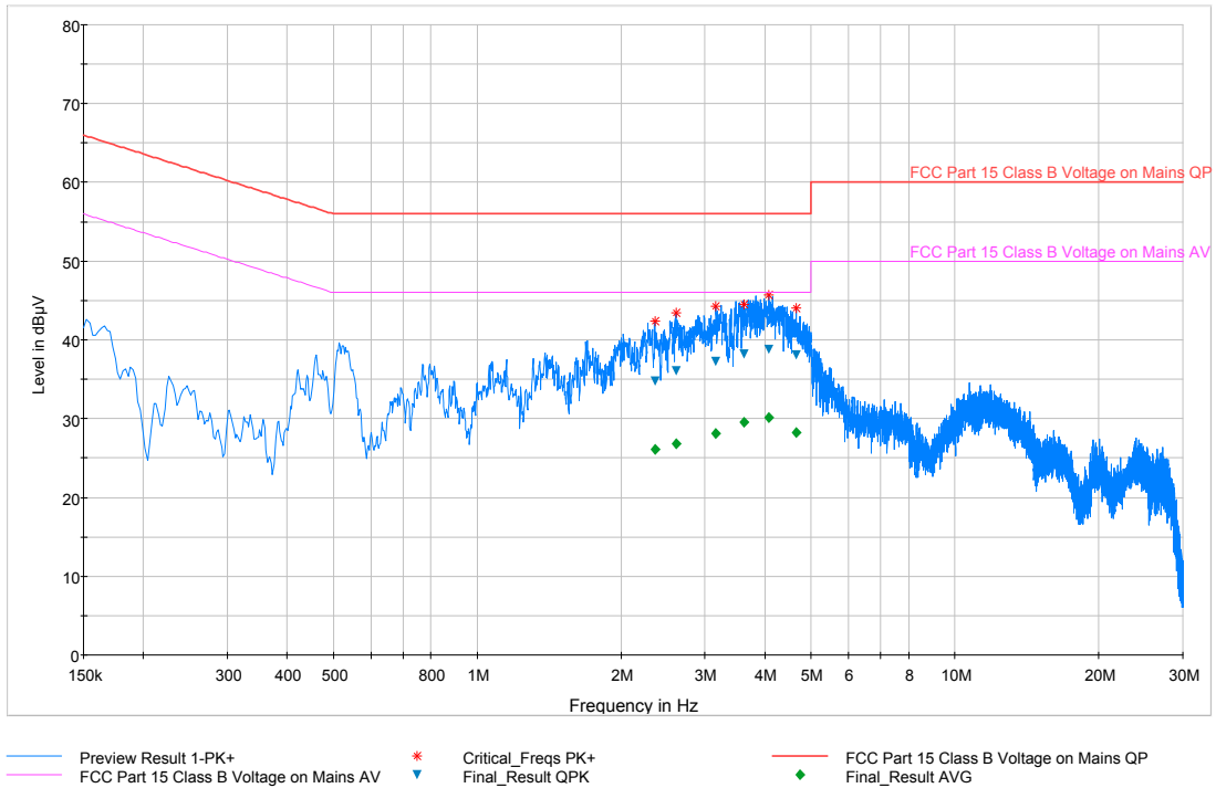
Plot 6-55. Line-Conducted Test Plot (N)
