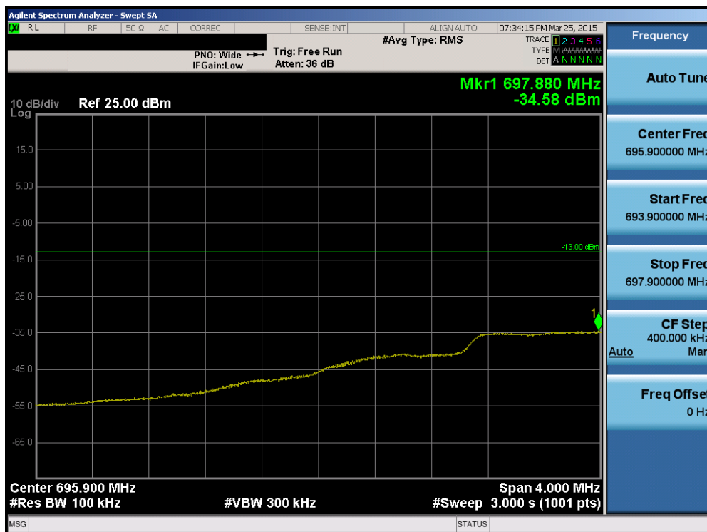
Plot 6-78. Lower Extended Band Edge Plot (Band 12 - 1.4MHz QPSK - RB Size 6)
