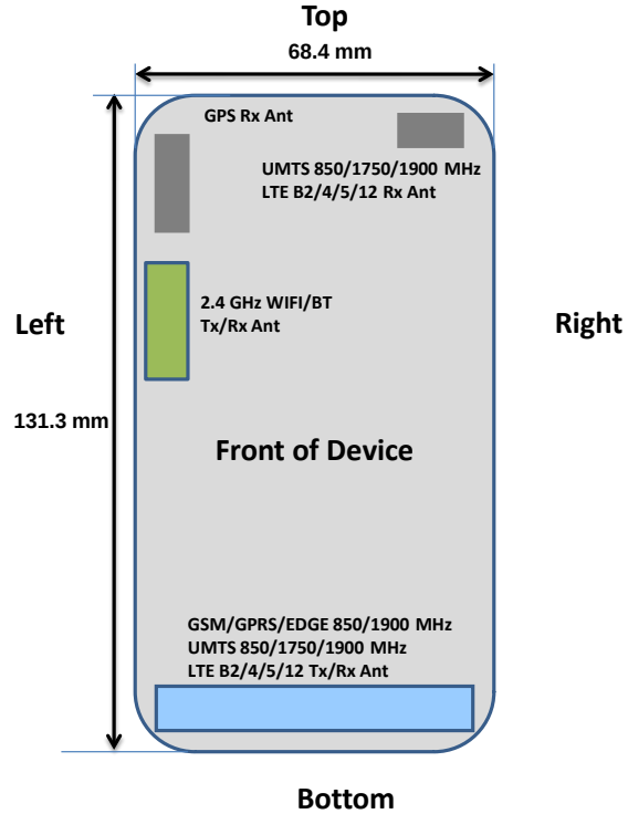
Figure F-1 DUT Antenna Locations
