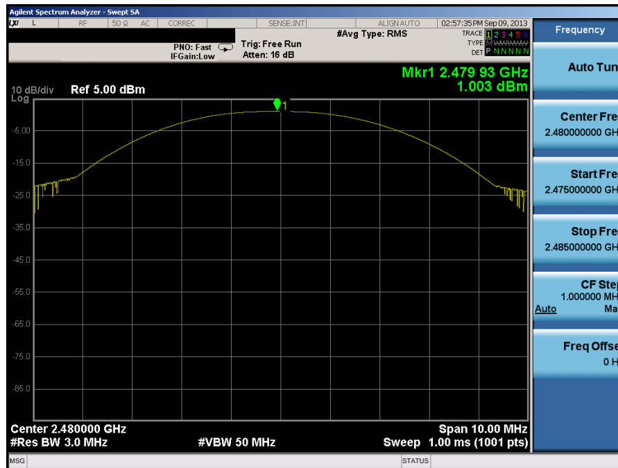
Plot 6-6. Peak Power Plot (Bluetooth (LE) – Ch. 39)
