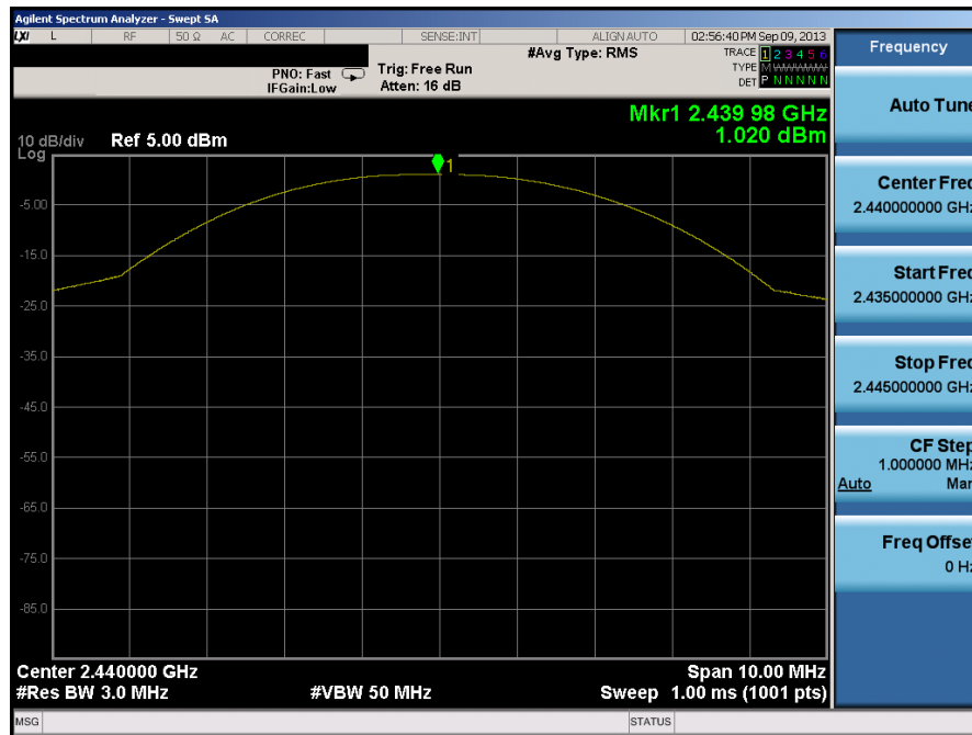
Plot 6-5. Peak Powery Plot (Bluetooth (LE) – Ch. 19)
