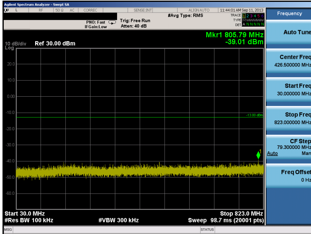
Plot 6-2. Conducted Spurious Plot (Cellular GSM Mode – Ch. 128)
