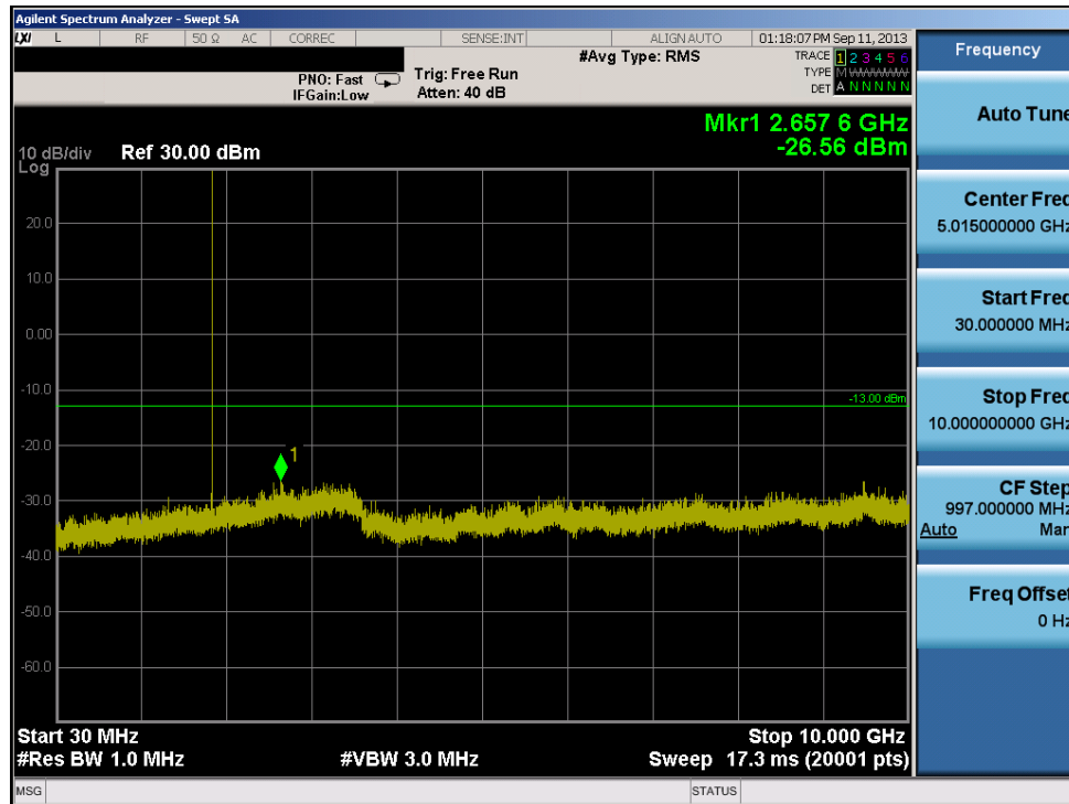
Plot 6-11. Conducted Spurious Plot (PCS GSM Mode – Ch. 512)
