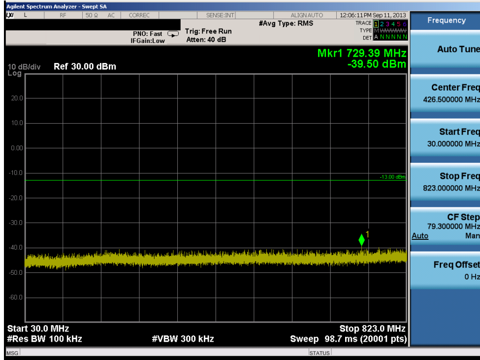
Plot 6-8. Conducted Spurious Plot (Cellular GSM Mode – Ch. 251)
