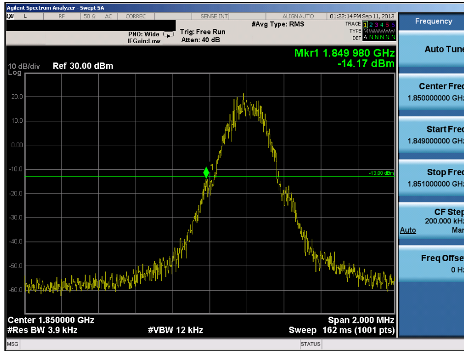
Plot 6-19. Band Edge Plot (PCS GSM Mode – Ch. 512)
