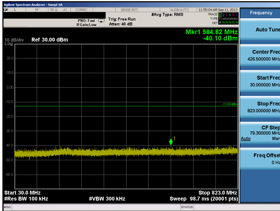
Plot 6-5. Conducted Spurious Plot (Cellular GSM Mode – Ch. 190)
