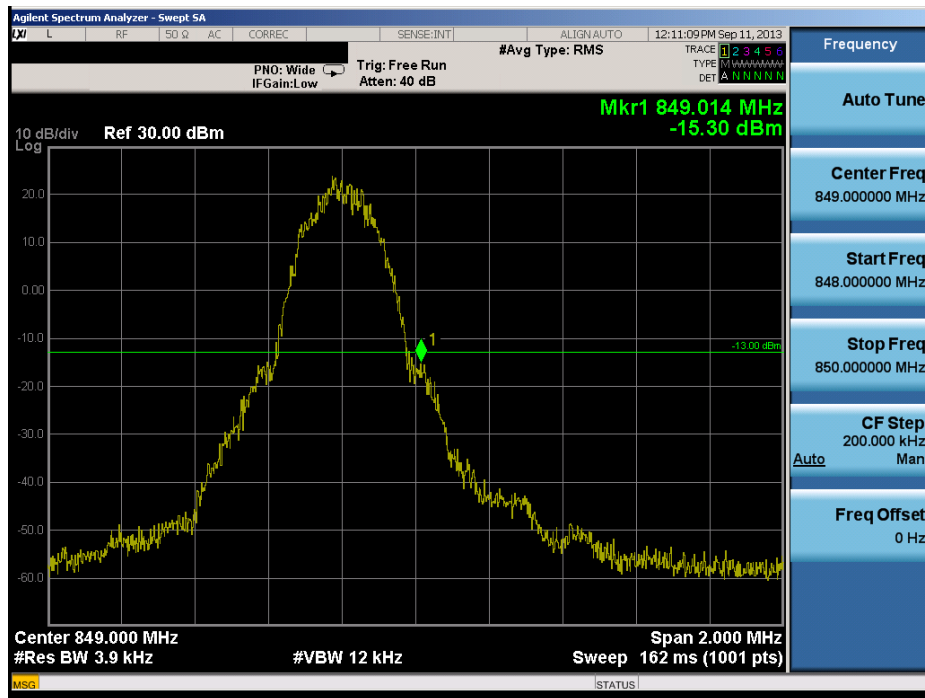
Plot 6-18. Band Edge Plot (Cellular GSM Mode – Ch. 251)
