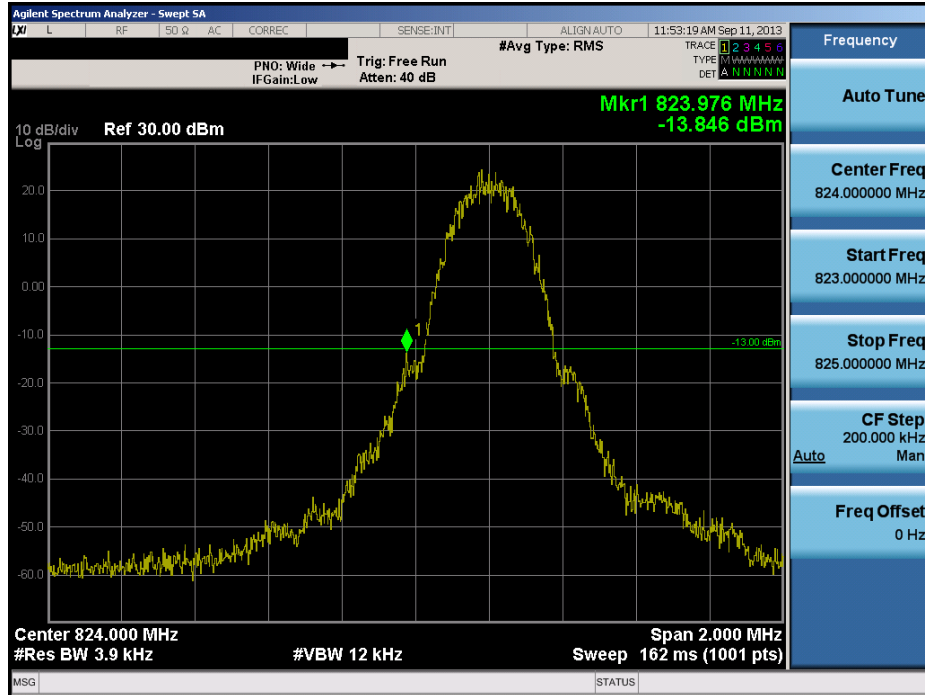
Plot 6-17. Band Edge Plot (Cellular GSM Mode – Ch. 128)
