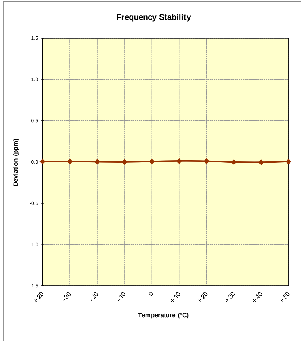
Figure 6-8. Frequency Stability Graph (PCS GSM Mode – Ch. 661)
