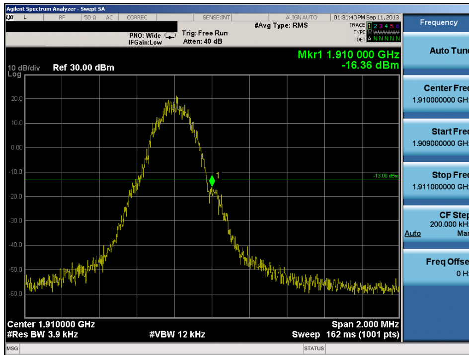
Plot 6-20. Band Edge Plot (PCS GSM Mode – Ch. 810)
