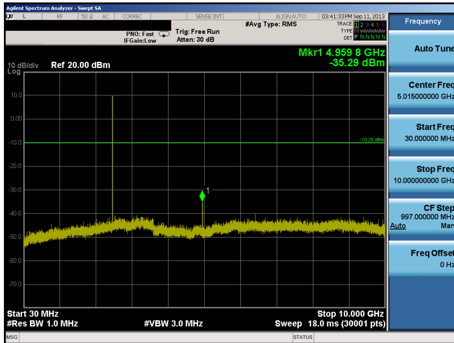
Plot 6-40. Conducted Spurious Plot (Bluetooth, 1Mbps – Ch. 78)
