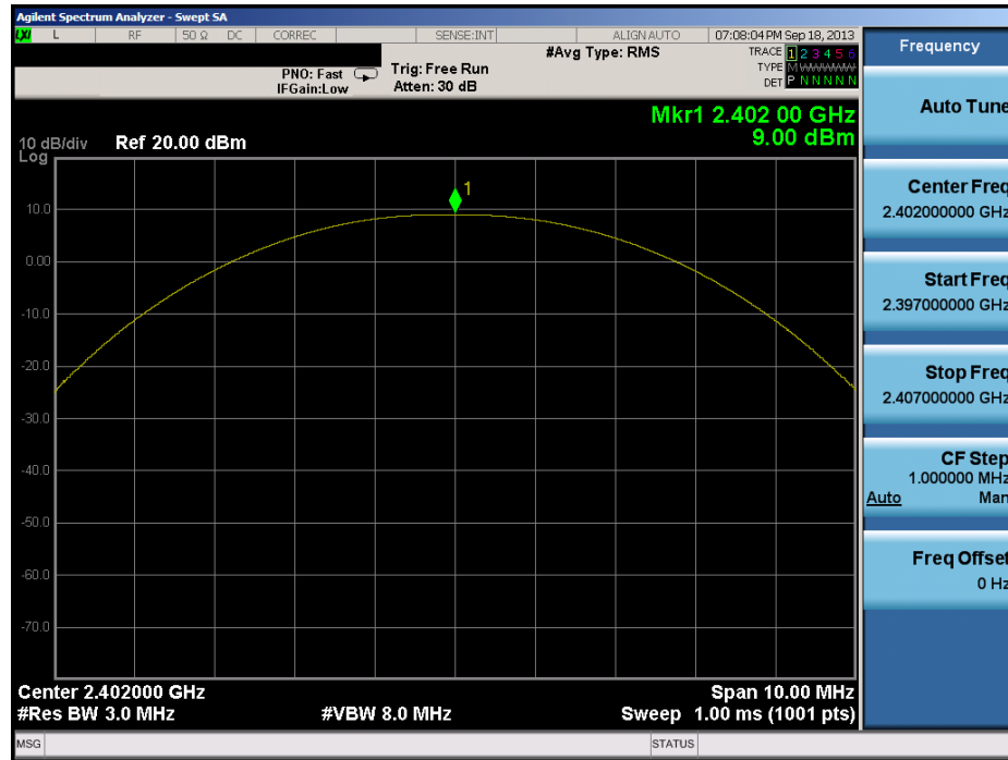
Plot 6-10. Peak Conducted Power (1Mbps - Ch. 0)
