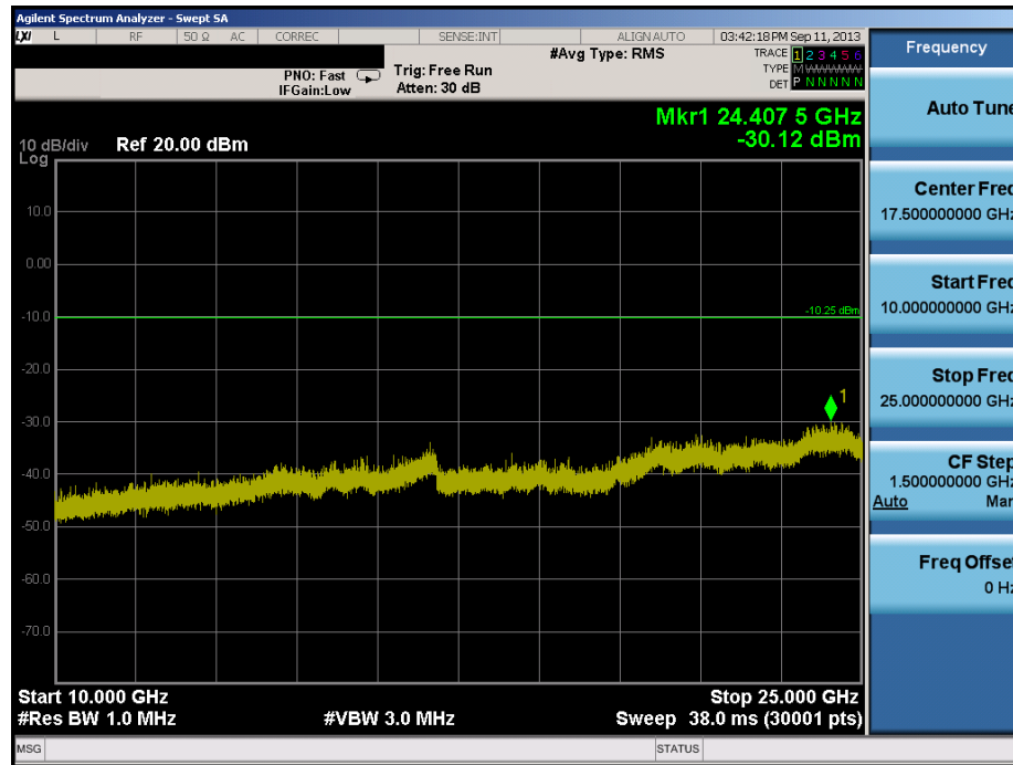
Plot 6-41. Conducted Spurious Plot (Bluetooth, 1Mbps – Ch. 78)
