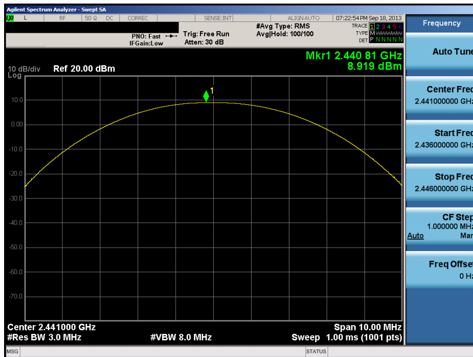
Plot 6-11. Peak Conducted Power (1Mbps - Ch. 39)
