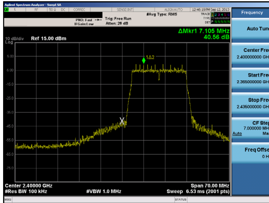
Plot 6-23. Band Edge Plot (802.11n (2.4GHz) – Ch. 1)
