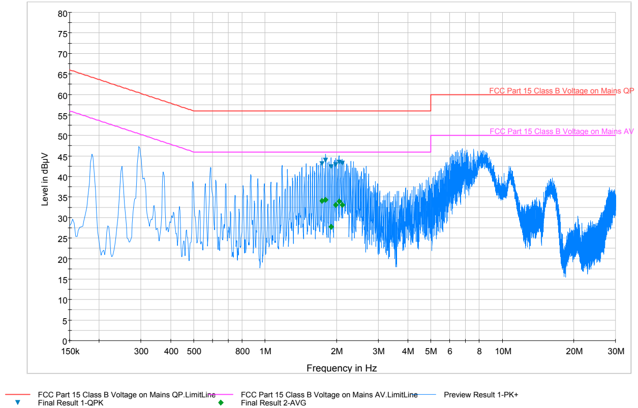
Plot 6-36. Line Conducted Plot with 802.11b (N)
