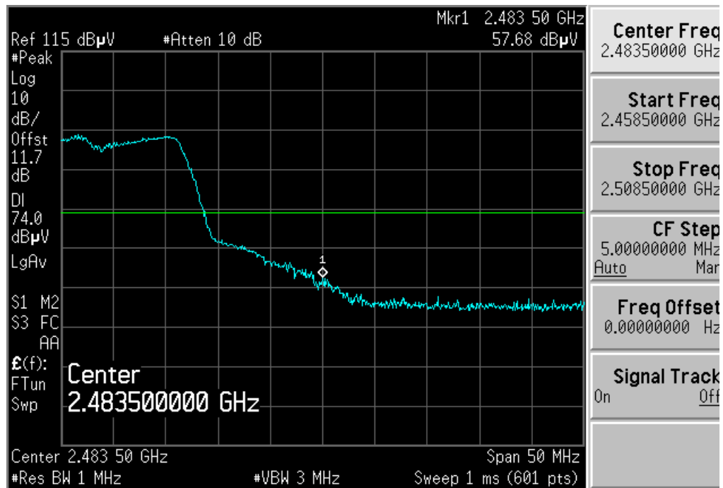
Plot 6-34. Radiated Restricted Upper Band Edge Measurement (Peak)
