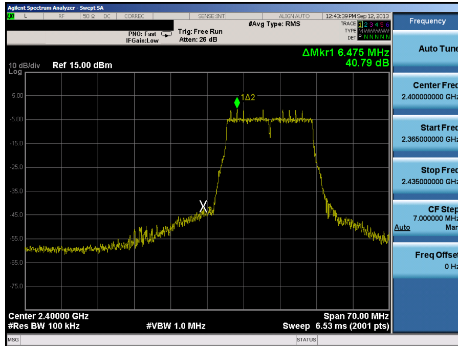
Plot 6-21. Band Edge Plot (802.11g- Ch. 1)
