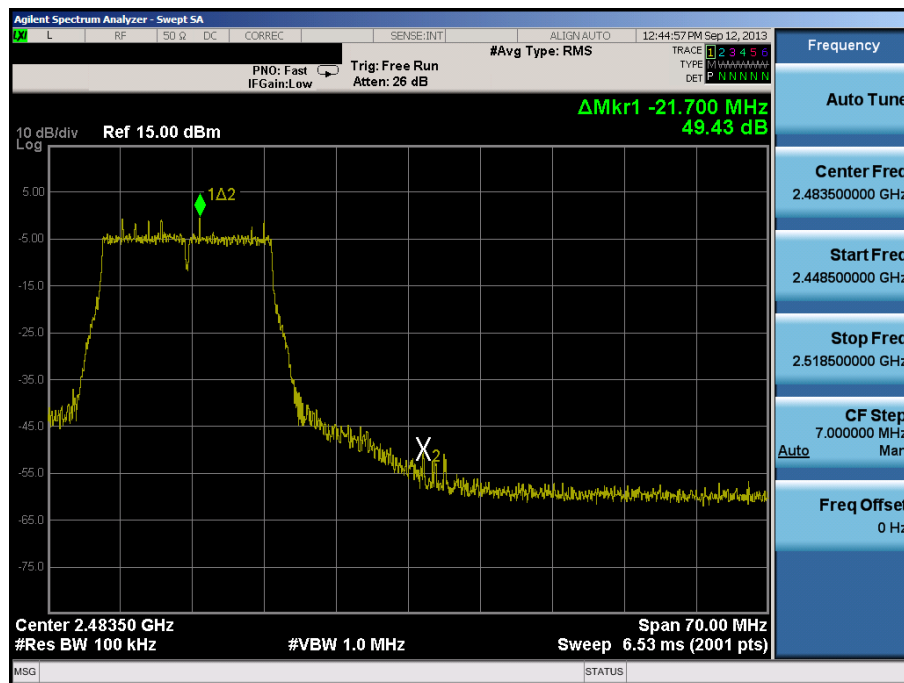
Plot 6-22. Band Edge Plot (802.11g - Ch. 11)
