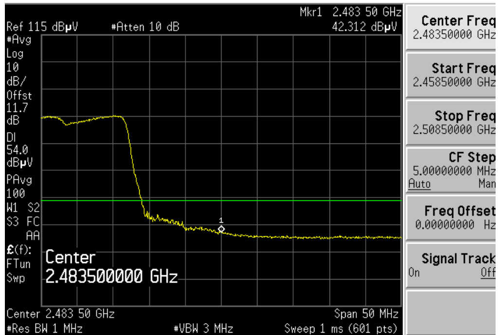
Plot 6-33. Radiated Restricted Upper Band Edge Measurement (Average)
