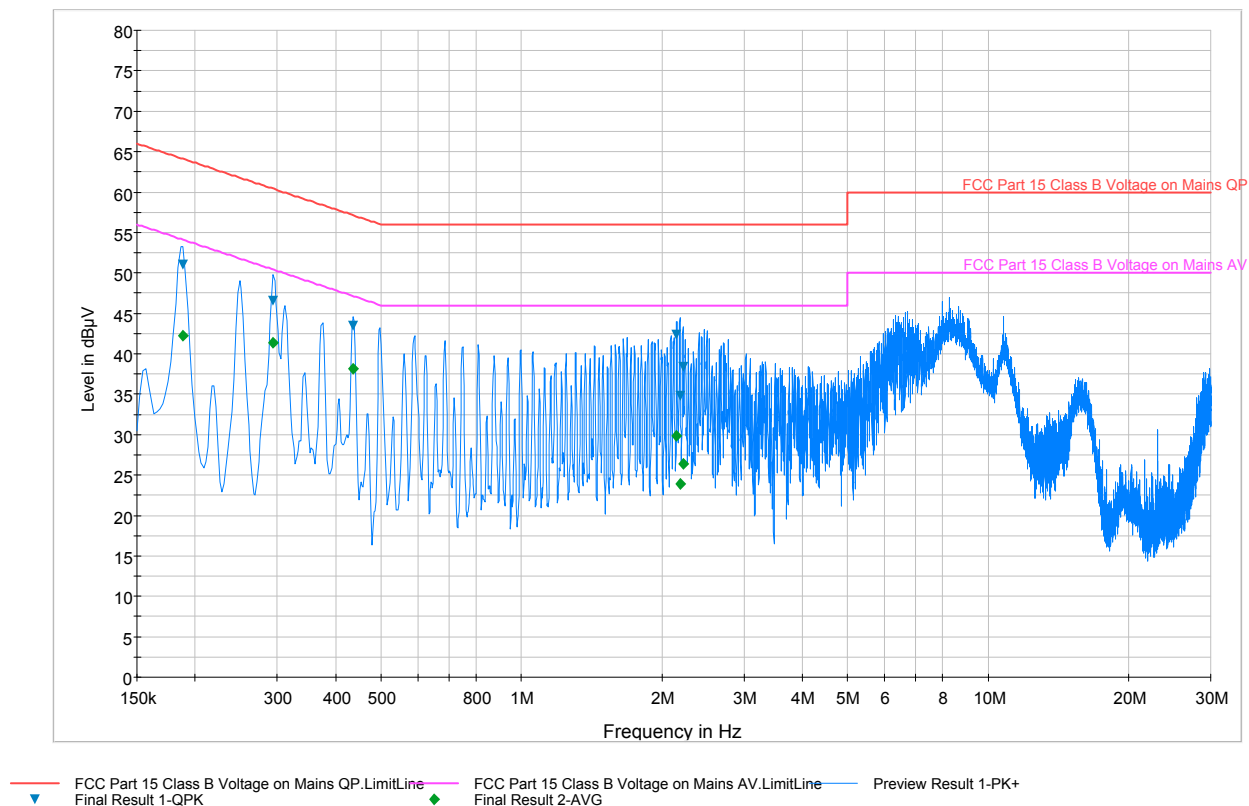
Plot 6-35. Line Conducted Plot with 802.11b (L1)
