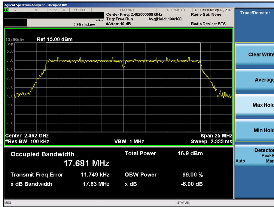
Plot 6-9. 6dB Bandwidth Plot (802.11n (2.4GHz) – Ch. 11)
