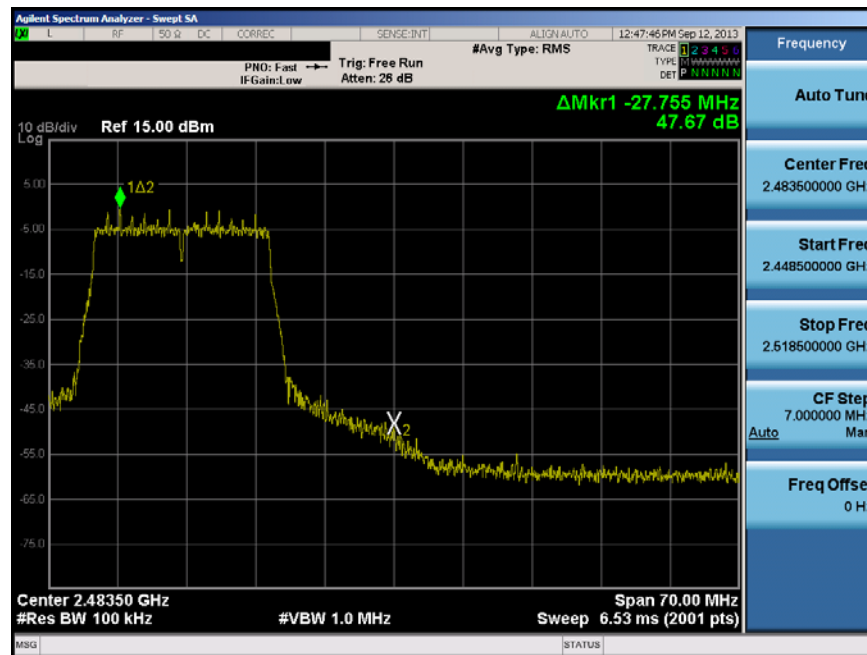
Plot 6-24. Band Edge Plot (802.11n (2.4GHz) – Ch. 11)
