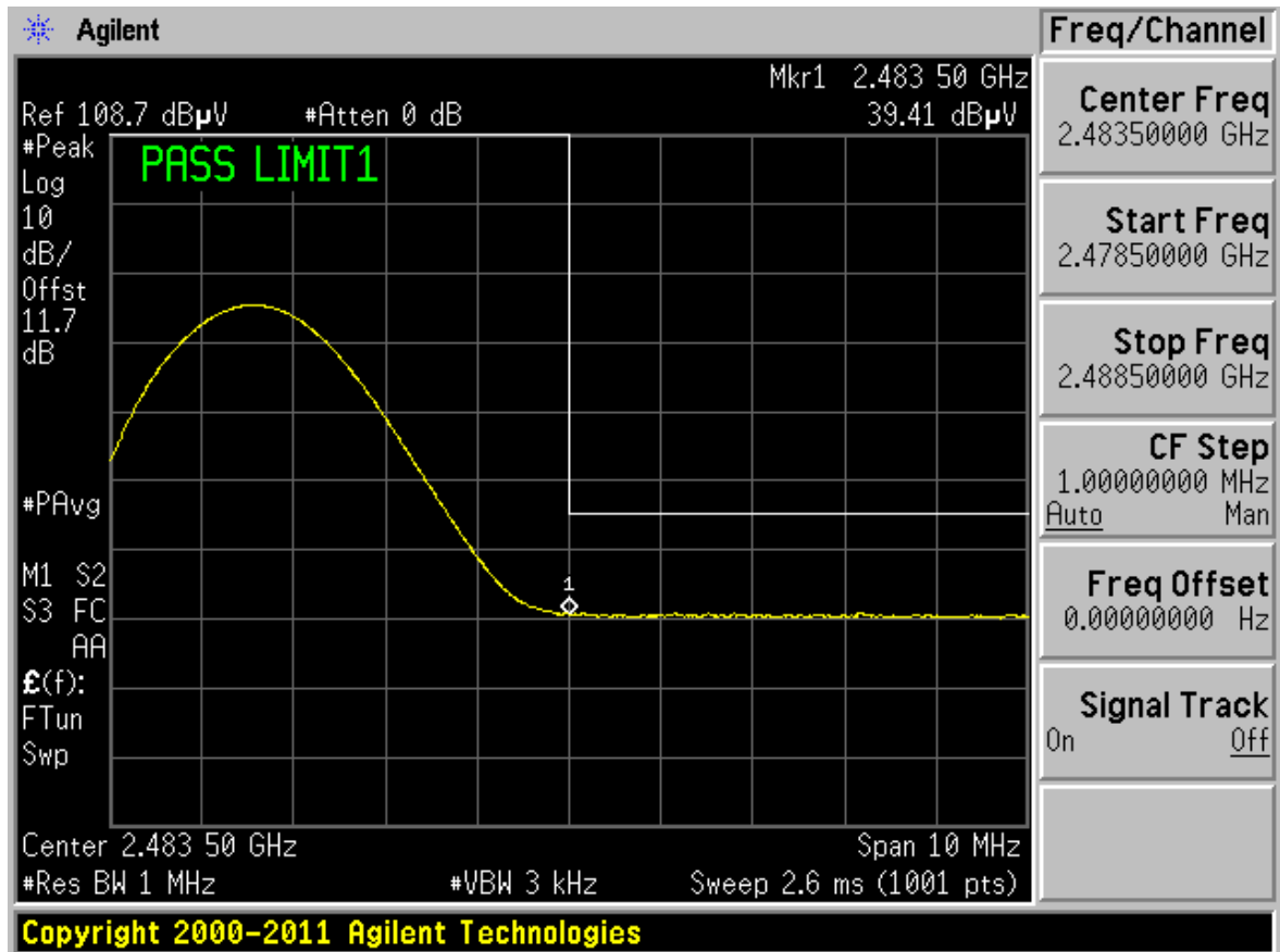
Plot 6-18. Upper Radiated Restricted Band Edge Measurement (Average)
