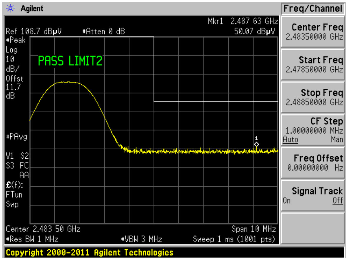
Plot 6-19. Upper Radiated Restricted Band Edge Measurement (Peak)
