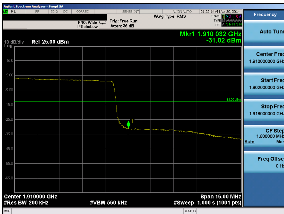
Plot 6-143. Upper Band Edge Plot (Band 2 – 20.0MHz QPSK – RB Size 100)
