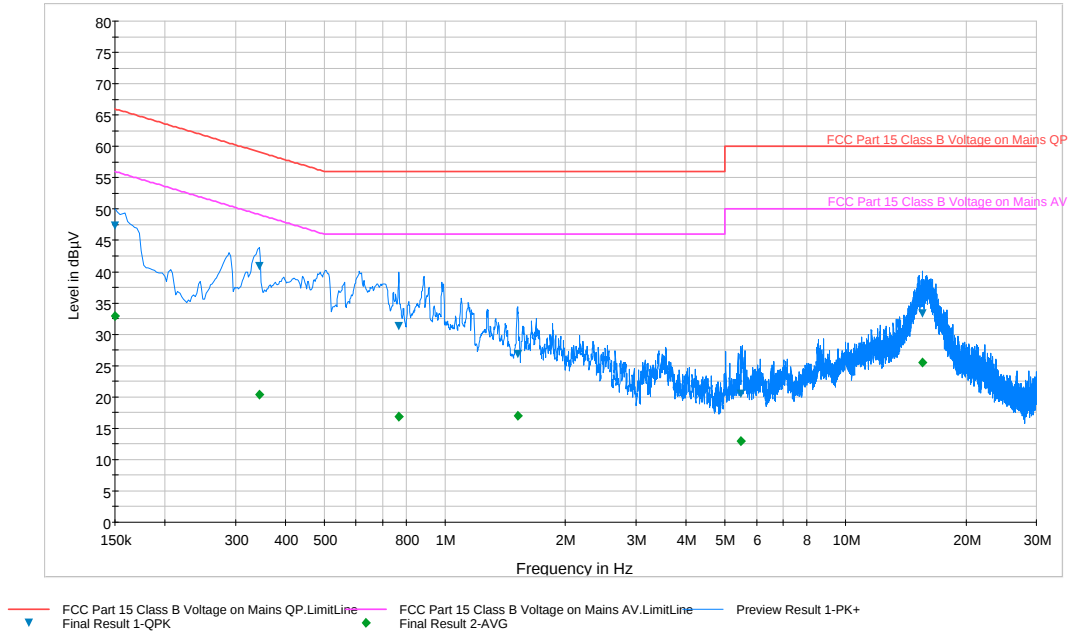
Plot 7-1. Line Conducted Plot (L1)
