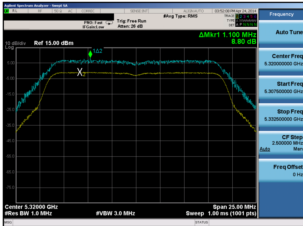
Plot 6-56. Peak Excursion Ratio Plot (20MHz BW 802.11n (UNII Band 2A) – Ch. 64)
