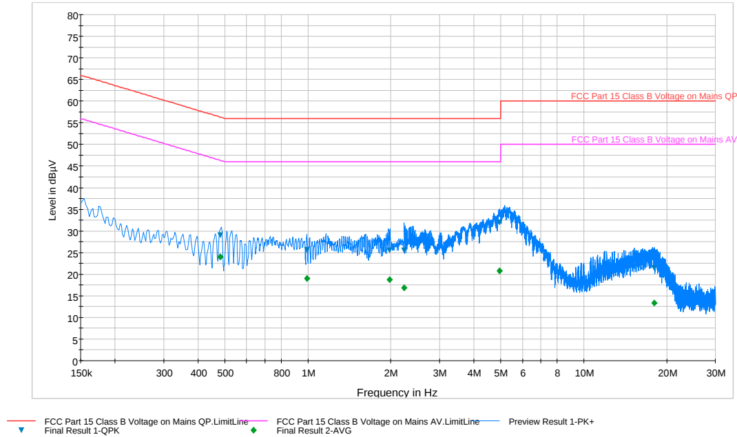
Plot 6-73. Line Conducted Plot with 802.11a UNII Band 1 (L1)
