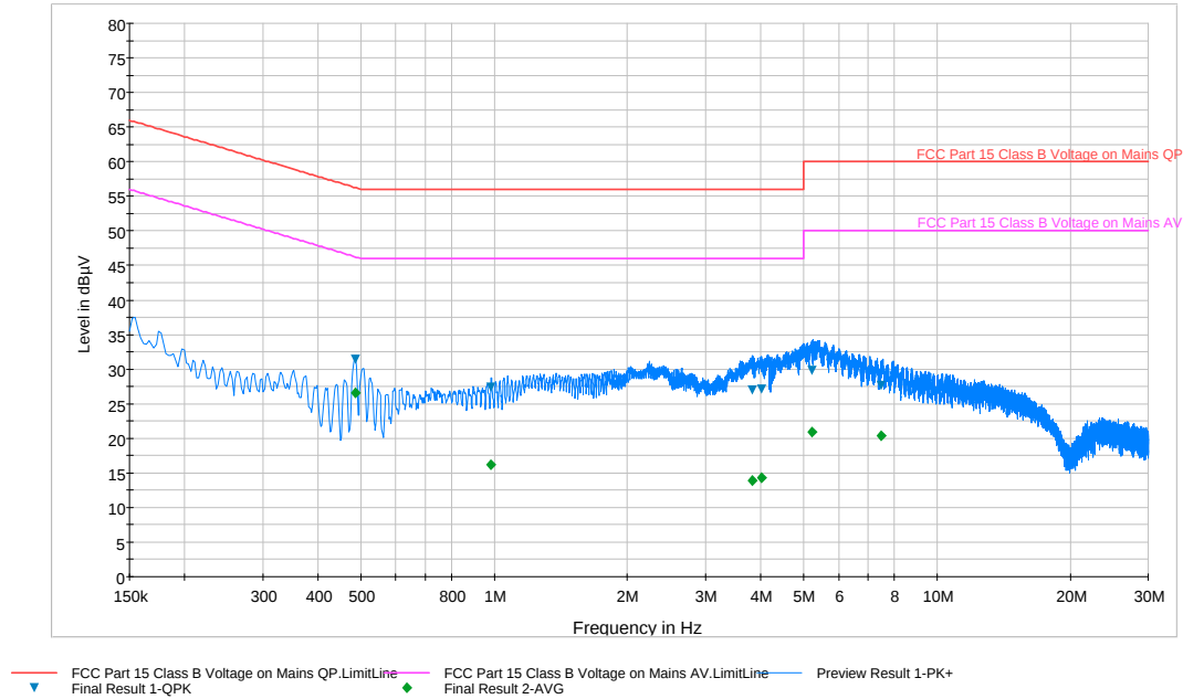
Plot 6-76. Line Conducted Plot with 802.11a UNII Band 2A (N)
