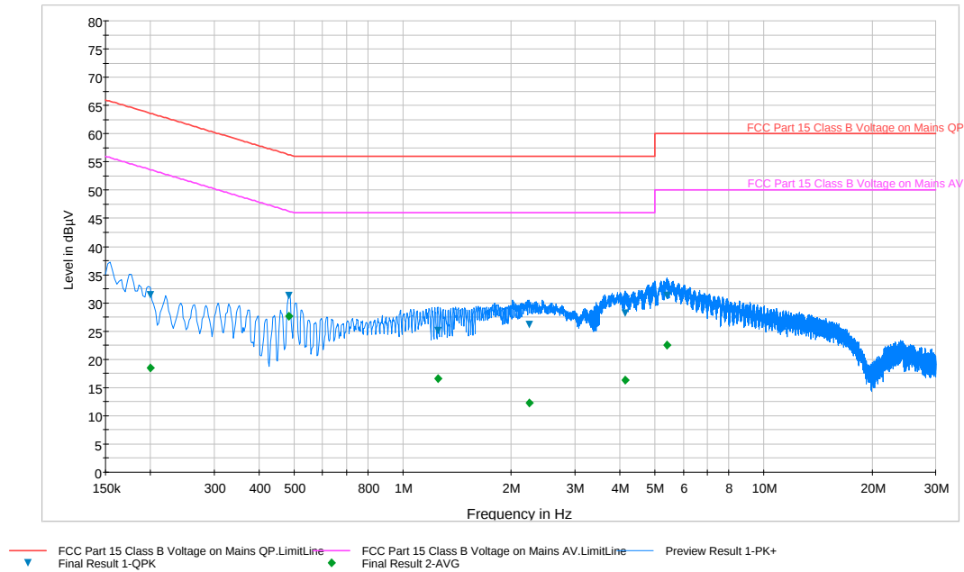
Plot 6-78. Line Conducted Plot with 802.11a UNII Band 2C (N)
