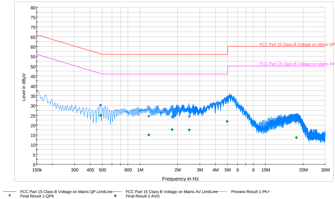
Plot 6-75. Line Conducted Plot with 802.11a UNII Band 2A (L1)
