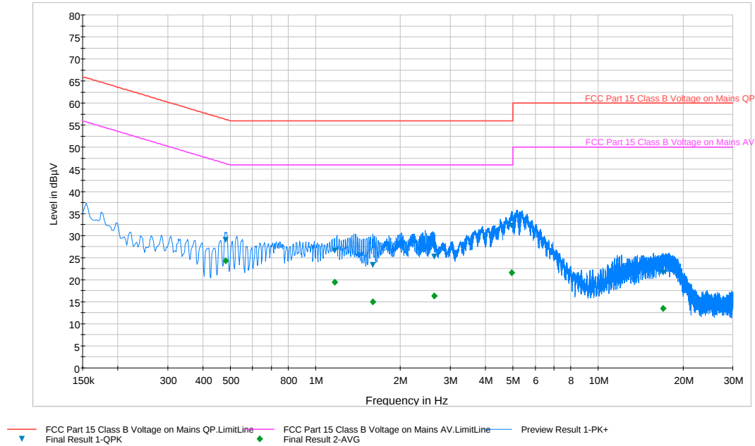
Plot 6-77. Line Conducted Plot with 802.11a UNII Band 2C (L1)
