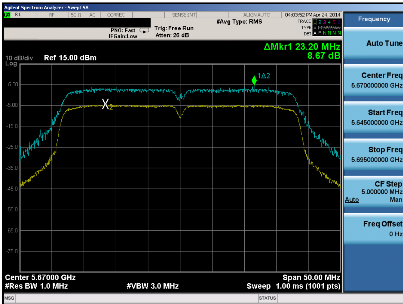
Plot 6-58. Peak Excursion Ratio Plot (40MHz BW 802.11n (UNII Band 2C) - Ch. 134)
