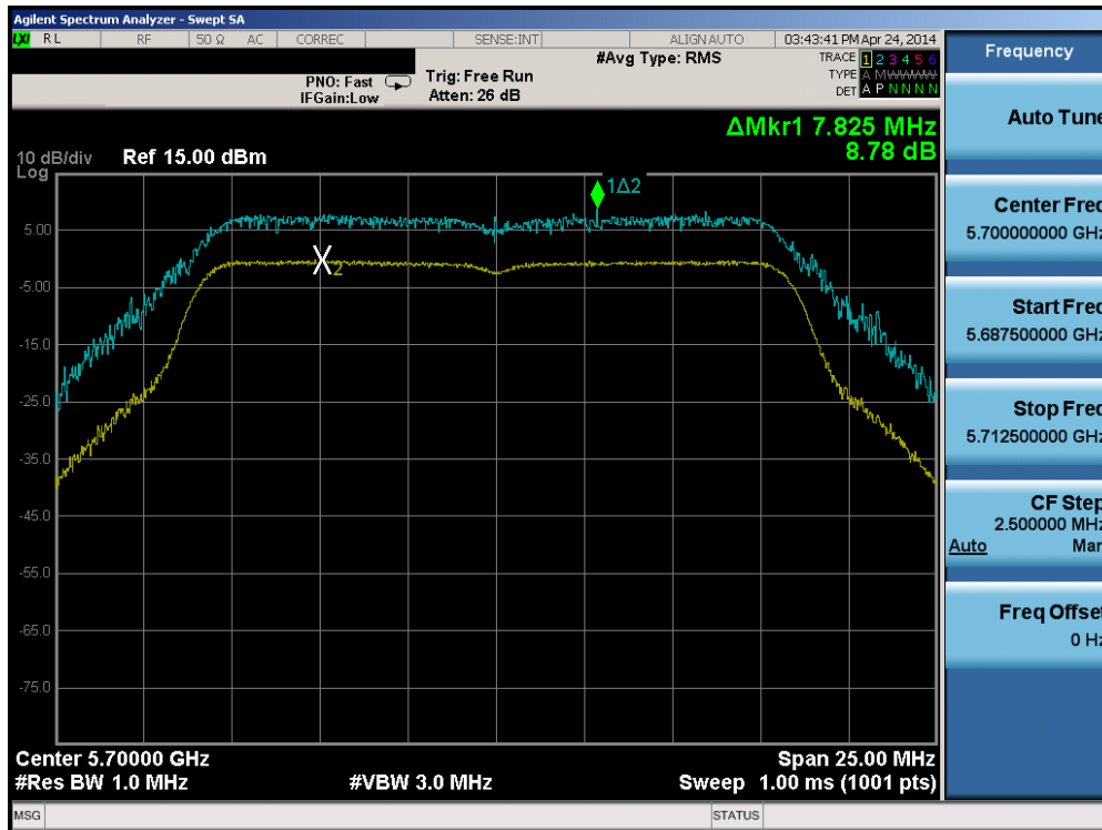
Plot 6-57. Peak Excursion Ratio Plot (802.11a (UNII Band 2C) – Ch. 140)
