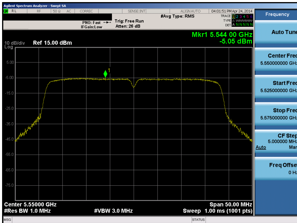
Plot 6-54. Peak Power Spectral Density Plot (40MHz BW 802.11a/n (UNII Band 2C) – Ch. 110)
