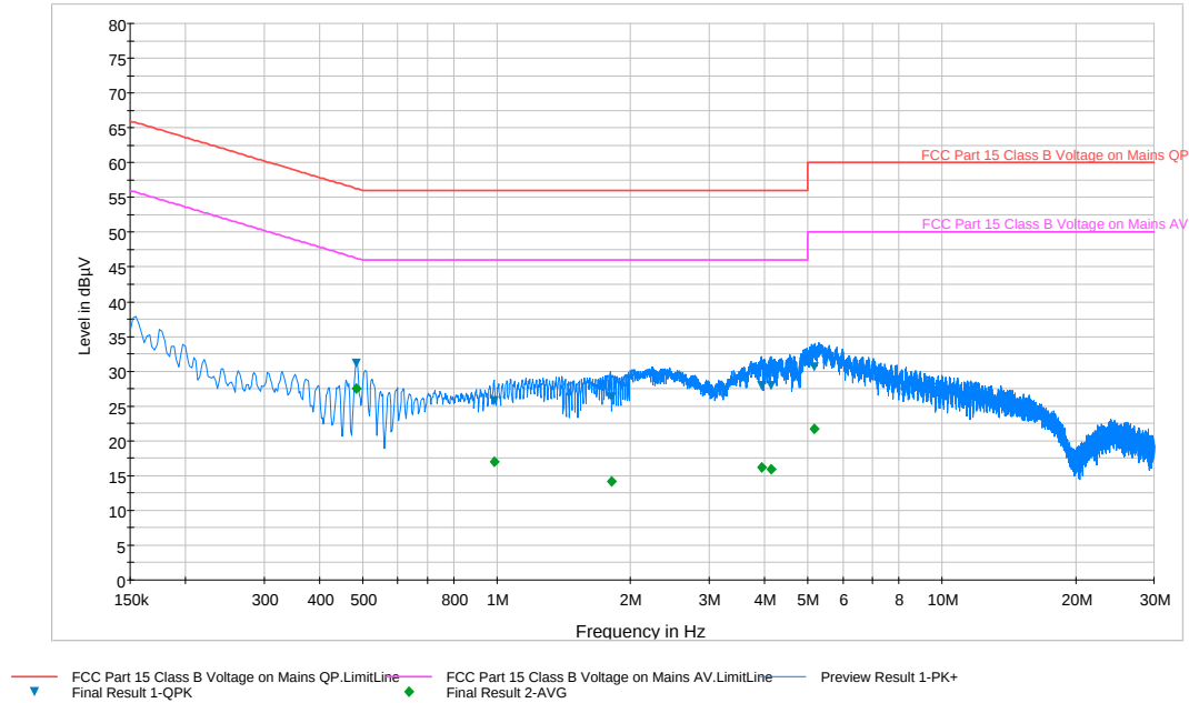
Plot 6-74. Line Conducted Plot with 802.11a UNII Band 1 (N)
