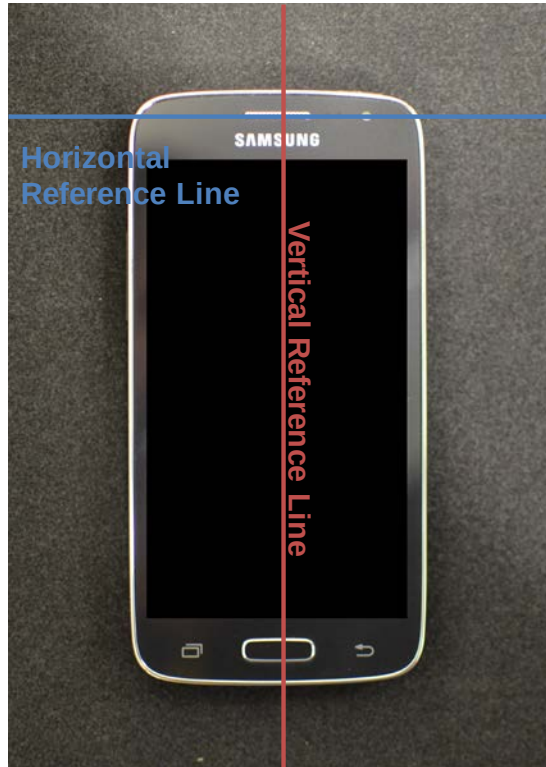
SAR Test Setup Photo 9 – Vertical and Horizontal Reference Lines
