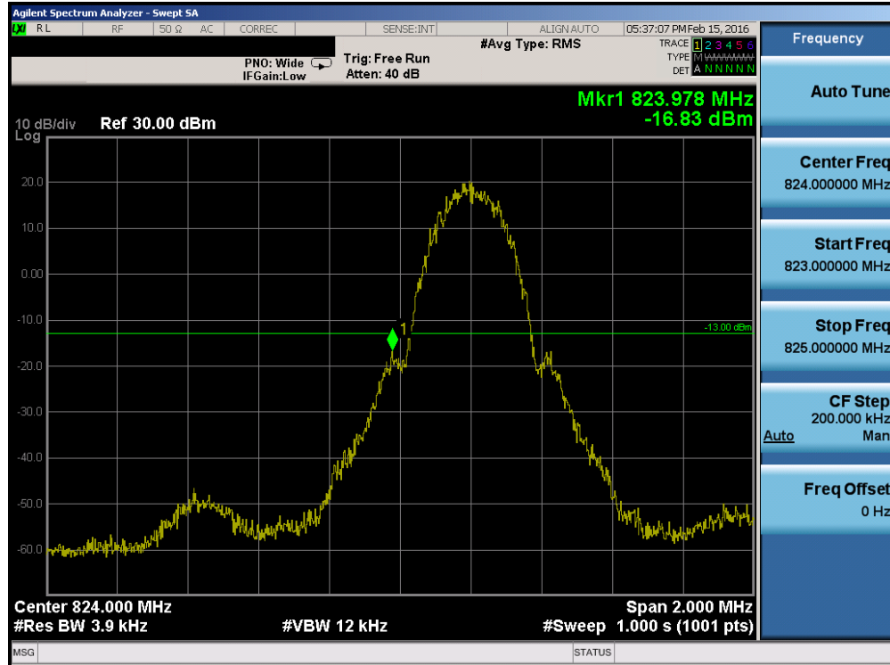
Plot 7-41. Band Edge Plot (Cellular GPRS Mode – Ch. 128)
