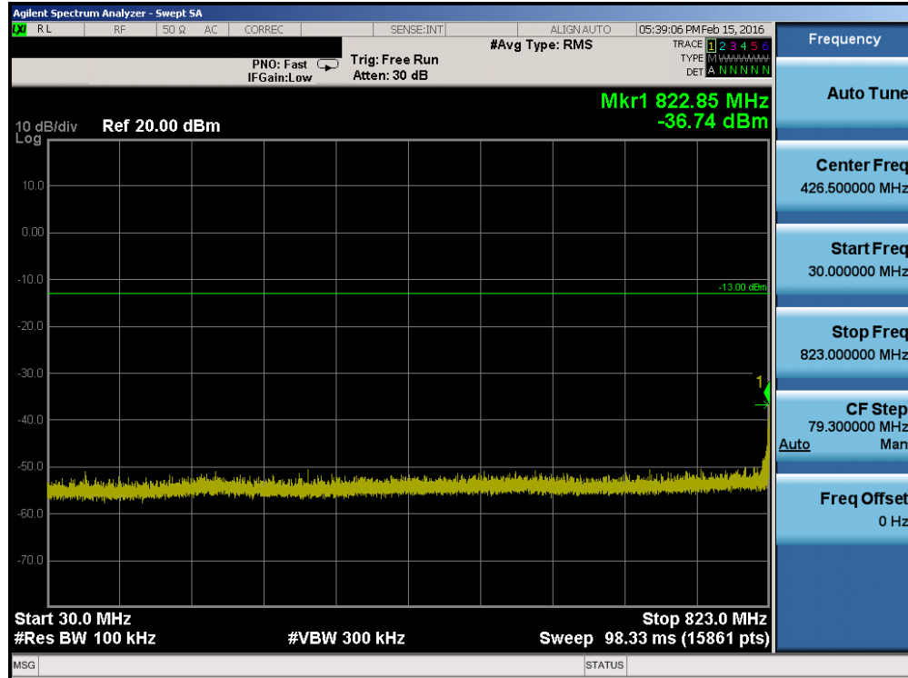
Plot 7-5. Conducted Spurious Plot (Cellular GPRS Mode – Ch. 128)
