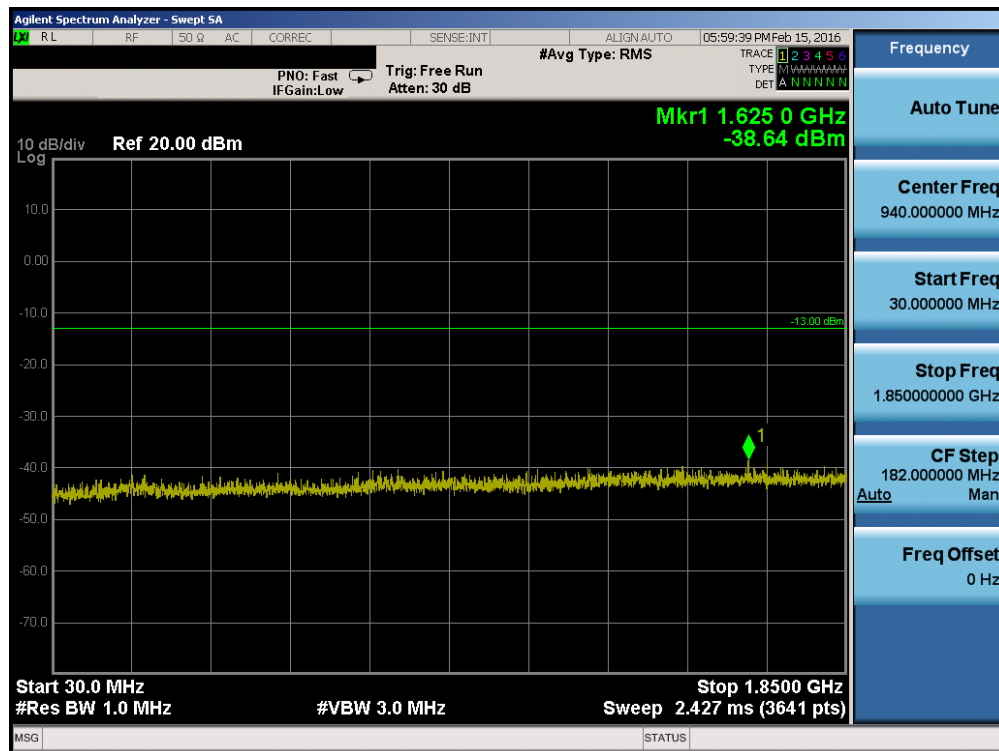
Plot 7-20. Conducted Spurious Plot (PCS GPRS Mode – Ch. 810)
