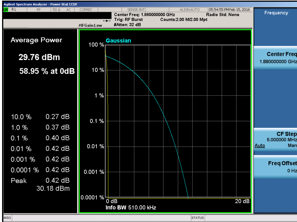
Plot 7-53. Peak-Average Ratio Plot (PCS GPRS Mode – Ch. 661)
