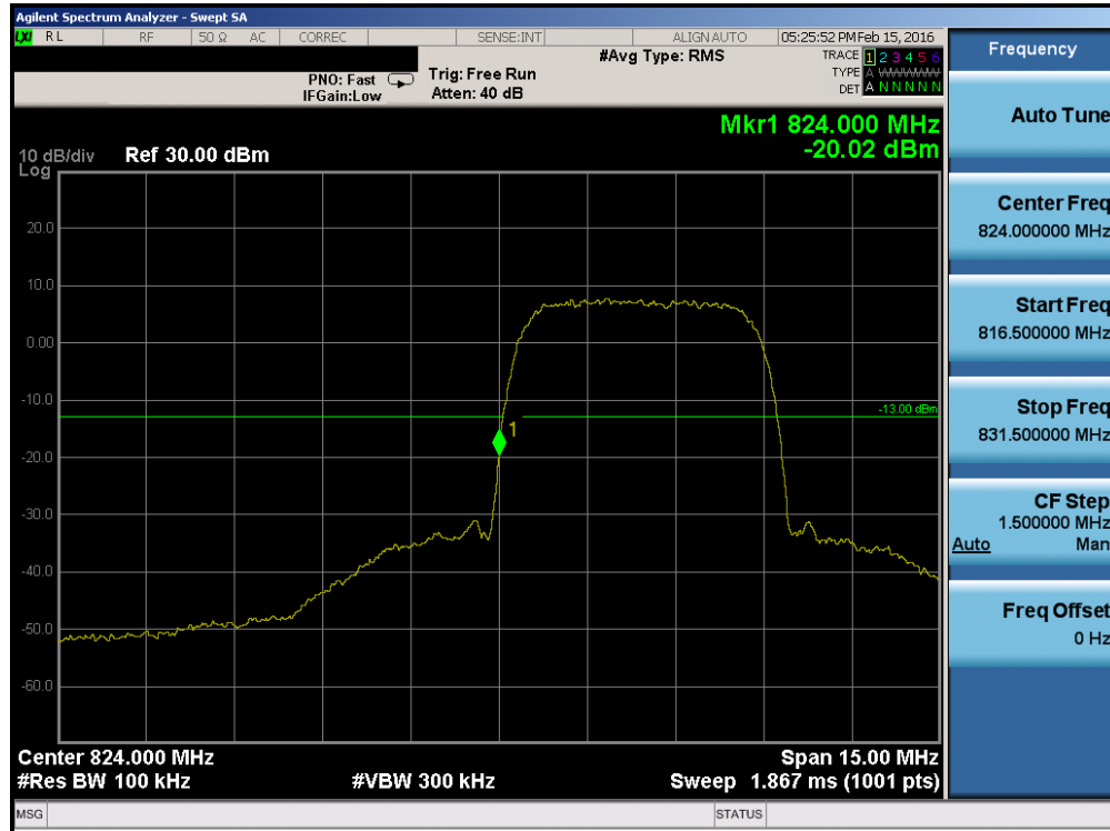
Plot 7-47. Band Edge Plot (Cellular WCDMA Mode – Ch. 4132)
