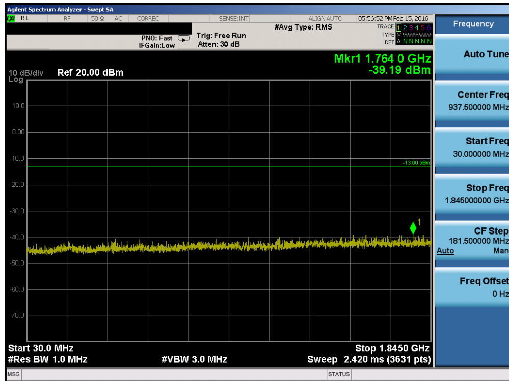
Plot 7-14. Conducted Spurious Plot (PCS GPRS Mode – Ch. 512)
