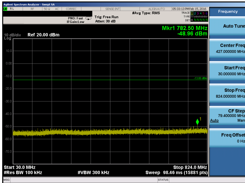
Plot 7-8. Conducted Spurious Plot (Cellular GPRS Mode – Ch. 190)
