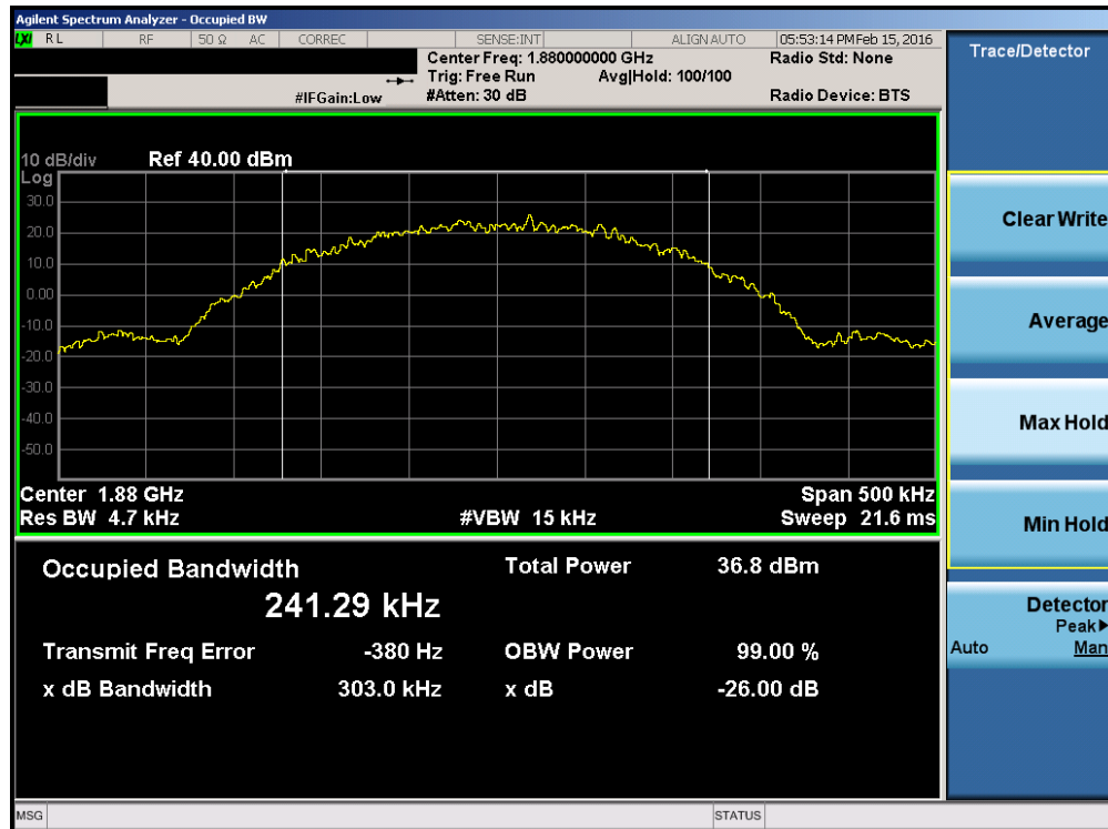
Plot 7-2. Occupied Bandwidth Plot (PCS GPRS Mode – Ch. 661)
