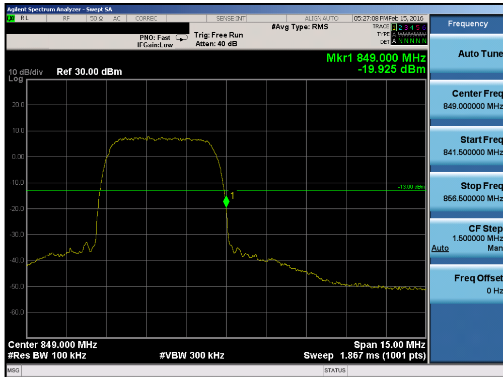
Plot 7-48. Band Edge Plot (Cellular WCDMA Mode – Ch. 4233)
