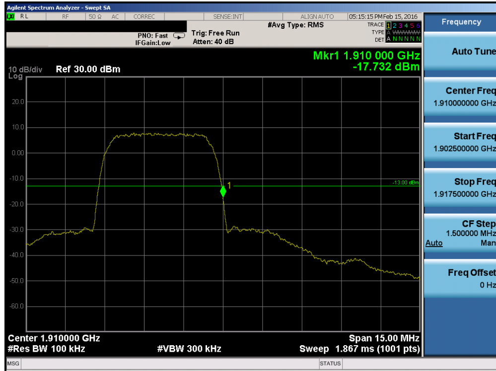
Plot 7-51. Band Edge Plot (PCS WCDMA Mode – Ch. 9538)
