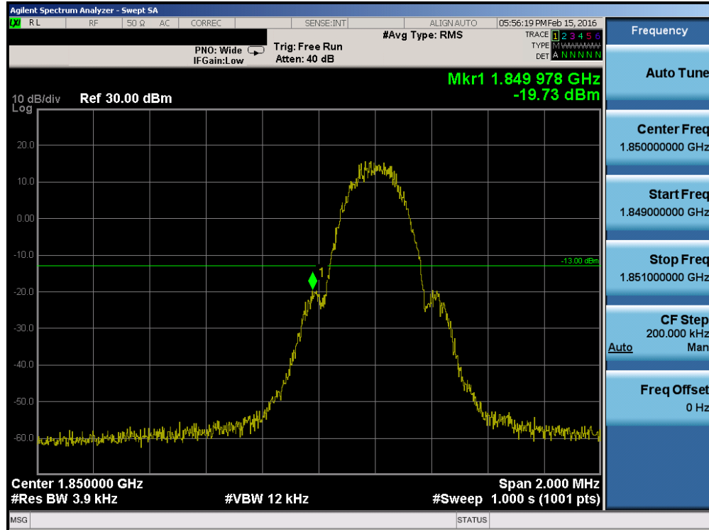
Plot 7-43. Band Edge Plot (PCS GPRS Mode – Ch. 512)
