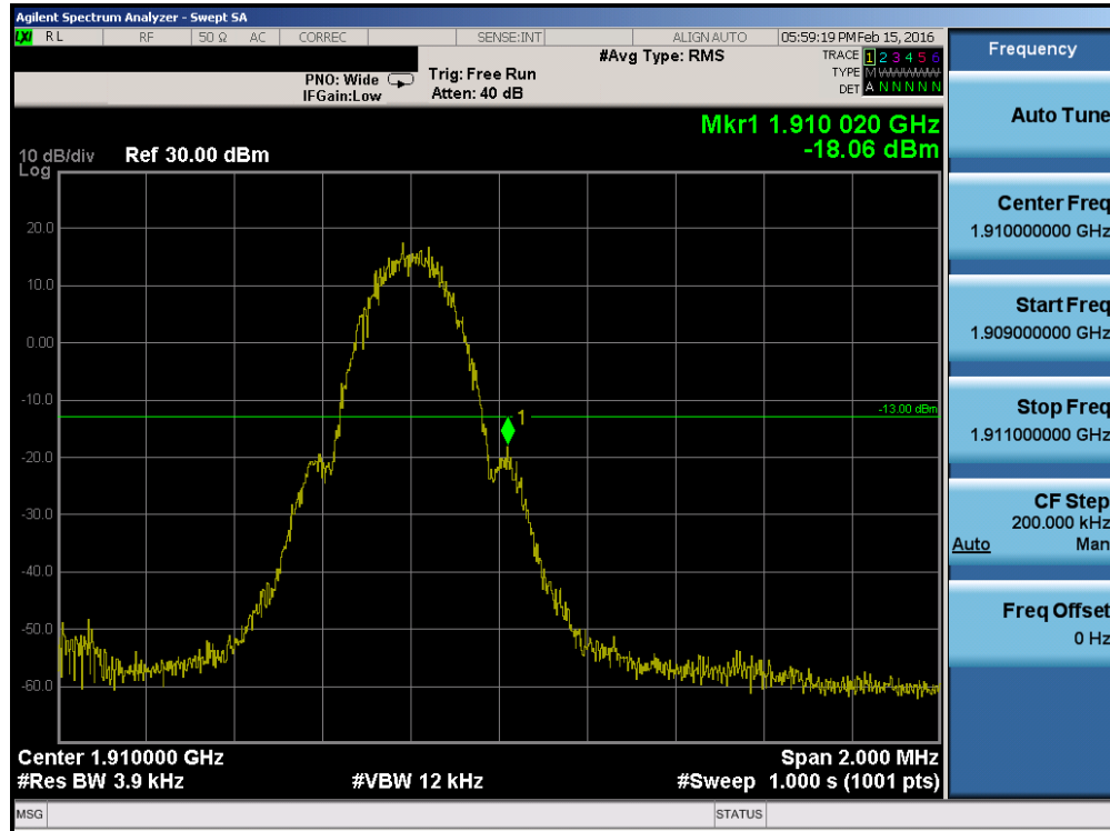
Plot 7-45. Band Edge Plot (PCS GPRS Mode – Ch. 810)
