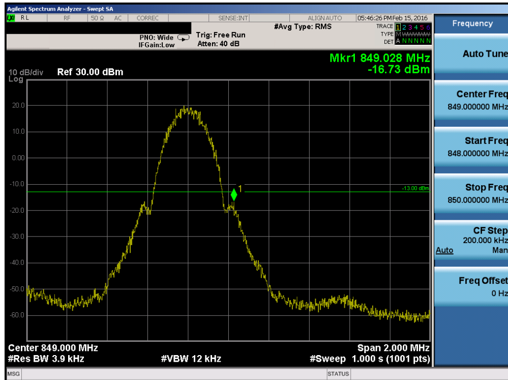
Plot 7-42. Band Edge Plot (Cellular GPRS Mode – Ch. 251)
