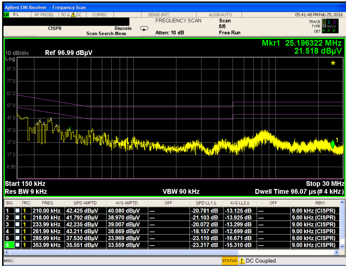
Plot 8-3. Line-Conducted Test Plot (N)
