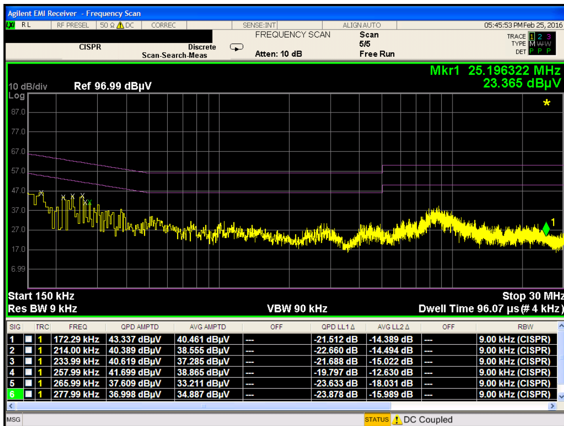
Plot 8-4. Line-Conducted Test Plot (L1)
