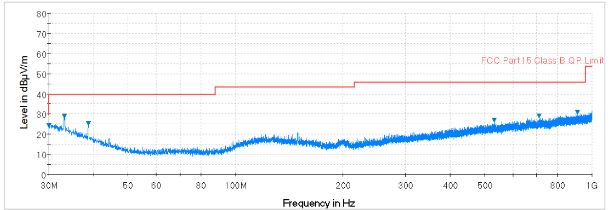
Plot 7-91. Radiated Spurious Plot below 1GHz (802.11a – U3 Ch. 157, Ant. Pol. H)
