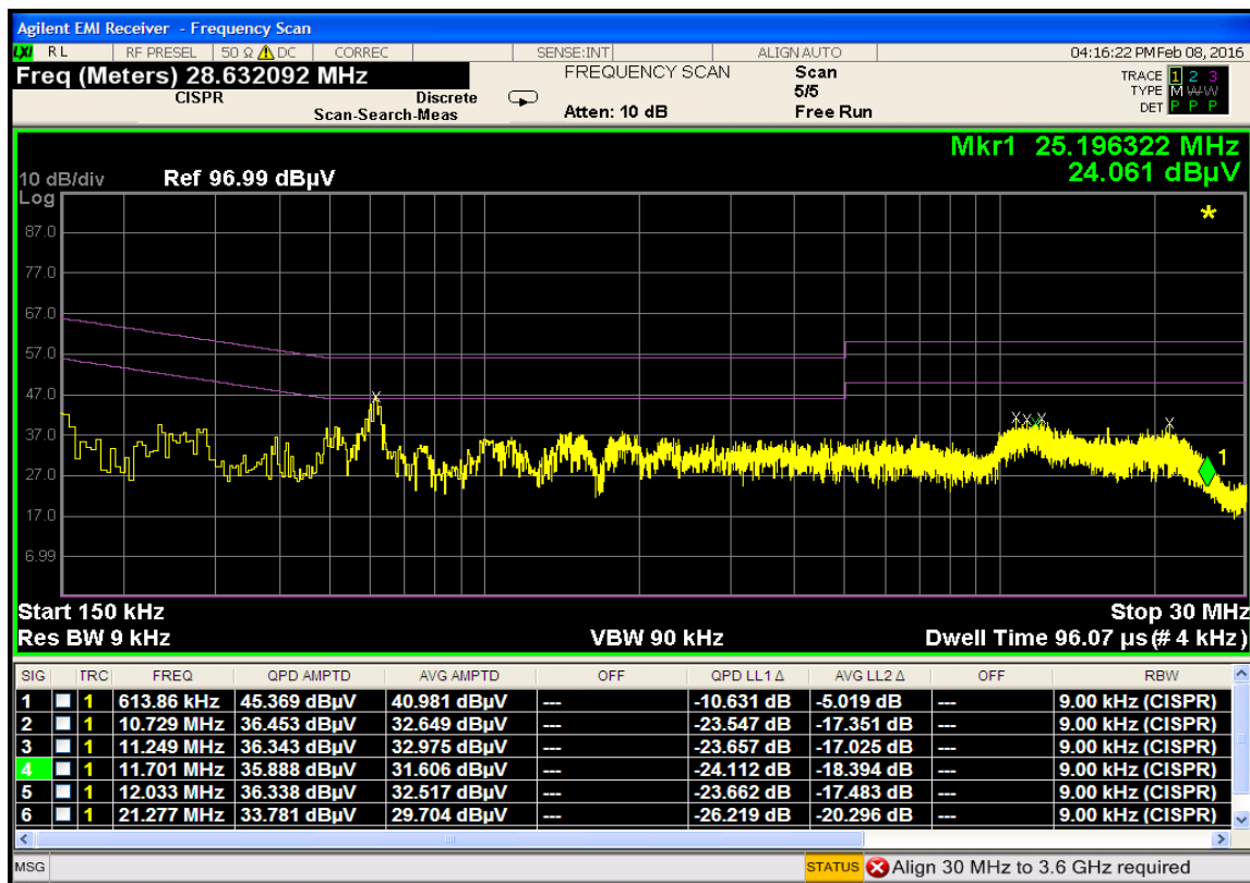
Plot 7-94. Line Conducted Plot with 802.11a UNII Band 1 (N)
