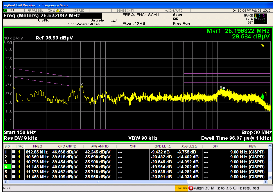
Plot 7-97. Line Conducted Plot with 802.11a UNII Band 2C (L1)
