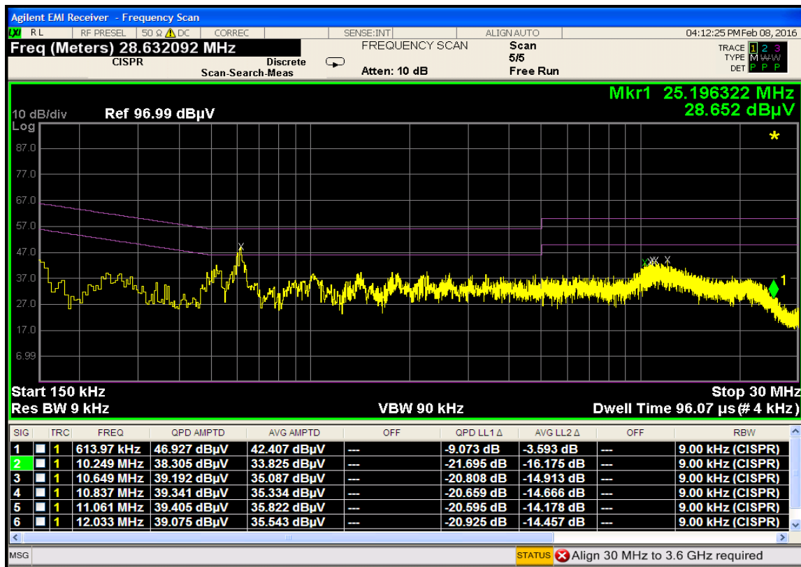
Plot 7-93. Line Conducted Plot with 802.11a UNII Band 1 (L1)
