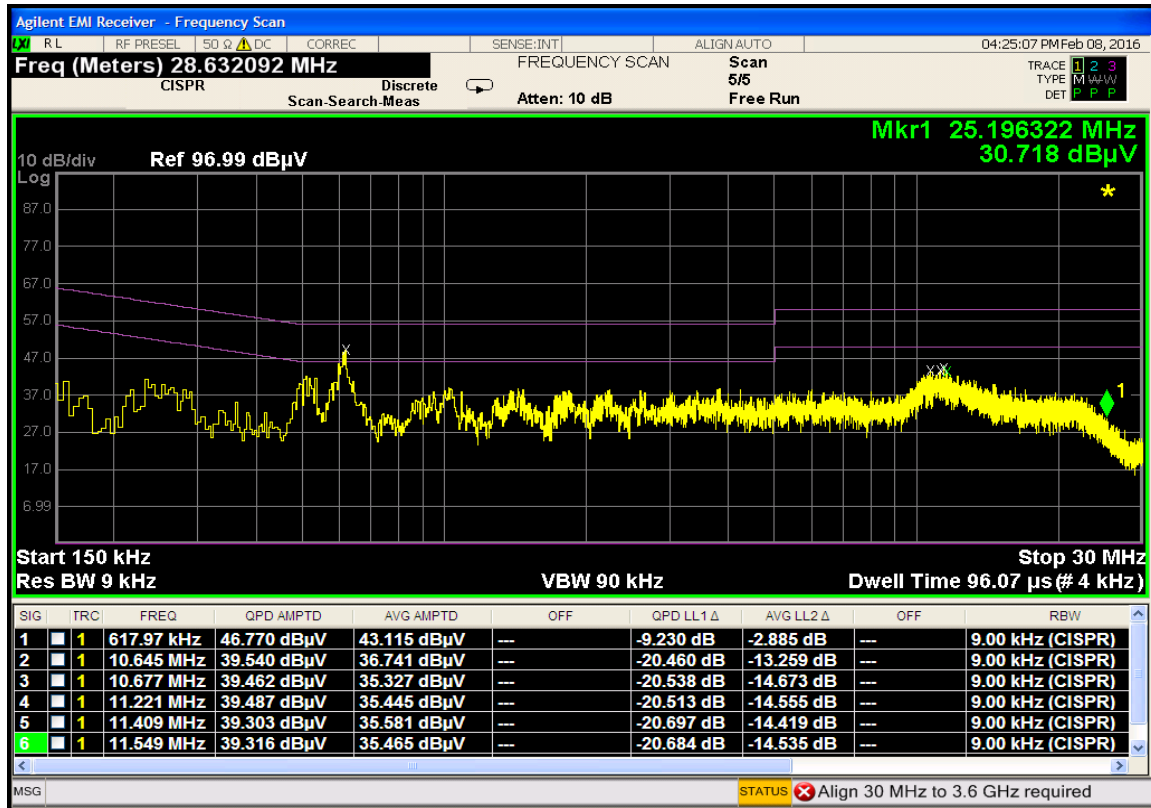
Plot 7-95. Line Conducted Plot with 802.11a UNII Band 2A (L1)
