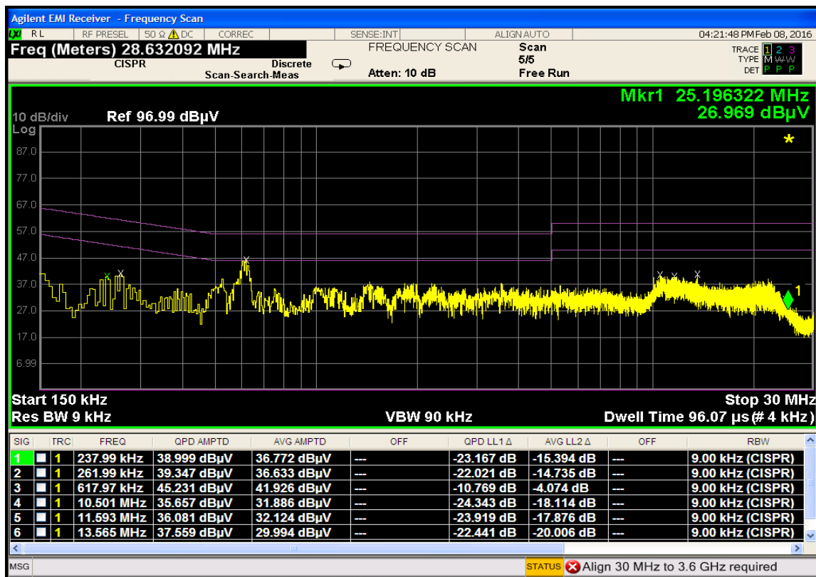
Plot 7-96. Line Conducted Plot with 802.11a UNII Band 2A (N)
