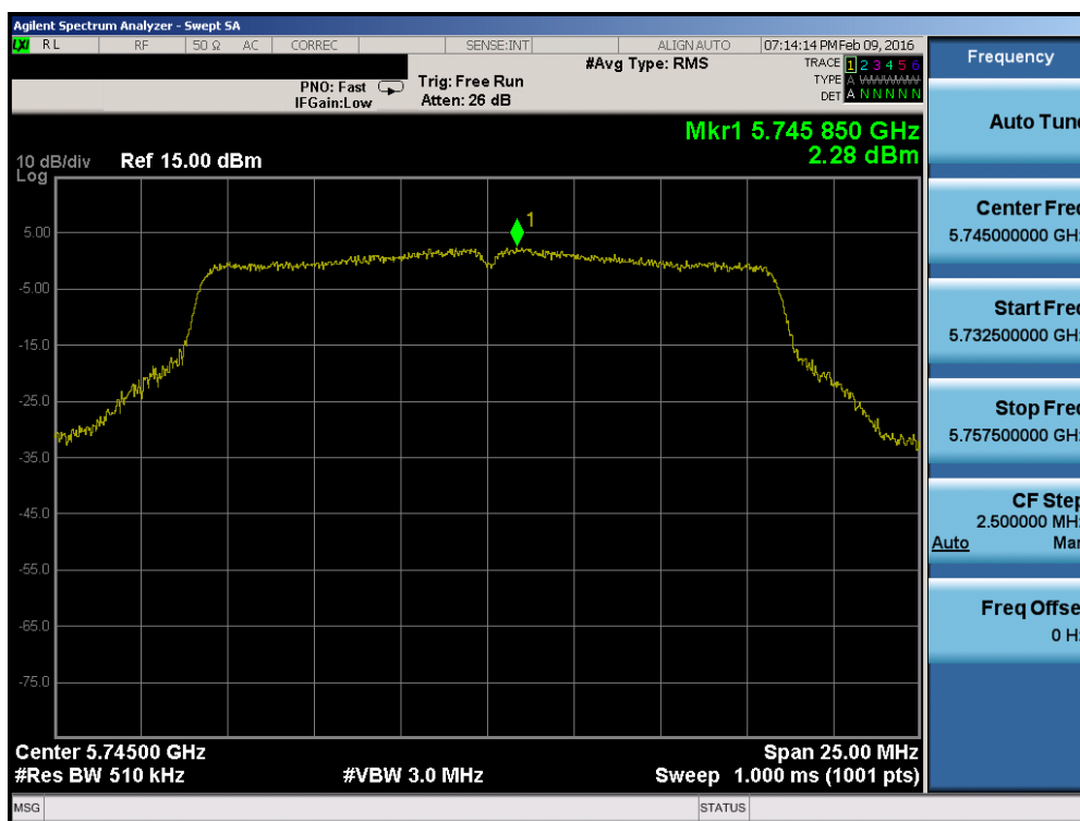
Plot 7-59. Power Spectral Density Plot (802.11a (UNII Band 3) – Ch. 149)
