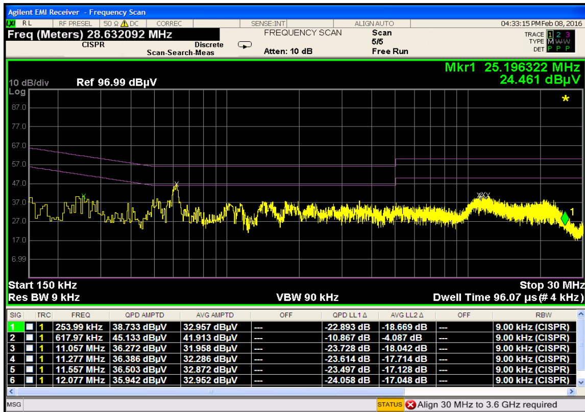
Plot 7-98. Line Conducted Plot with 802.11a UNII Band 2C (N)
