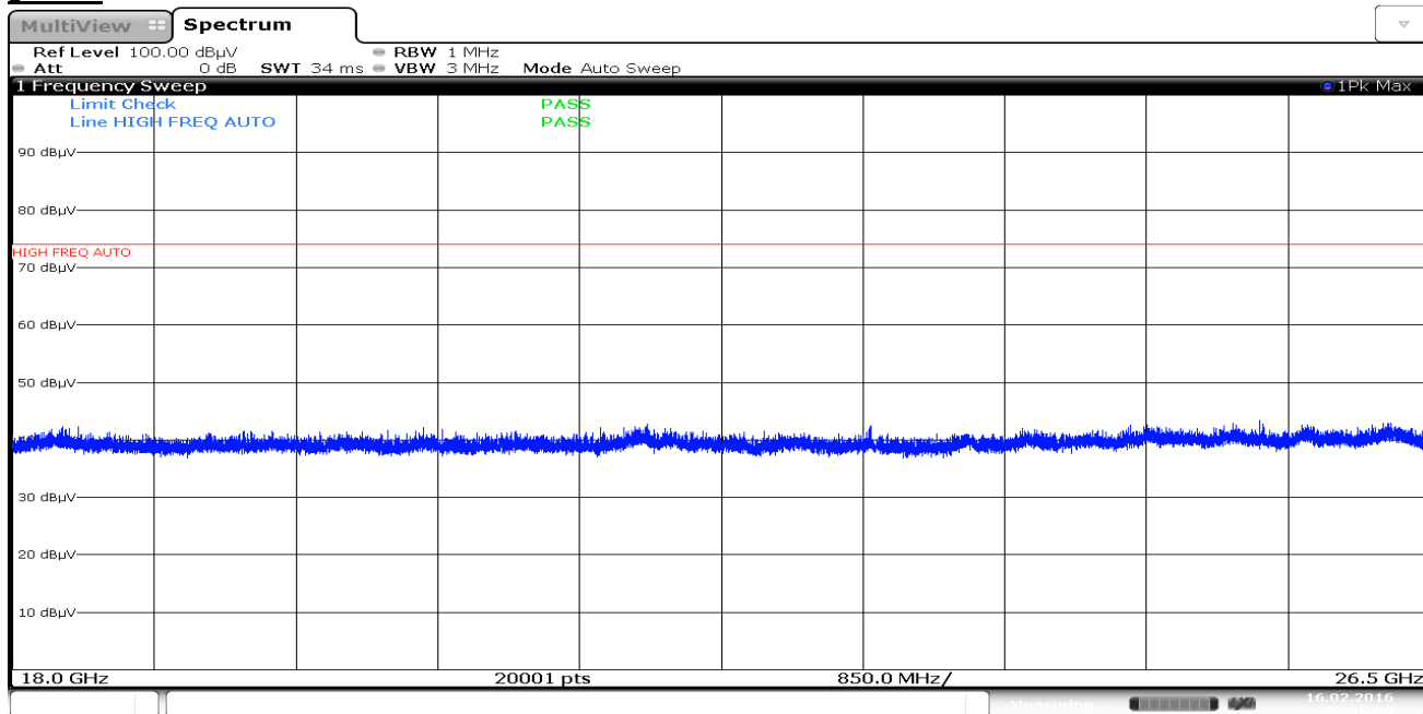
Plot 7-75. Radiated Spurious Plot above 18GHz (802.11a – Ant. Pol. H)
