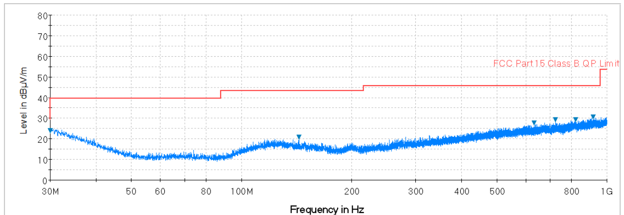
Plot 7-92. Radiated Spurious Plot below 1GHz (802.11a – U3 Ch. 157, Ant. Pol. V)
