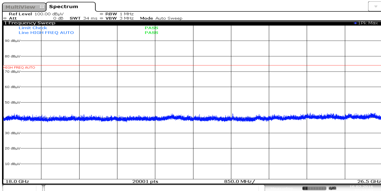
Plot 7-76. Radiated Spurious Plot above 18GHz (802.11a – Ant. Pol. V)
