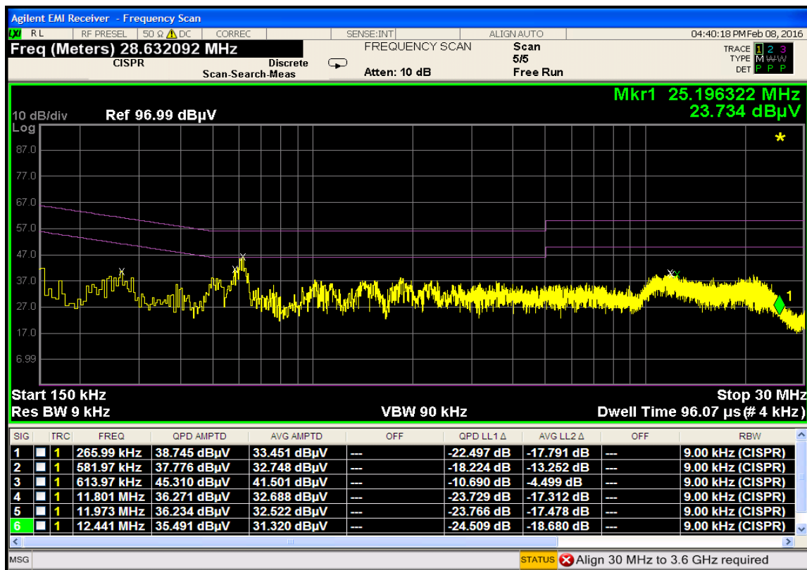
Plot 7-100. Line Conducted Plot with 802.11a UNII Band 3 (N)
