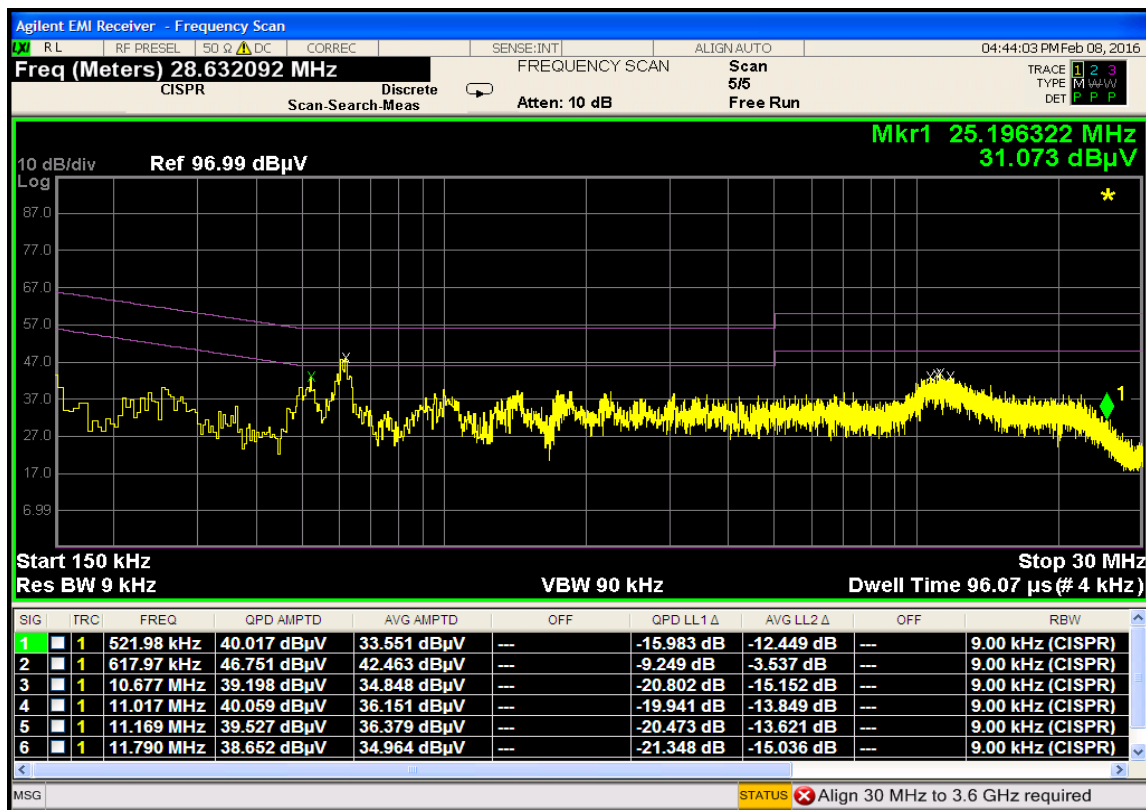
Plot 7-99. Line Conducted Plot with 802.11a UNII Band 3 (L1)
