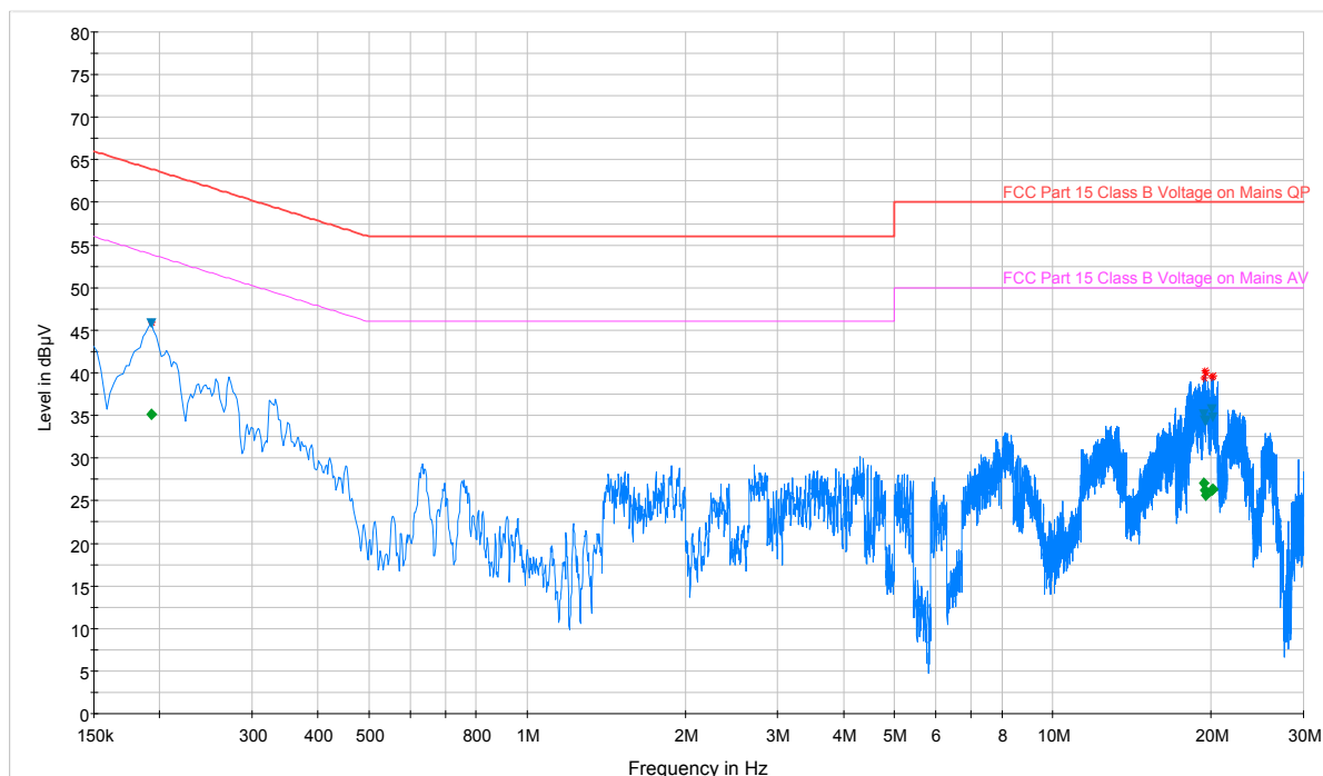
Plot 7-21. Line Conducted Plot with Bluetooth LE (N)
