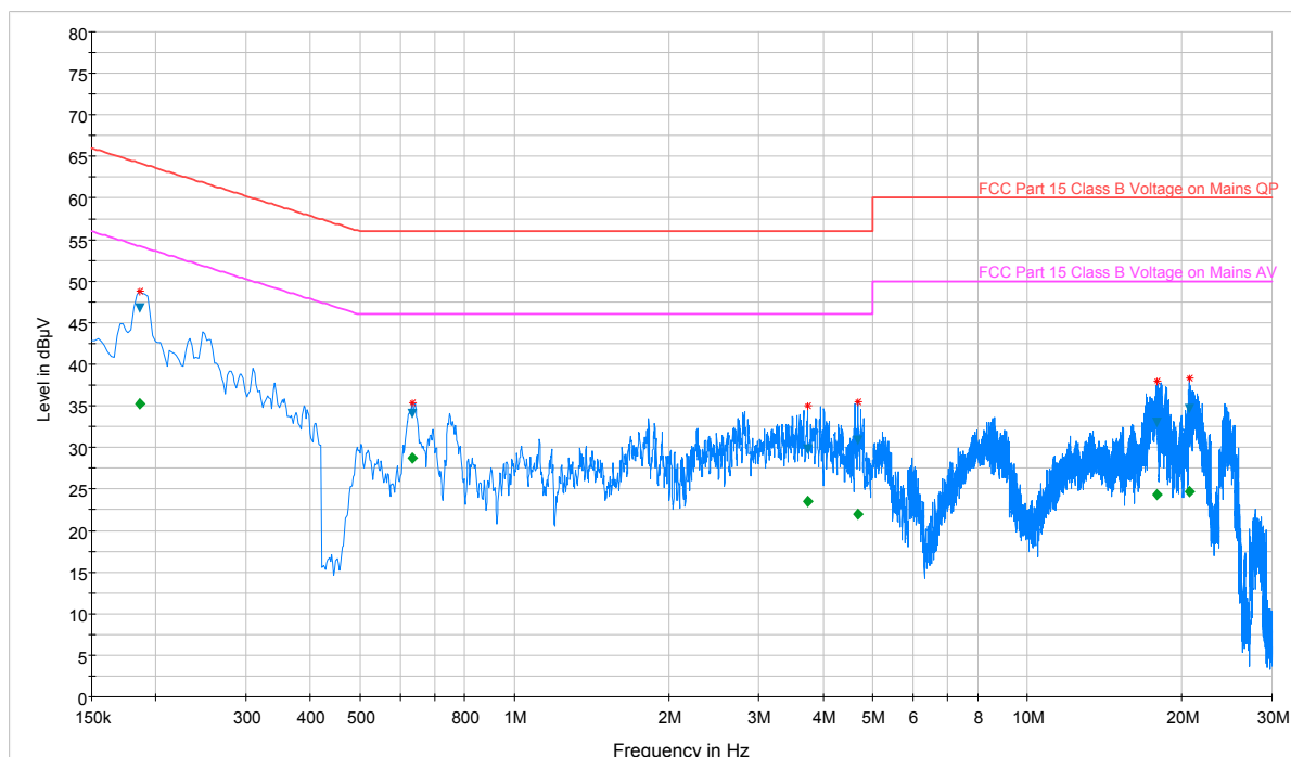
Plot 7-20. Line Conducted Plot with Bluetooth LE (L1)
