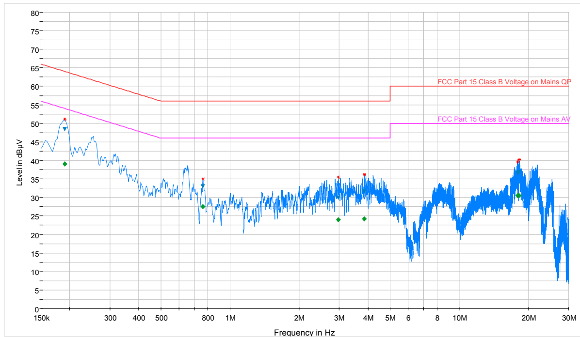
Plot 7-54. Line-Conducted Test Plot (L1)
