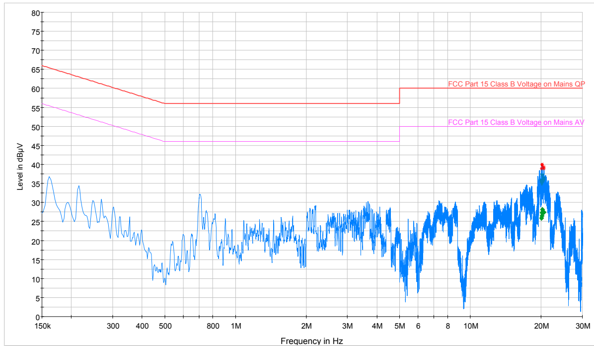
Plot 7-55. Line-Conducted Test Plot (N)
