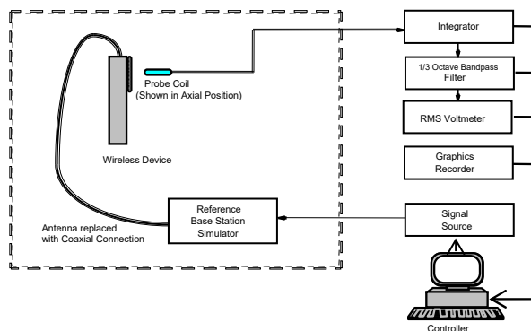
Figure 4-13 Audio Magnetic Field Test Setup
