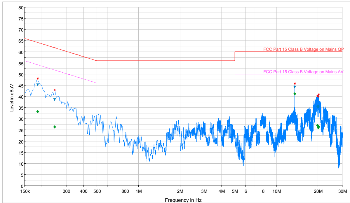
Plot 7-2. Line-Conducted Test Plot (N)
