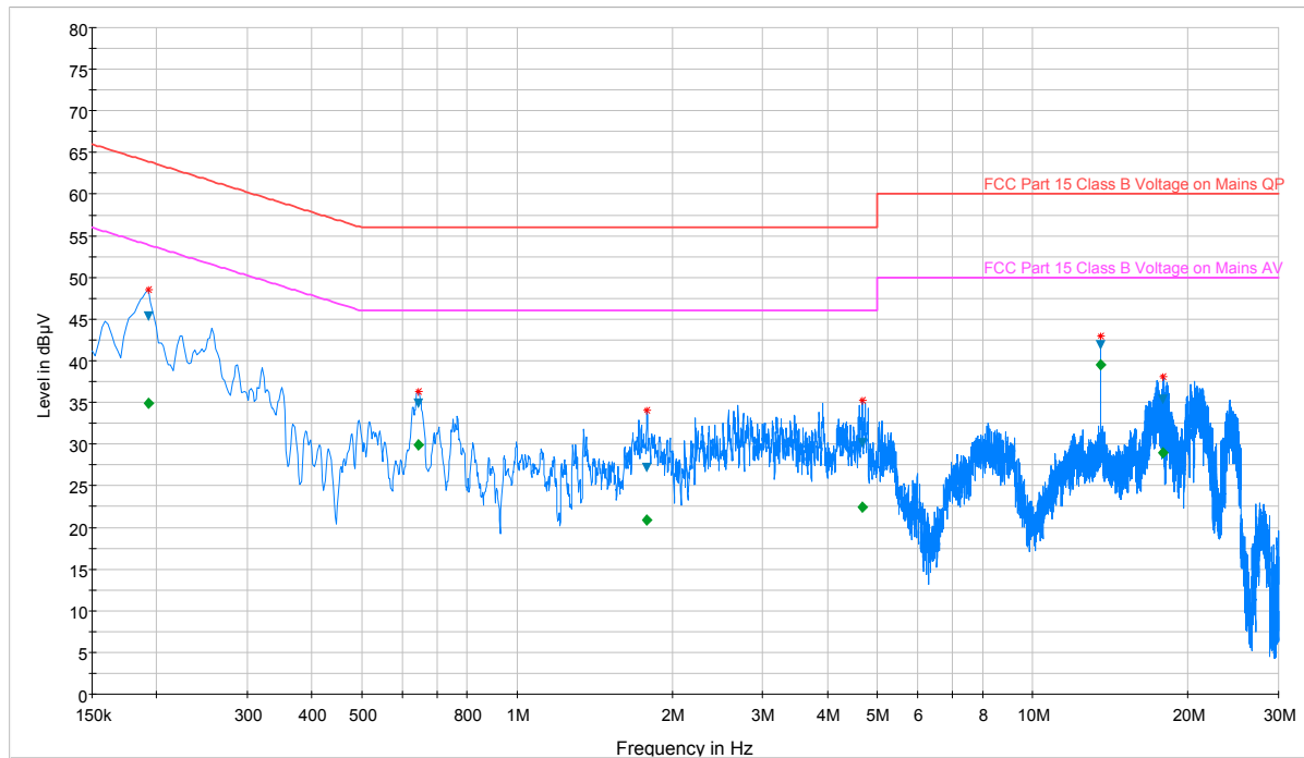
Plot 7-1. Line-Conducted Test Plot (L1)
