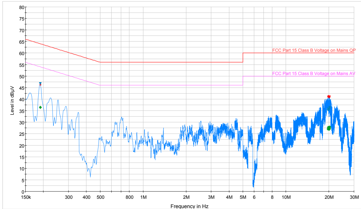
Plot 7-95. Line Conducted Plot with 802.11a UNII Band 1 (N)
