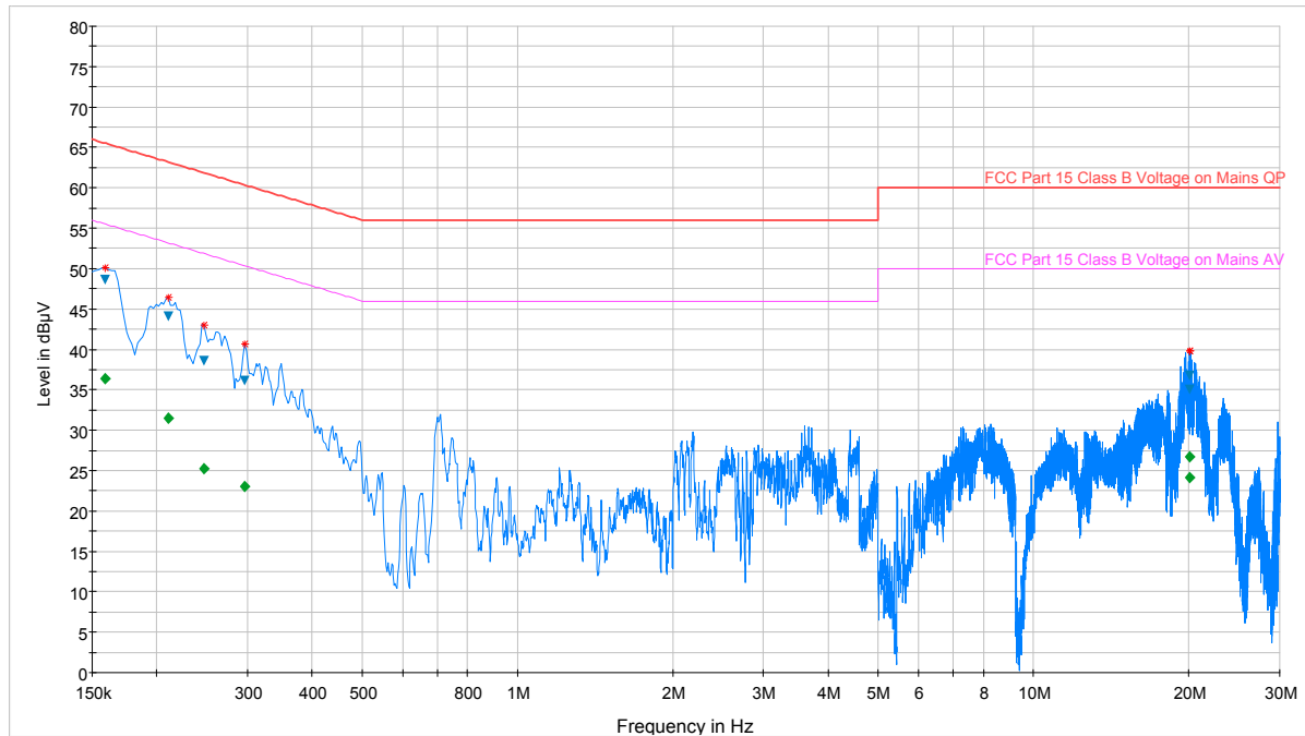
Plot 7-101. Line Conducted Plot with 802.11a UNII Band 3 (N)
