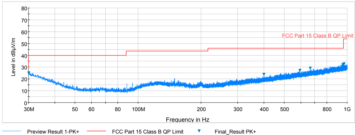
Plot 7-93. Radiated Spurious Plot below 1GHz (802.11a – U3 Ch. 157, Ant. Pol. V)
