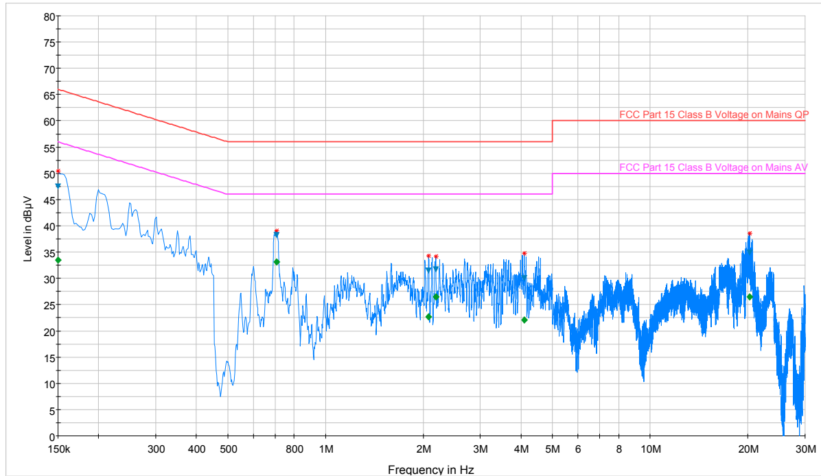
Plot 7-96. Line Conducted Plot with 802.11a UNII Band 2A (L1)
