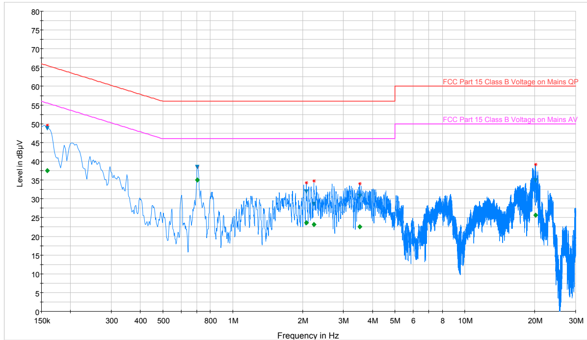
Plot 7-98. Line Conducted Plot with 802.11a UNII Band 2C (L1)
