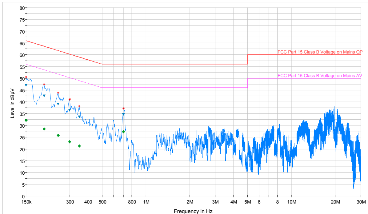
Plot 7-97. Line Conducted Plot with 802.11a UNII Band 2A (N)
