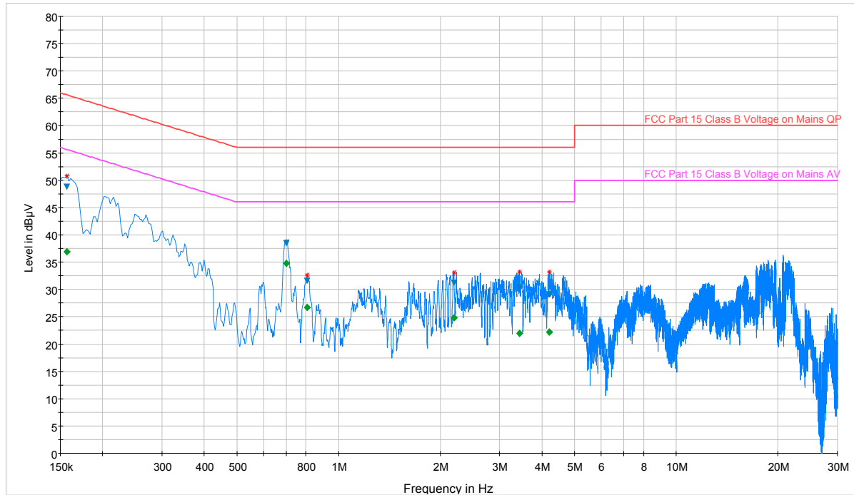
Plot 7-100. Line Conducted Plot with 802.11a UNII Band 3 (L1)
