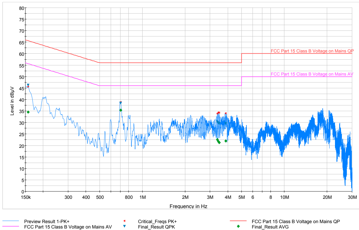
Plot 7-94. Line Conducted Plot with 802.11a UNII Band 1 (L1)
