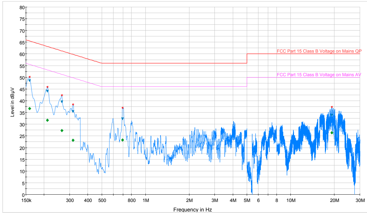
Plot 7-99. Line Conducted Plot with 802.11a UNII Band 2C (N)
