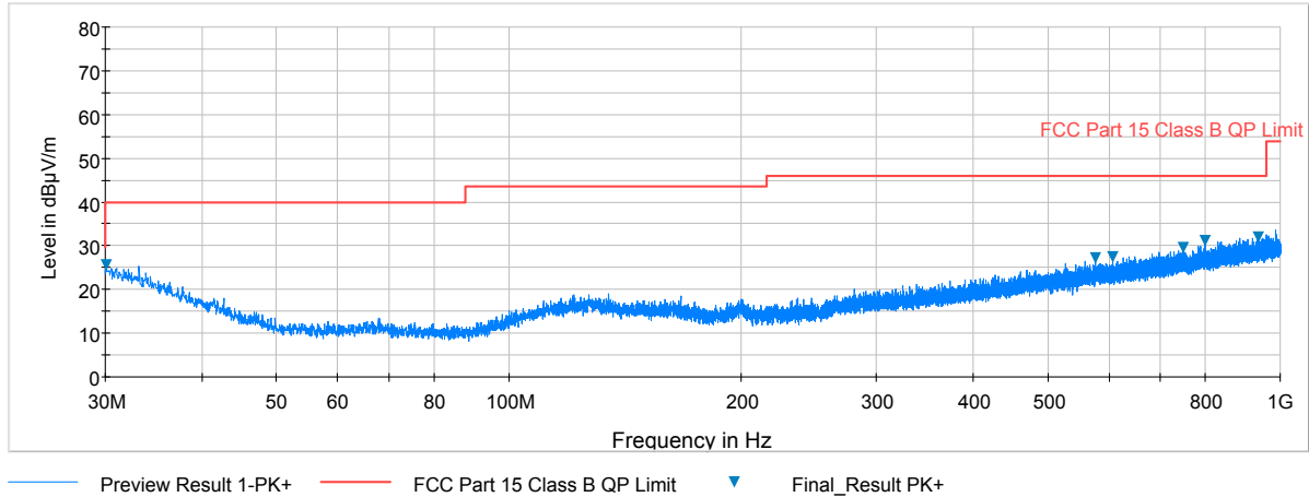
Plot 7-92. Radiated Spurious Plot below 1GHz (802.11a – U3 Ch. 157, Ant. Pol. H)
