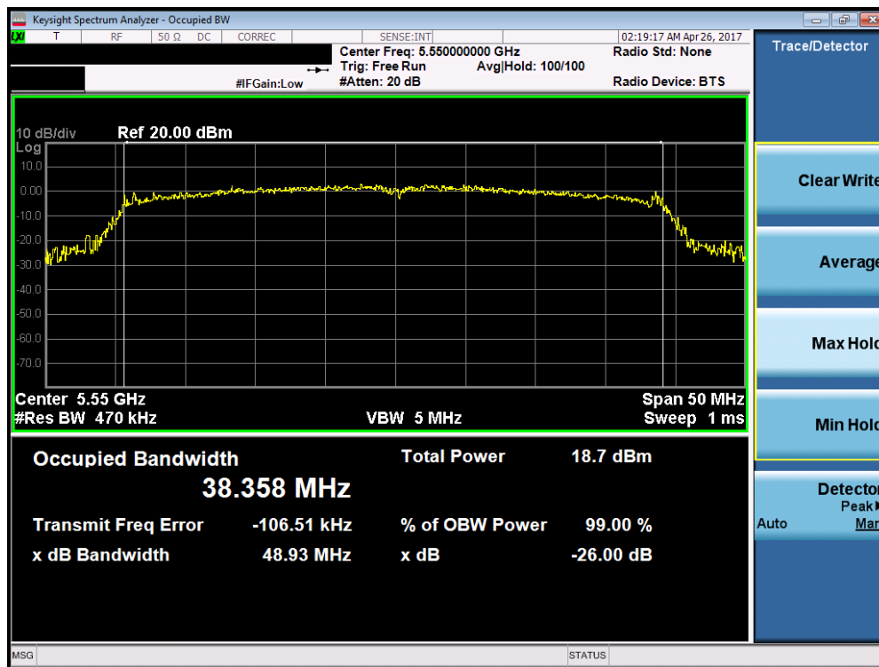
Plot 7-24. 26dB Bandwidth Plot (40MHz BW 802.11n (UNII Band 2C) – Ch. 110)
