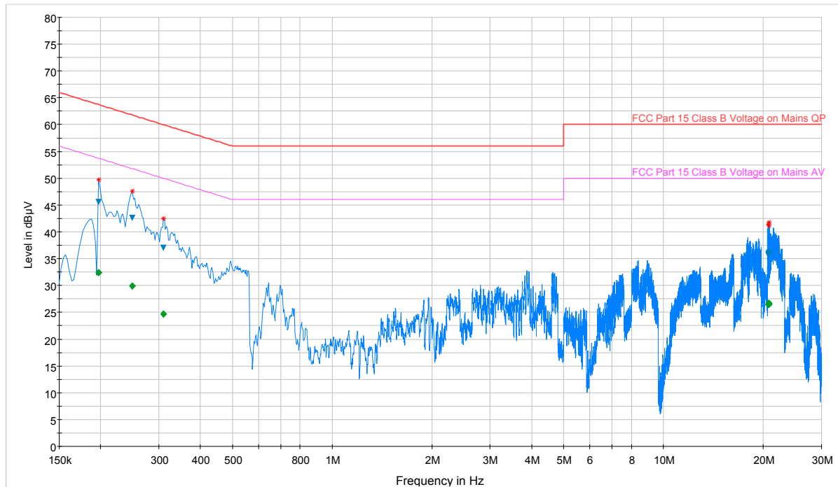
Plot 7-46. Line Conducted Plot with 802.11b (N)
