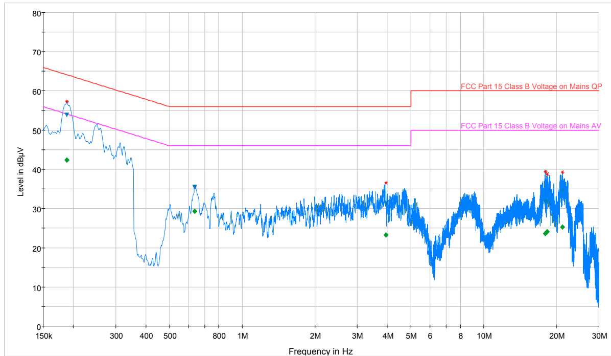
Plot 7-45. Line Conducted Plot with 802.11b (L1)
