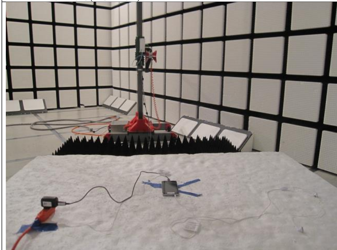
RADIATED BACK PHOTO (ABOVE 1 GHz)
