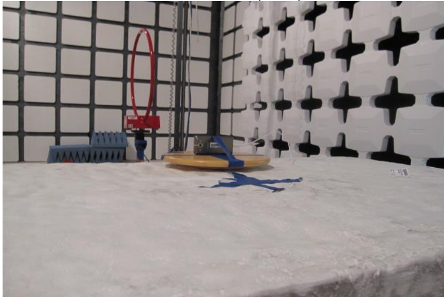
RADIATED EMISSIONS BELOW 30MHz (BACK)
