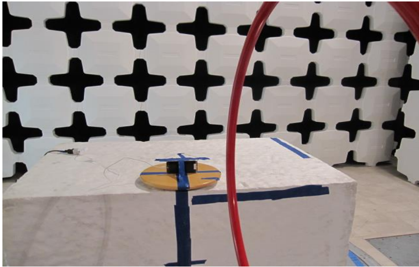
RADIATED EMISSIONS BELOW 30MHz (FRONT)
