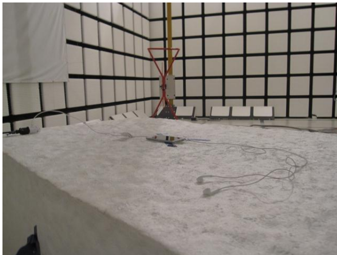
RADIATED FRONT PHOTO (BELOW 1 GHz)
