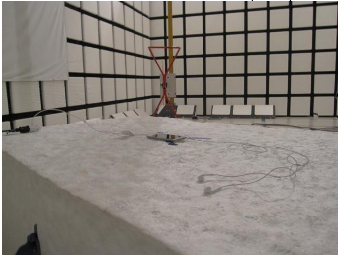
RADIATED EMISSIONS ABOVE 30 MHz (BACK)
