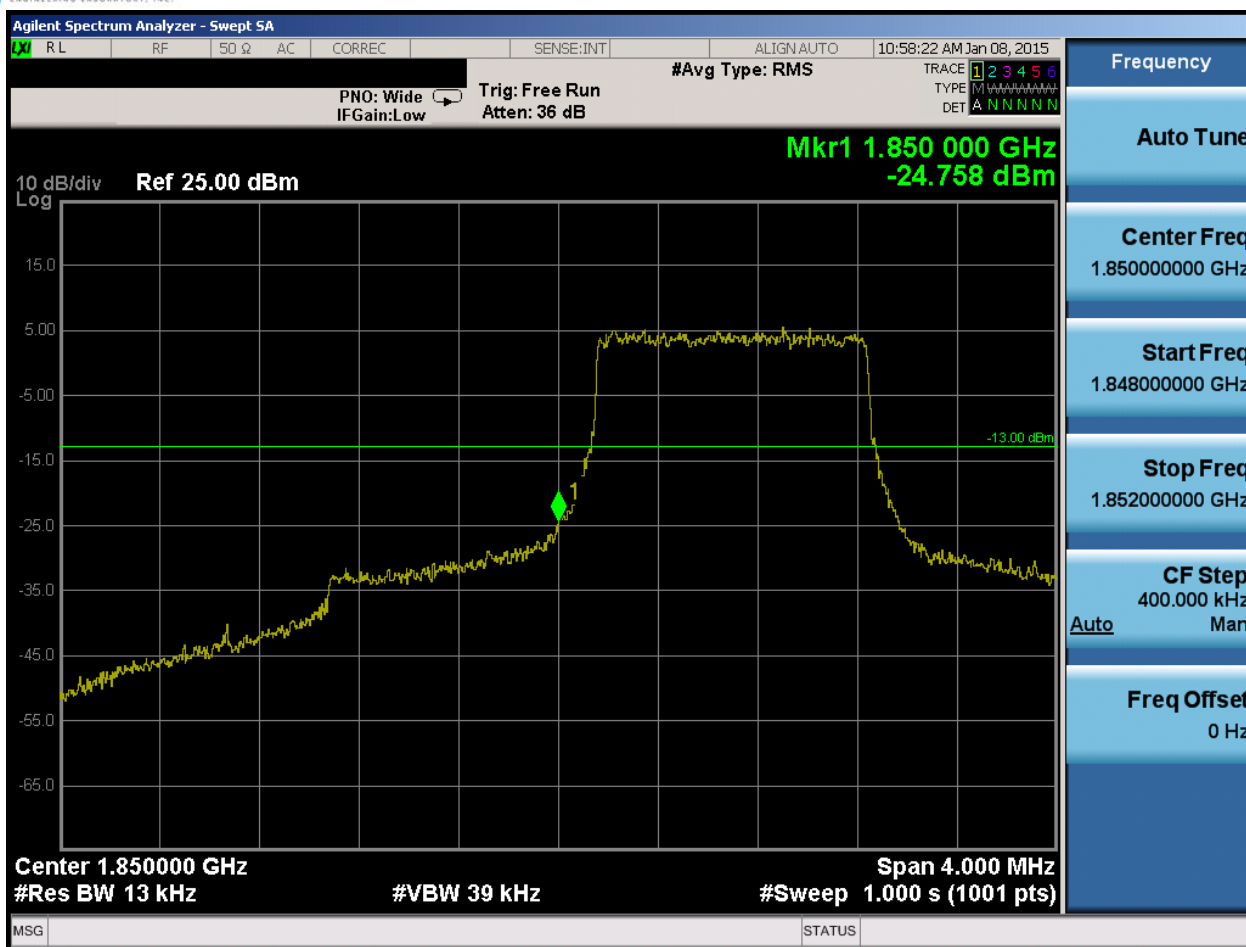
Plot 6-117. Lower Band Edge Plot (Band 2 – 1.4MHz QPSK – RB Size 6)
