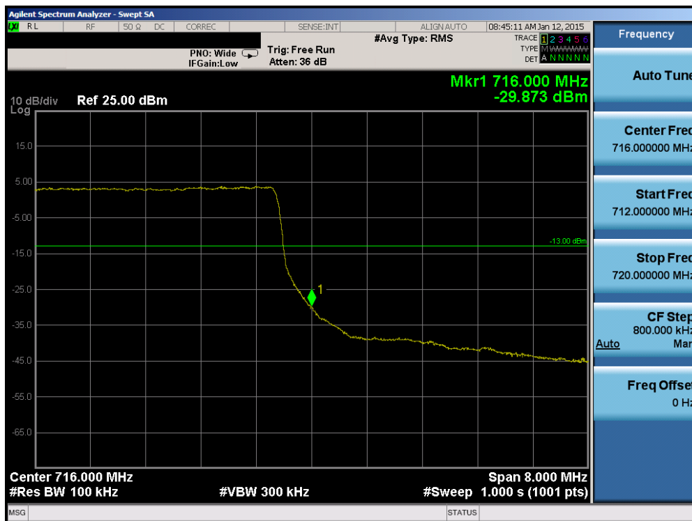
Plot 6-78. Upper Band Edge Plot (Band 17 – 10.0MHz QPSK – RB Size 50)
