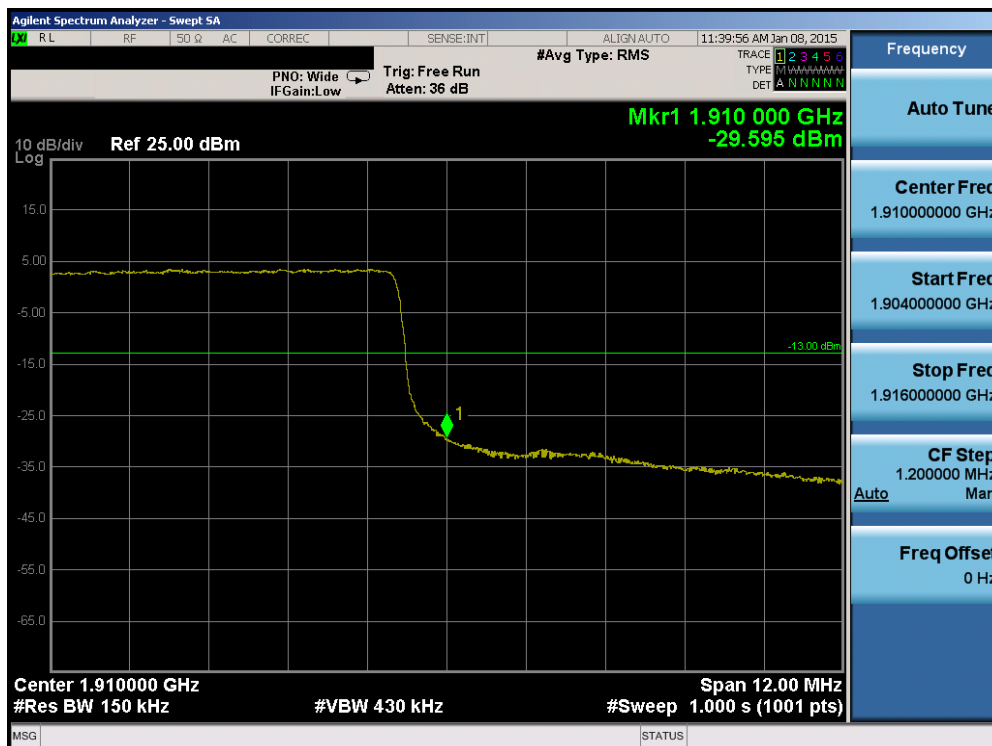
Plot 6-135. Upper Band Edge Plot (Band 2 – 15.0MHz QPSK – RB Size 75)
