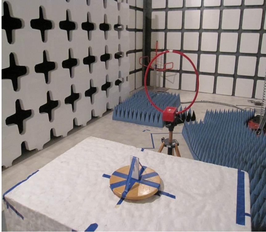
RADIATED EMISSIONS BELOW 30MHz (BACK)
