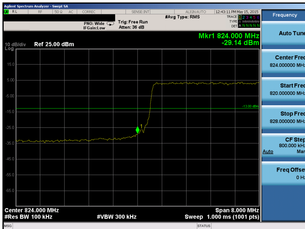
Plot 6-122. Lower Band Edge Plot (Band 5/26 - 10.0MHz QPSK - RB Size 50)
