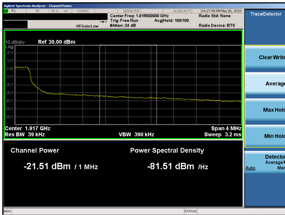
Plot 6-161. Upper Extended Band Edge Plot (Band 2/25 – 5.0MHz QPSK – RB Size 25)
