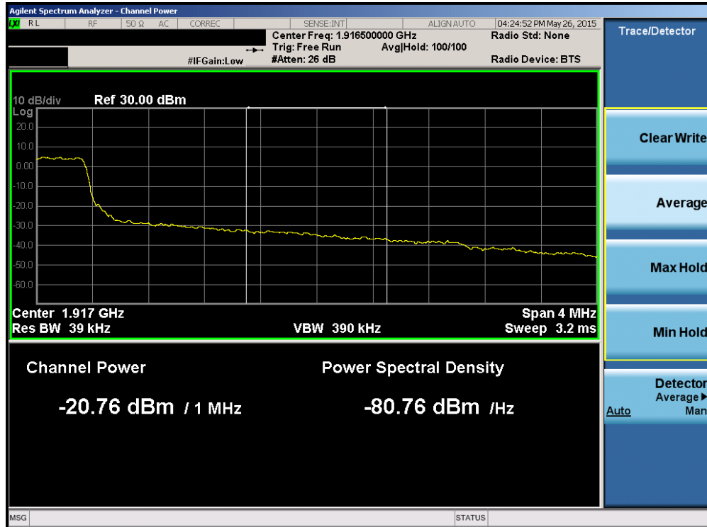
Plot 6-157. Upper Extended Band Edge Plot (Band 2/25 – 3.0MHz QPSK – RB Size 15)
