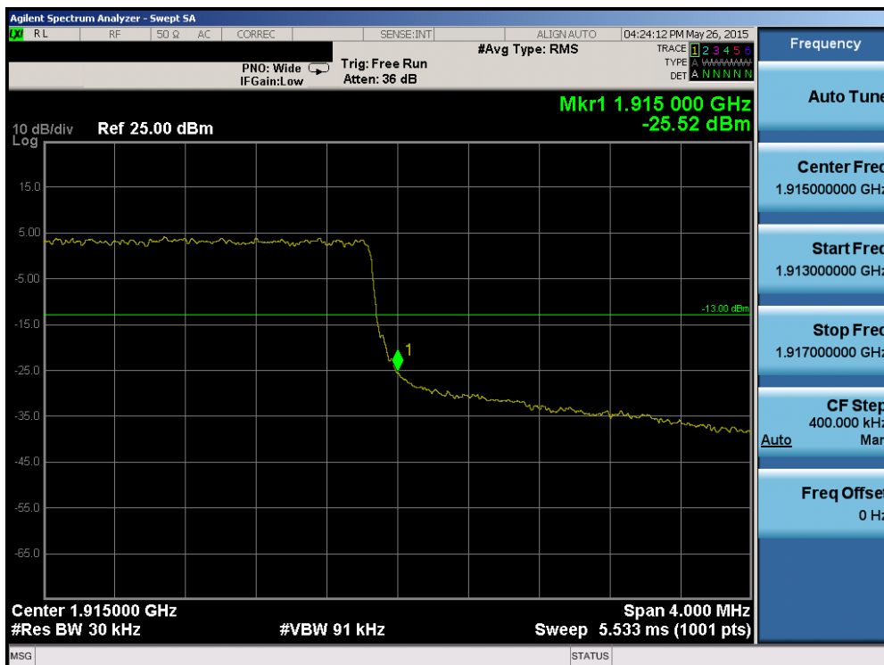
Plot 6-156. Upper Band Edge Plot (Band 2/25 – 3.0MHz QPSK – RB Size 15)
