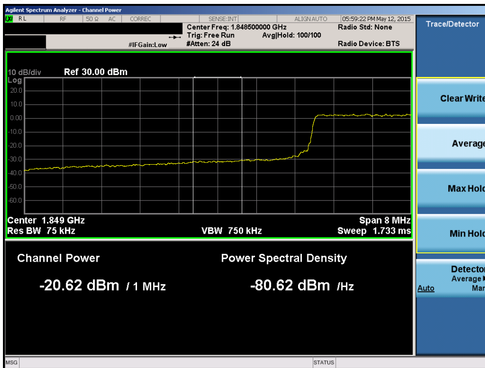
Plot 6-163. Lower Extended Band Edge Plot (Band 2/25 – 10.0MHz QPSK – RB Size 50)
