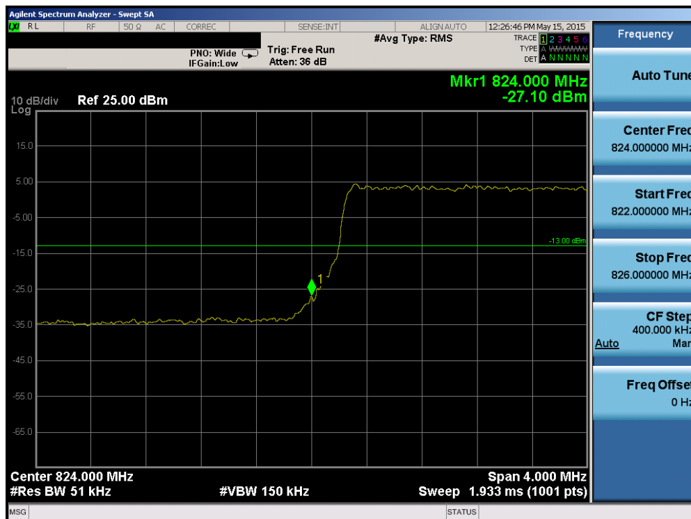
Plot 6-118. Lower Band Edge Plot (Band 5/26 – 5.0MHz QPSK – RB Size 25)
