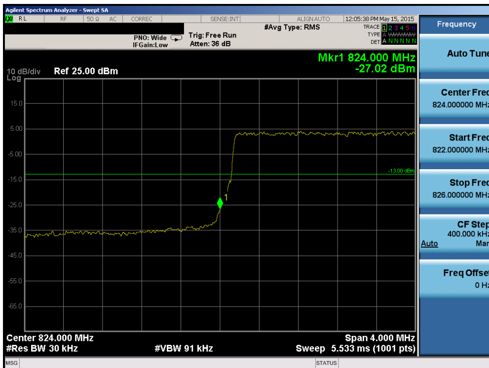
Plot 6-114. Lower Band Edge Plot (Band 5/26 - 3.0MHz QPSK - RB Size 15)
