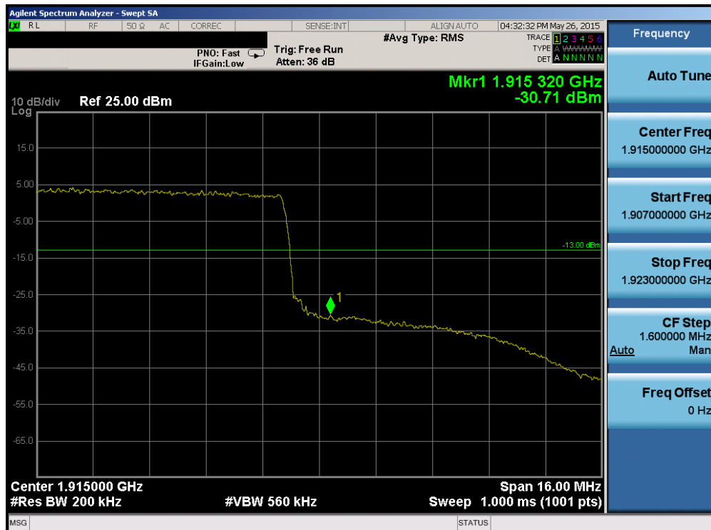
Plot 6-172. Upper Band Edge Plot (Band 2/25 – 20.0MHz QPSK – RB Size 100)
