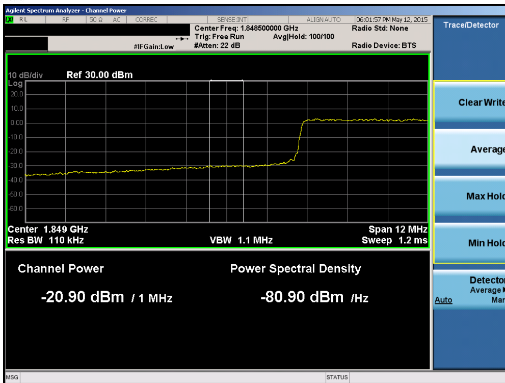
Plot 6-167. Lower Extended Band Edge Plot (Band 2/25 – 15.0MHz QPSK – RB Size 75)
