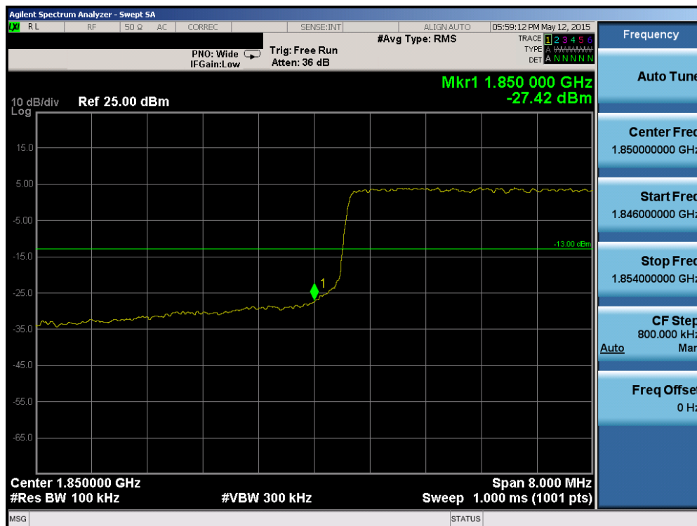
Plot 6-162. Lower Band Edge Plot (Band 2/25 – 10.0MHz QPSK – RB Size 50)
