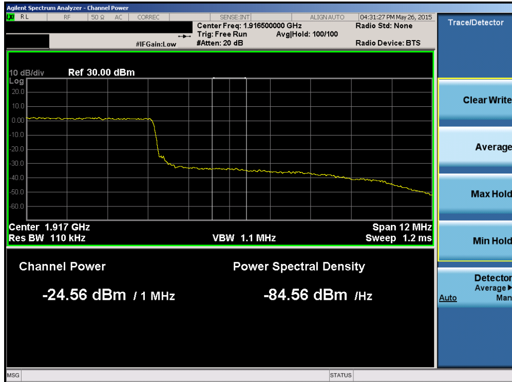
Plot 6-169. Upper Extended Band Edge Plot (Band 2/25 – 15.0MHz QPSK – RB Size 75)
