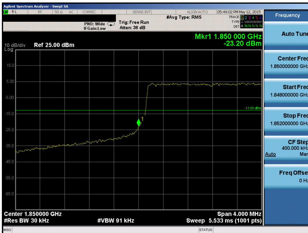
Plot 6-154. Lower Band Edge Plot (Band 2/25 – 3.0MHz QPSK – RB Size 15)
