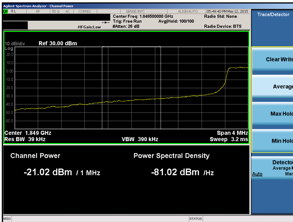
Plot 6-155. Lower Extended Band Edge Plot (Band 2/25 – 3.0MHz QPSK – RB Size 15)
