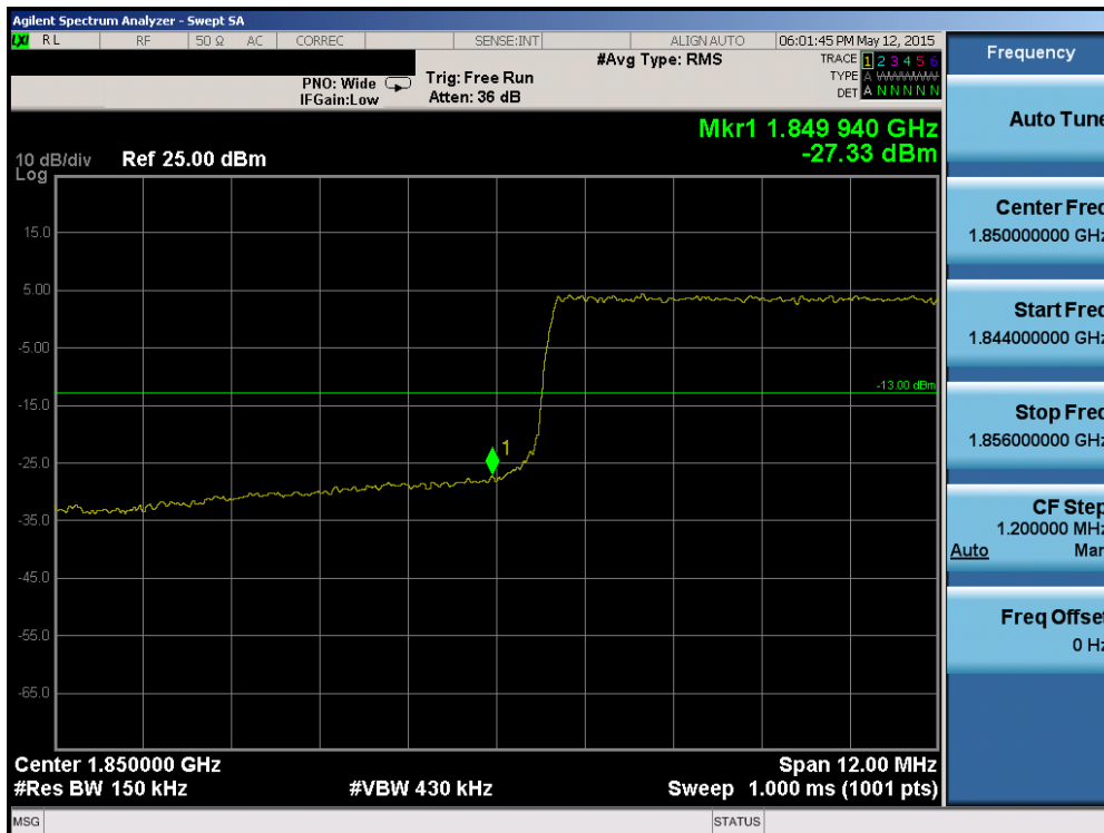
Plot 6-166. Lower Band Edge Plot (Band 2/25 – 15.0MHz QPSK – RB Size 75)
