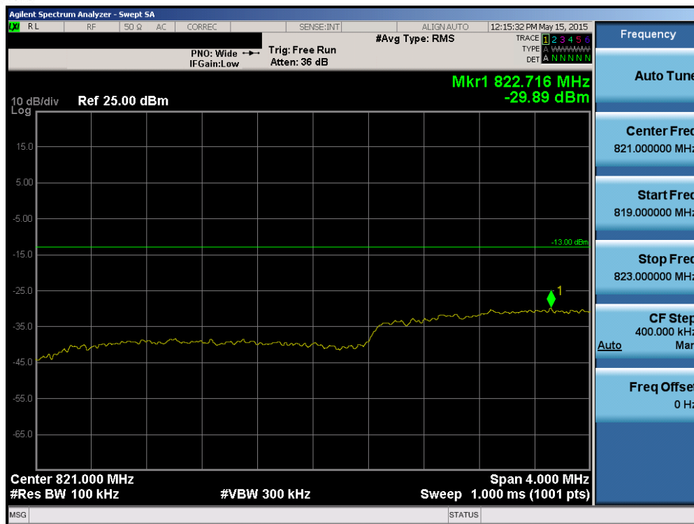
Plot 6-115. Lower Extended Band Edge Plot (Band 5/26 – 3.0MHz QPSK – RB Size 15)
