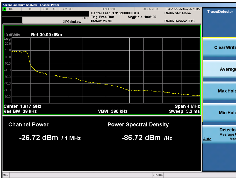
Plot 6-153. Upper Extended Band Edge Plot (Band 2/25 – 1.4MHz QPSK – RB Size 6)
