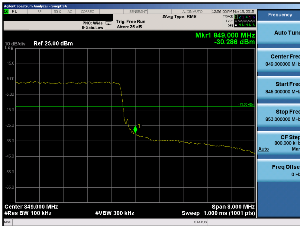
Plot 6-123. Upper Band Edge Plot (Band 5/26 – 10.0MHz QPSK – RB Size 50)
