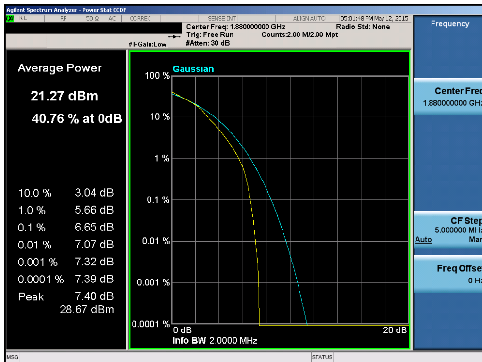
Plot 6-183. PAR Plot (Band 2/25 – 1.4MHz 16-QAM – RB Size 6)
