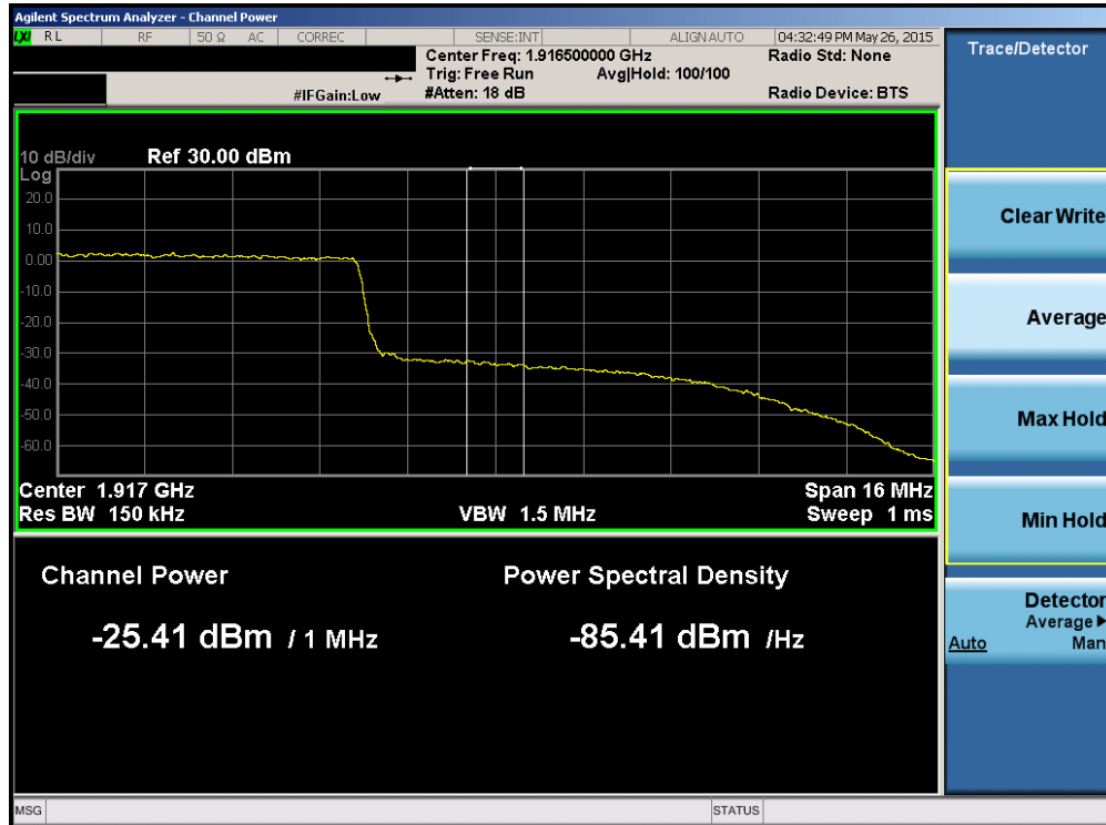
Plot 6-173. Upper Extended Band Edge Plot (Band 2/25 – 20.0MHz QPSK – RB Size 100)
