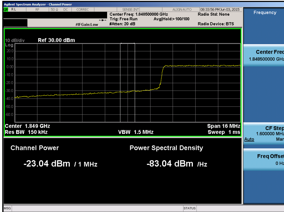
Plot 6-171. Lower Extended Band Edge Plot (Band 2/25 – 20.0MHz QPSK – RB Size 100)
