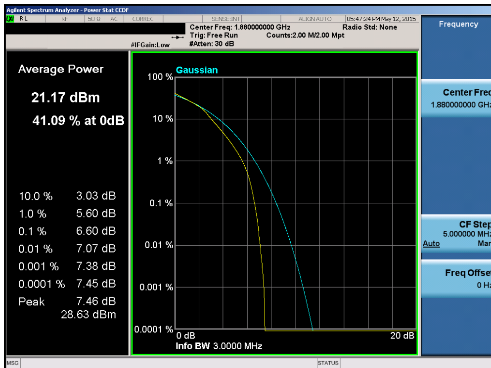
Plot 6-185. PAR Plot (Band 2/25 – 3.0MHz 16-QAM – RB Size 15)
