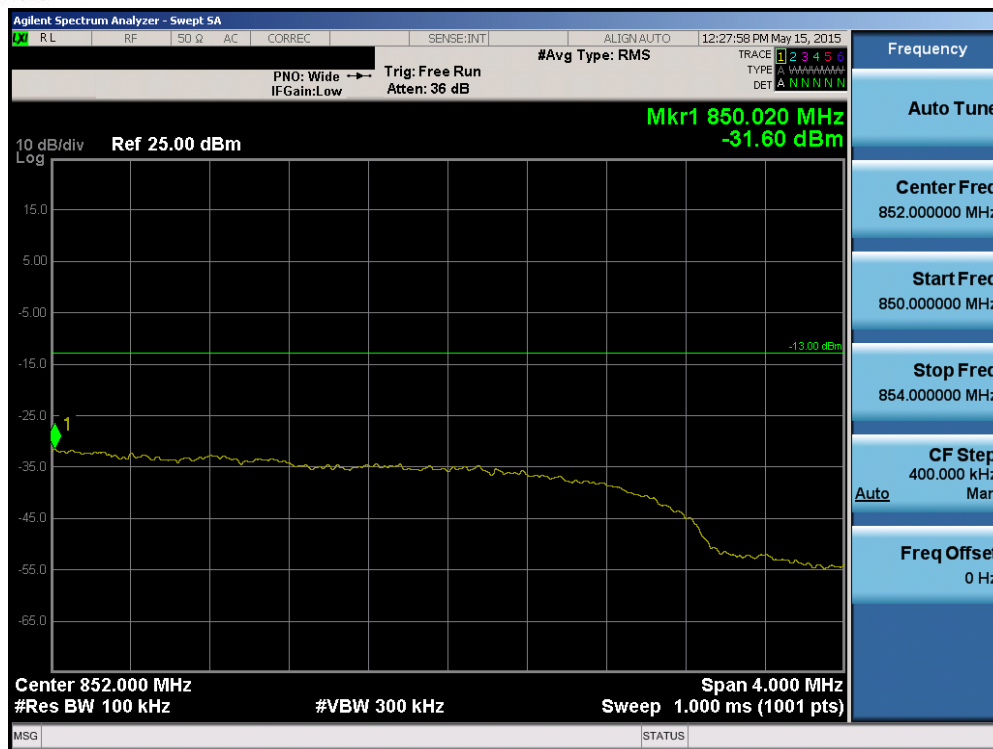
Plot 6-121. Upper Extended Band Edge Plot (Band 5/26 - 5.0MHz QPSK - RB Size 25)
