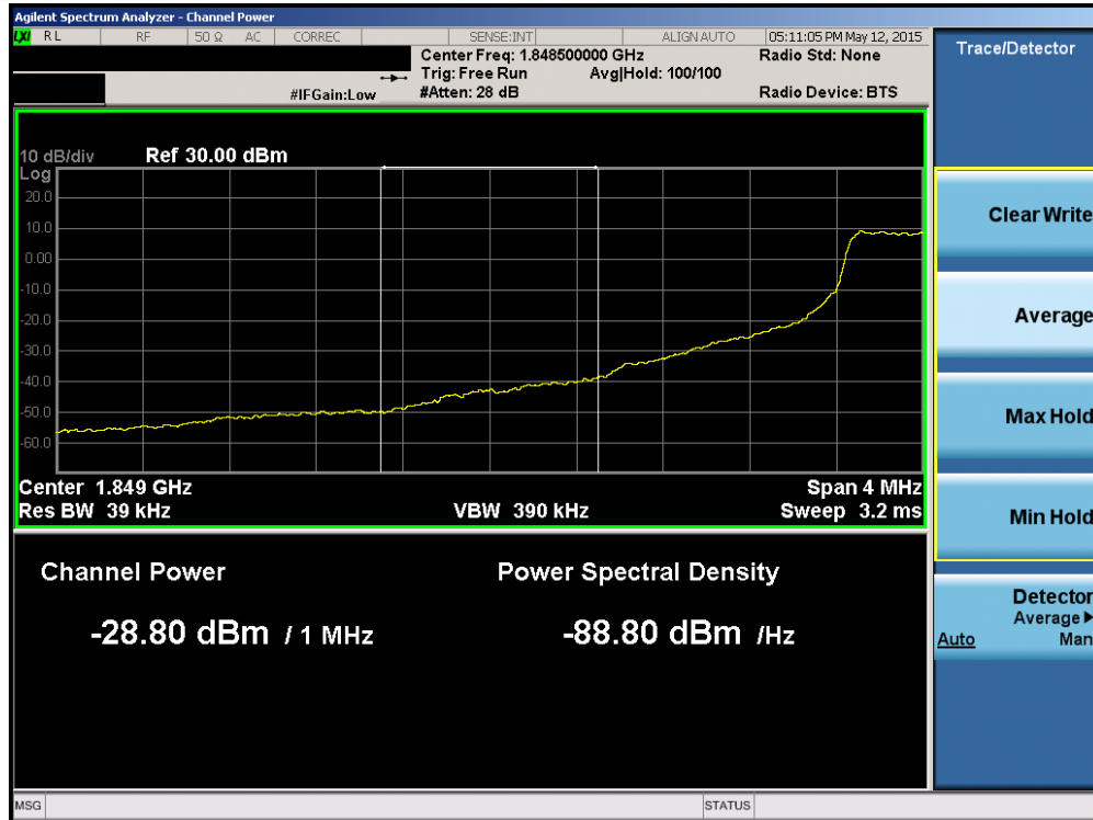
Plot 6-151. Lower Extended Band Edge Plot (Band 2/25 – 1.4MHz QPSK – RB Size 6)
