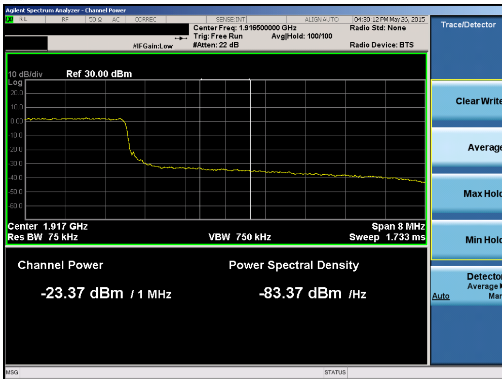
Plot 6-165. Upper Extended Band Edge Plot (Band 2/25 – 10.0MHz QPSK – RB Size 50)
