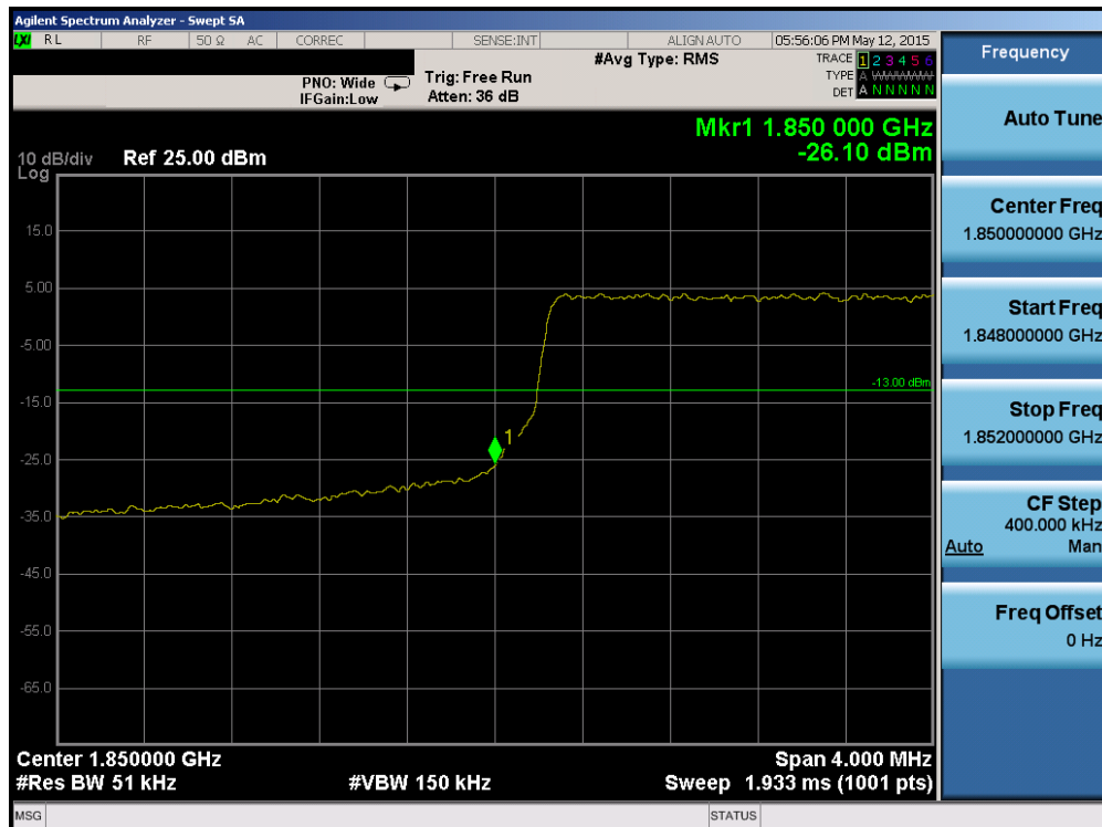
Plot 6-158. Lower Band Edge Plot (Band 2/25 – 5.0MHz QPSK – RB Size 25)
