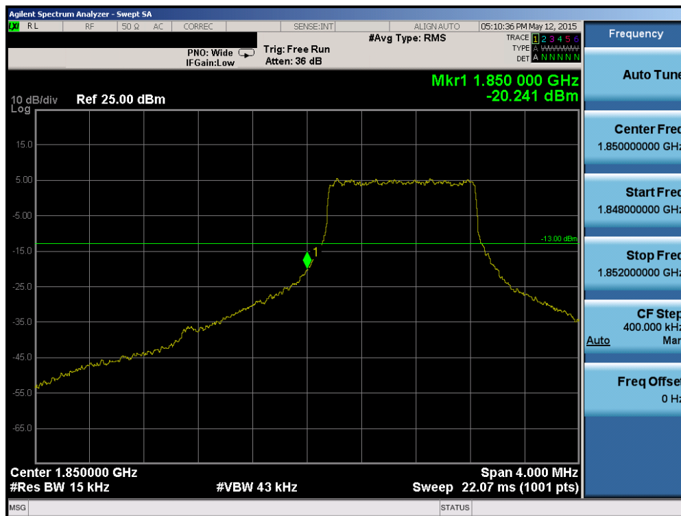
Plot 6-150. Lower Band Edge Plot (Band 2/25 – 1.4MHz QPSK – RB Size 6)
