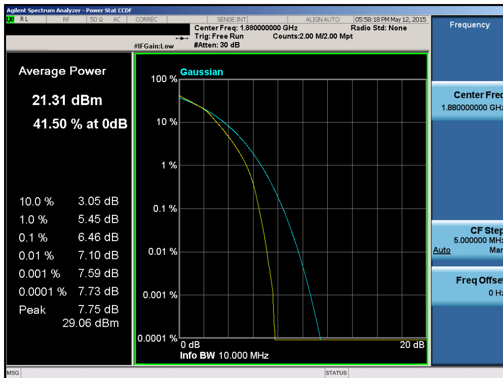
Plot 6-189. PAR Plot (Band 2/25 – 10.0MHz 16-QAM – RB Size 50)
