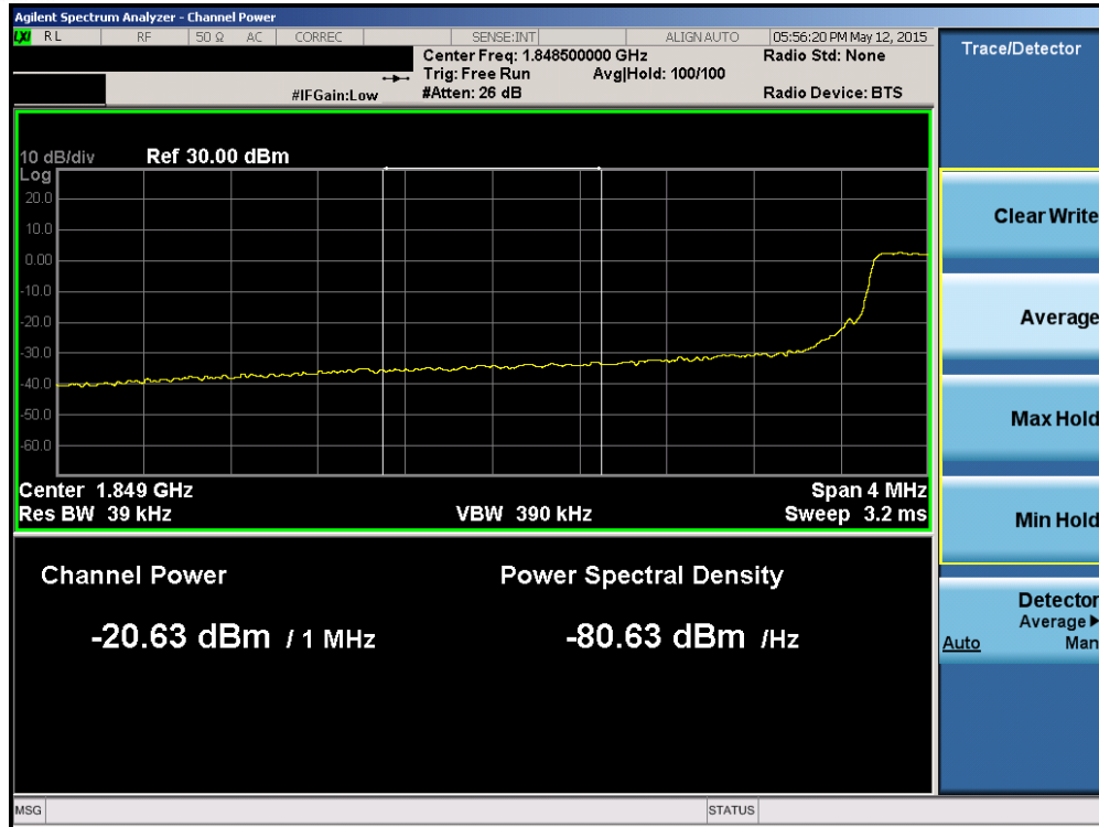
Plot 6-159. Lower Extended Band Edge Plot (Band 2/25 – 5.0MHz QPSK – RB Size 25)
