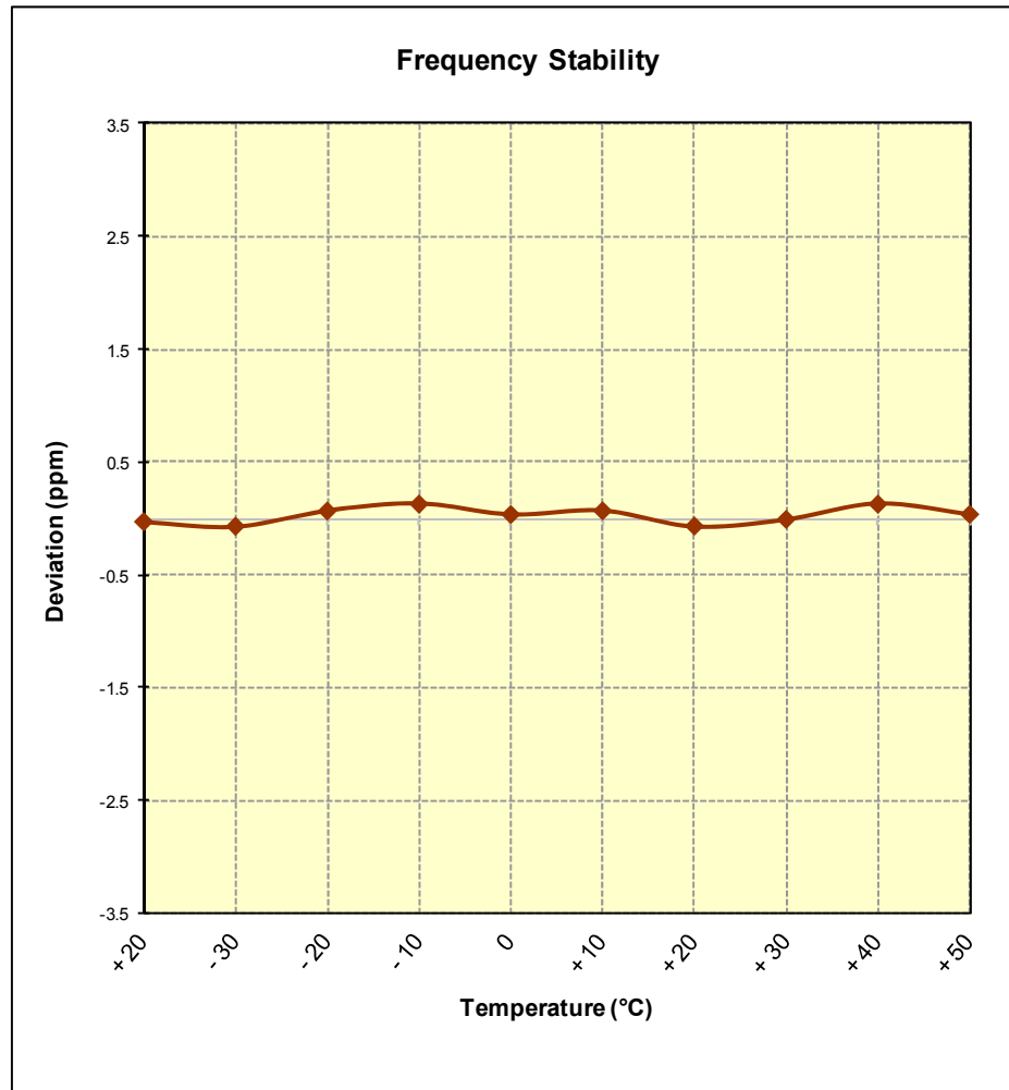
Figure 6-10. Frequency Stability Graph (Band 2/25)
