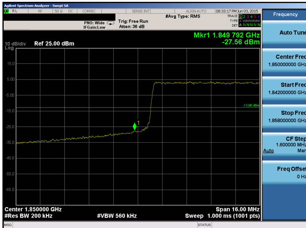
Plot 6-170. Lower Band Edge Plot (Band 2/25 – 20.0MHz QPSK – RB Size 100)
