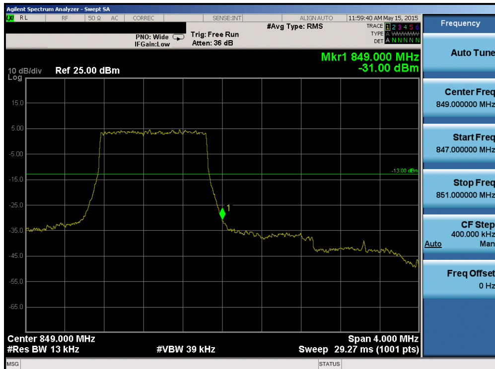
Plot 6-112. Upper Band Edge Plot (Band 5/26 – 1.4MHz QPSK – RB Size 6)
