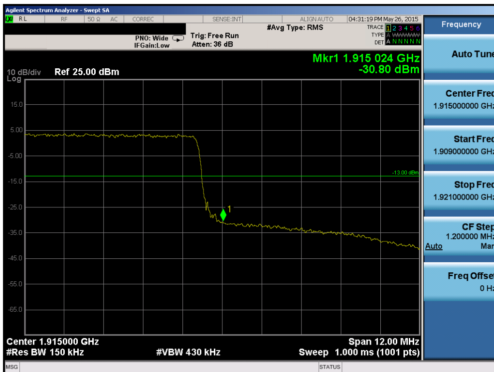
Plot 6-168. Upper Band Edge Plot (Band 2/25 – 15.0MHz QPSK – RB Size 75)
