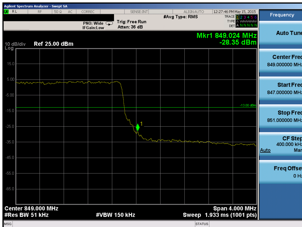
Plot 6-120. Upper Band Edge Plot (Band 5/26 – 5.0MHz QPSK – RB Size 25)
