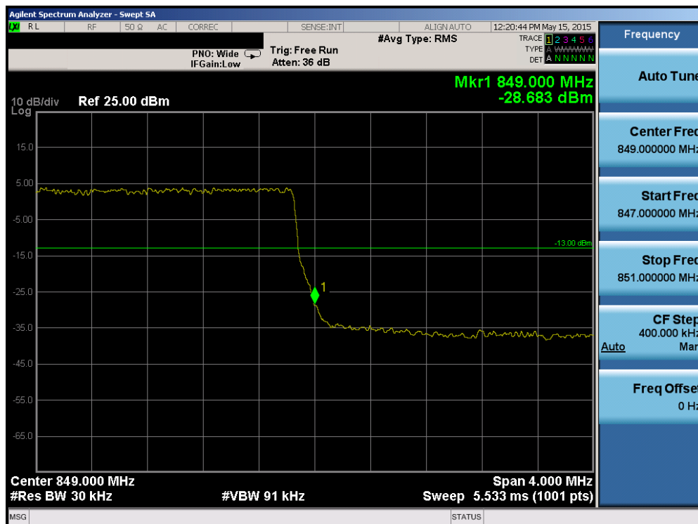
Plot 6-116. Upper Band Edge Plot (Band 5/26 – 3.0MHz QPSK – RB Size 15)
