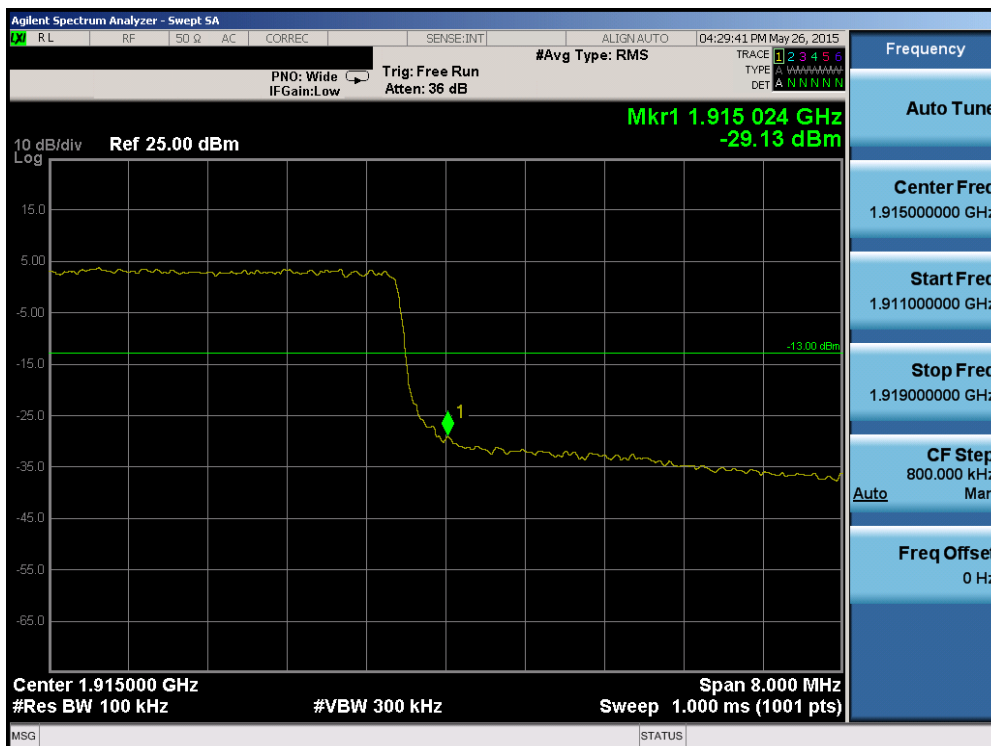
Plot 6-164. Upper Band Edge Plot (Band 2/25 – 10.0MHz QPSK – RB Size 50)
