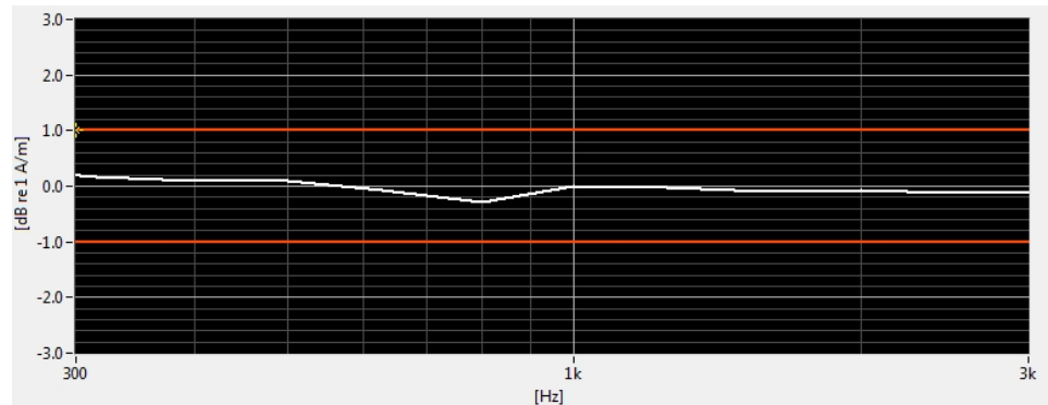
Figure 6-3 Helmholtz Coil Validation for Frequency Response
