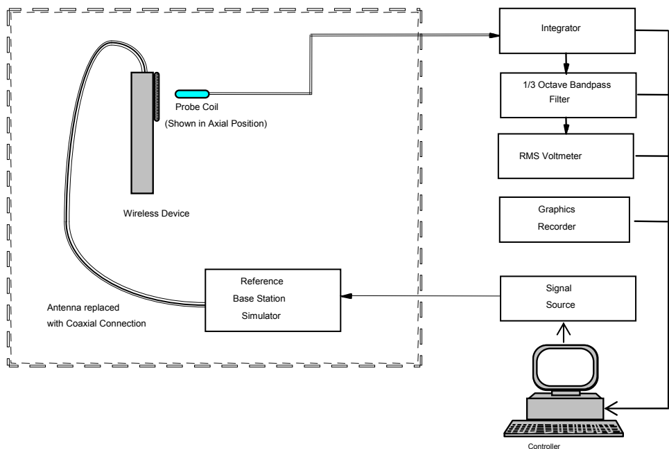
Figure 4-12 Audio Magnetic Field Test Setup
