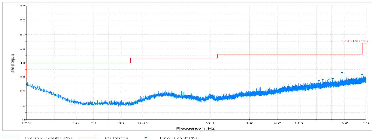
Plot 6-44. Radiated Spurious Plot below 1GHz (Pol. V)
