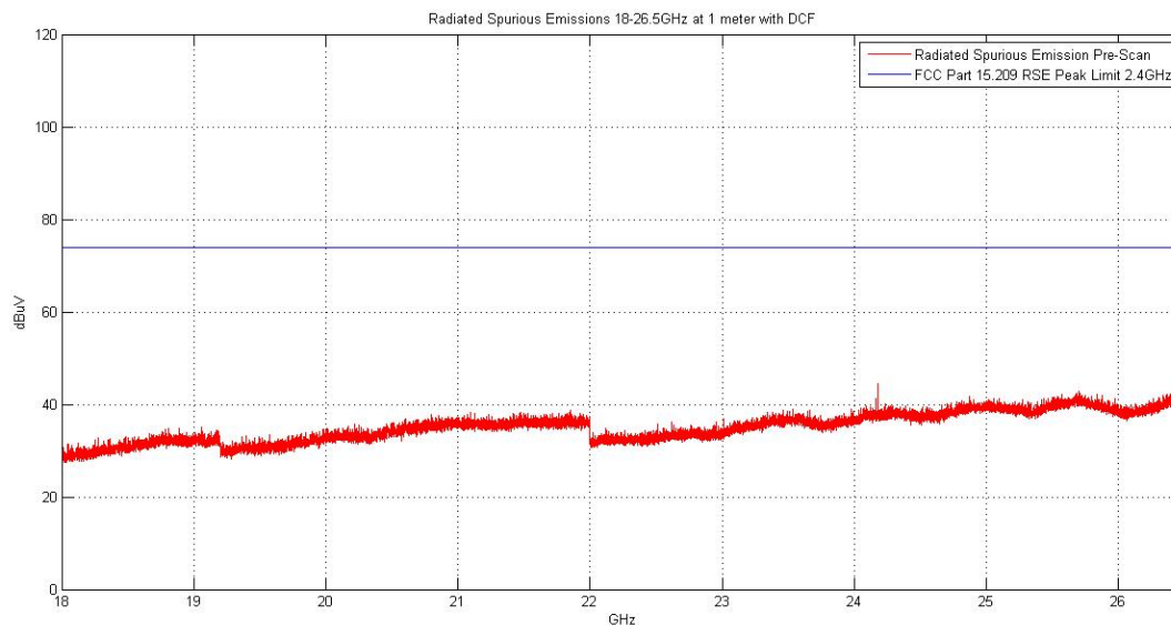
Plot 6-25. Radiated Spurious Plot above 18GHz (Pol. V)
