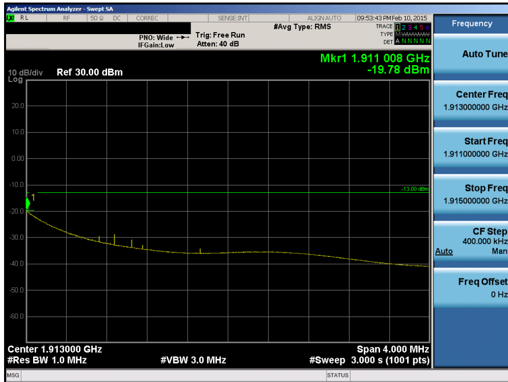
Plot 6-26. 4MHz Span Plot (PCS CDMA Mode – Ch. 1175)
