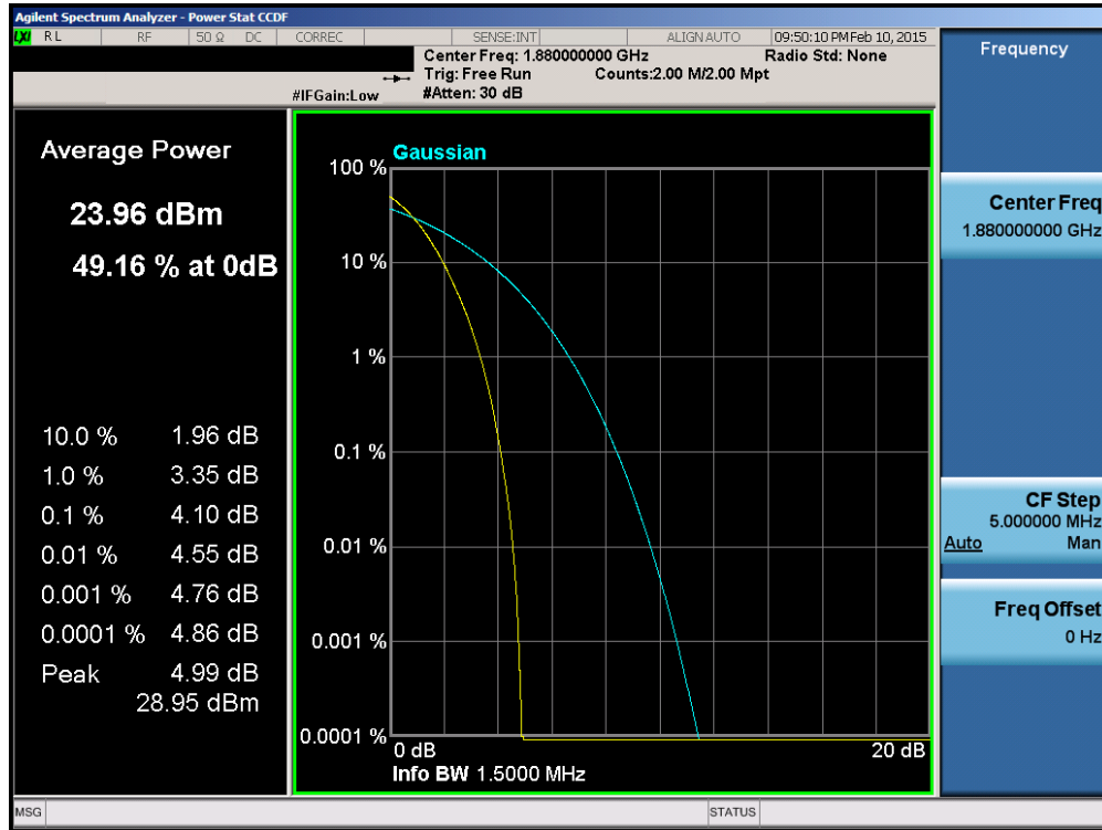
Plot 6-27. Peak-Average Ratio Plot (PCS CDMA Mode – Ch. 600)
