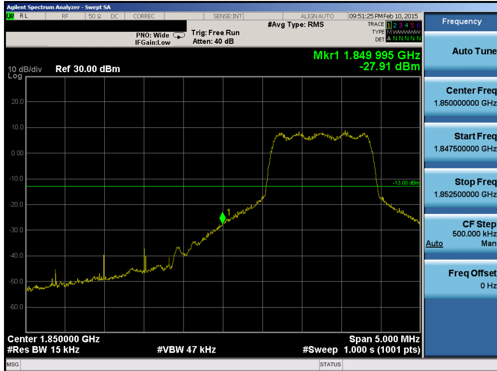
Plot 6-23. Band Edge Plot (PCS CDMA Mode – Ch. 25)
