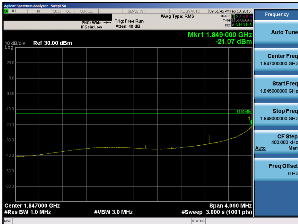
Plot 6-24. 4MHz Span Plot (PCS CDMA Mode – Ch. 25)
