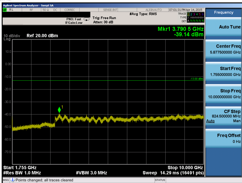
Plot 6-63. Conducted Spurious Plot (Band 4 – 20.0MHz QPSK – RB Size 1, RB Offset 0 – Mid Channel)
