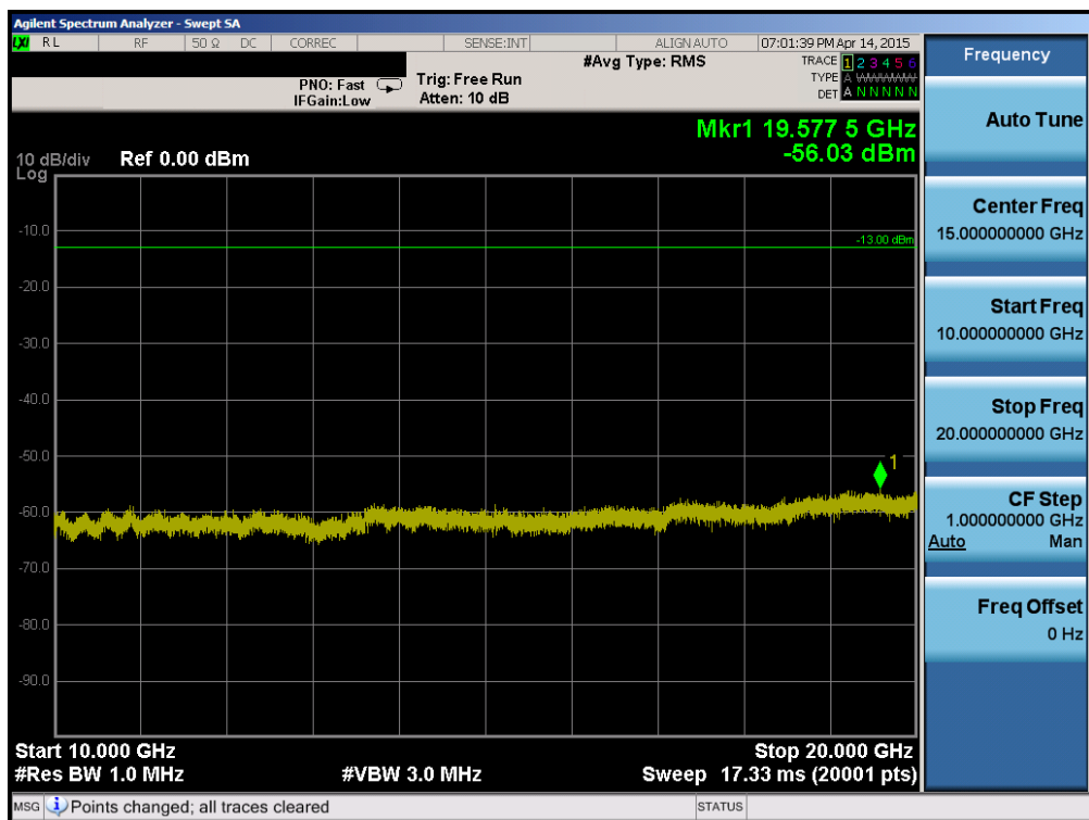
Plot 6-64. Conducted Spurious Plot (Band 4 – 20.0MHz QPSK – RB Size 1, RB Offset 0 – Mid Channel)
