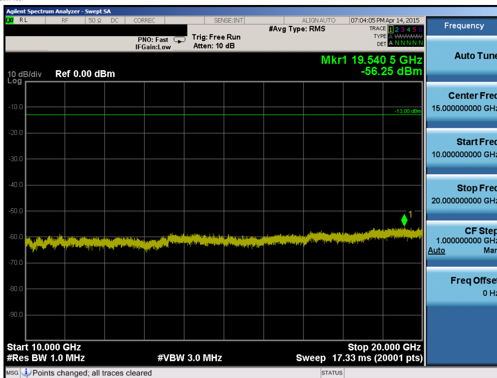
Plot 6-61. Conducted Spurious Plot (Band 4 – 20.0MHz QPSK – RB Size 1, RB Offset 0 – Low Channel)
