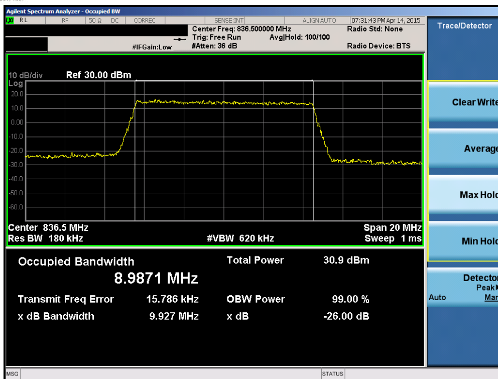
Plot 6-15. Occupied Bandwidth Plot (Band 5 – 10.0MHz QPSK – RB Size 50)
