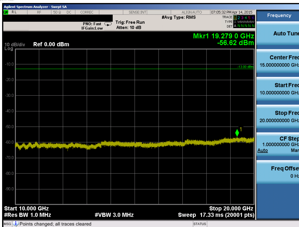
Plot 6-67. Conducted Spurious Plot (Band 4 – 20.0MHz QPSK – RB Size 1, RB Offset 0 – High Channel)
