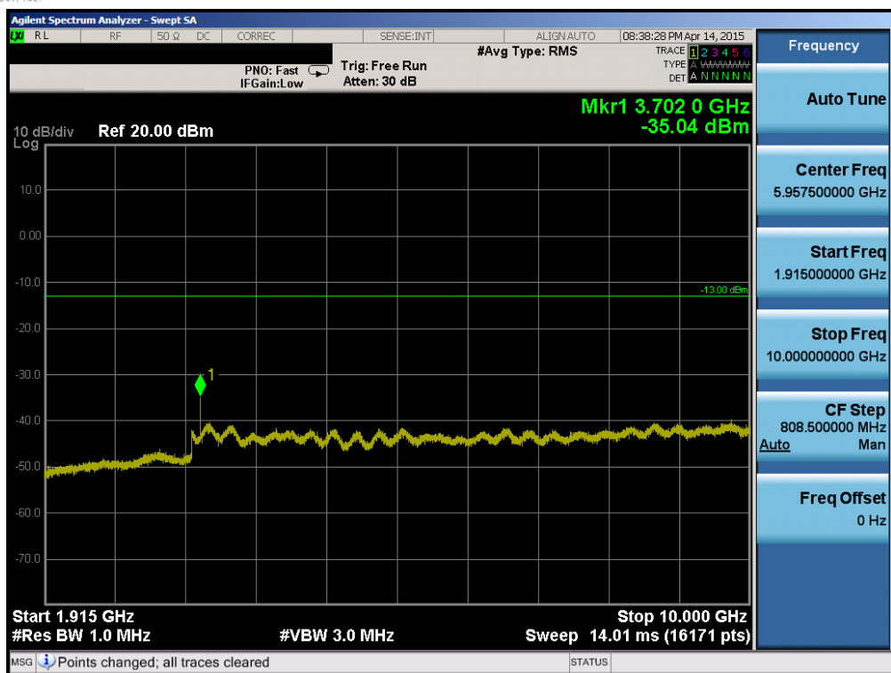
Plot 6-69. Conducted Spurious Plot (Band 25 – 10.0MHz QPSK – RB Size 1, RB Offset 0 – Low Channel)
