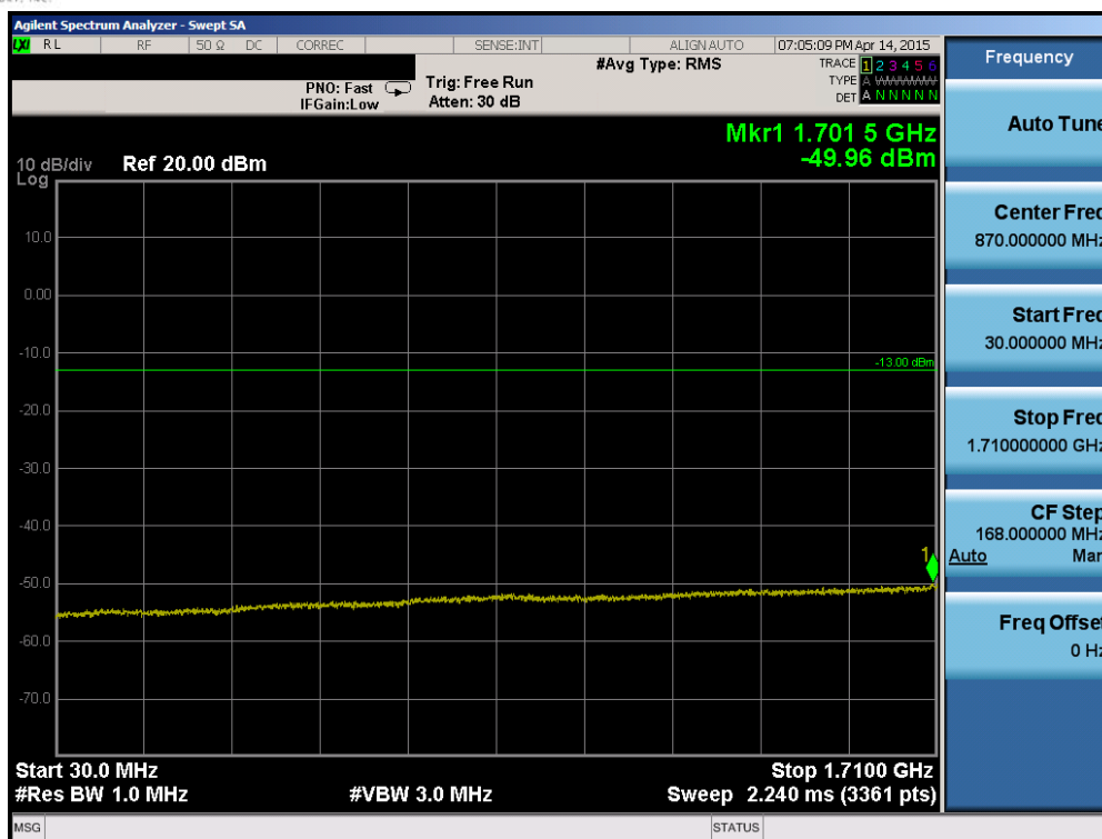
Plot 6-65. Conducted Spurious Plot (Band 4 – 20.0MHz QPSK – RB Size 1, RB Offset 0 – High Channel)
