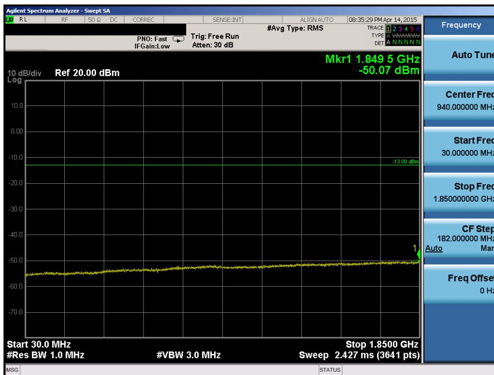
Plot 6-74. Conducted Spurious Plot (Band 25 – 10.0MHz QPSK – RB Size 1, RB Offset 0 – High Channel)
