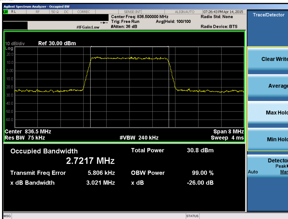
Plot 6-11. Occupied Bandwidth Plot (Band 5 - 3.0MHz QPSK - RB Size 15)
