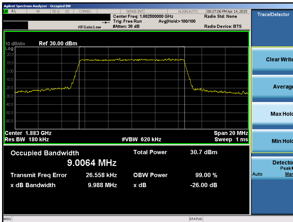
Plot 6-35. Occupied Bandwidth Plot (Band 25 – 10.0MHz QPSK – RB Size 50)
