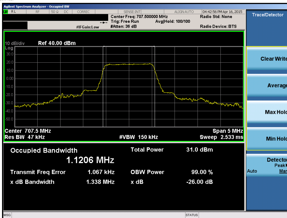
Plot 6-1. Occupied Bandwidth Plot (Band 12 – 1.4MHz QPSK – RB Size 6)
