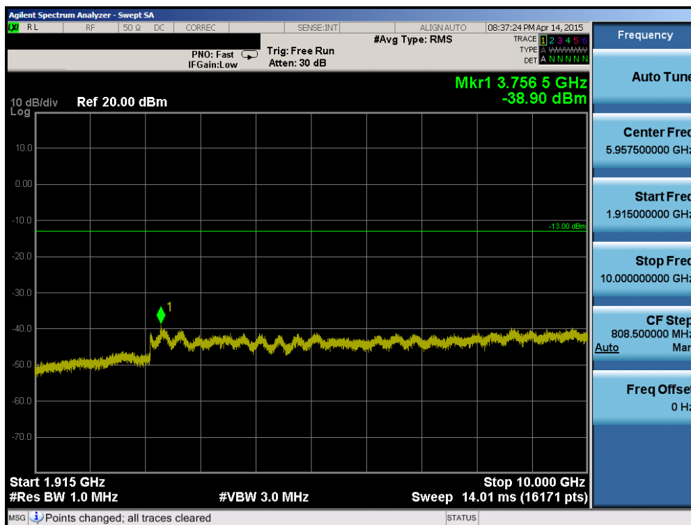
Plot 6-72. Conducted Spurious Plot (Band 25 – 10.0MHz QPSK – RB Size 1, RB Offset 0 – Mid Channel)
