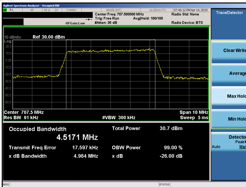
Plot 6-5. Occupied Bandwidth Plot (Band 12 – 5.0MHz QPSK – RB Size 25)
