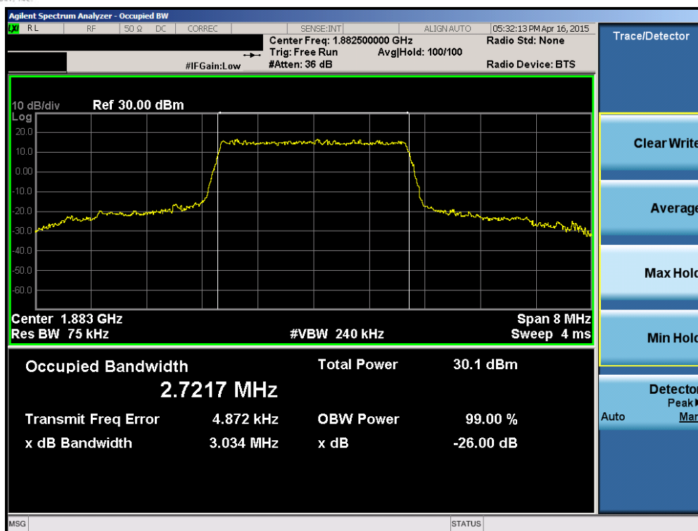
Plot 6-31. Occupied Bandwidth Plot (Band 25 – 3.0MHz QPSK – RB Size 15)
