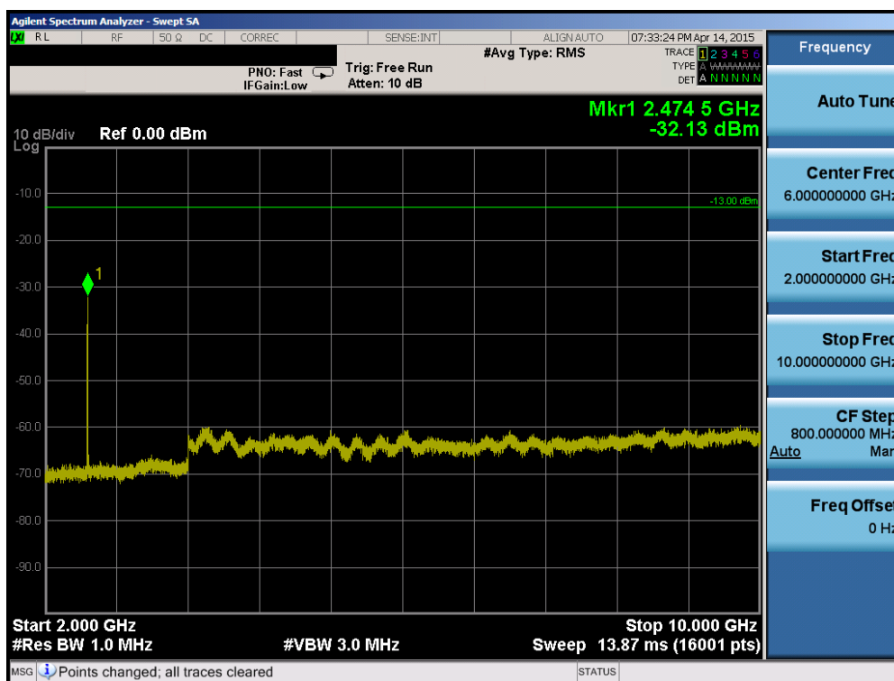
Plot 6-52. Conducted Spurious Plot (Band 5 – 10.0MHz QPSK – RB Size 1, RB Offset 0 – Low Channel)
