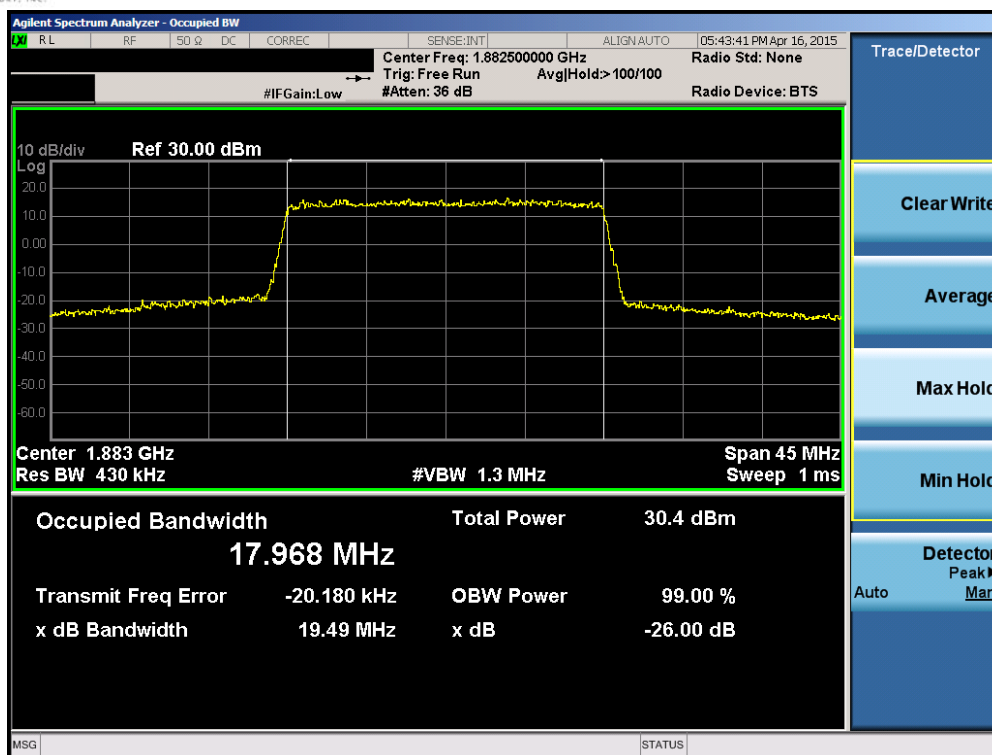
Plot 6-39. Occupied Bandwidth Plot (Band 25 – 20.0MHz QPSK – RB Size 100)
