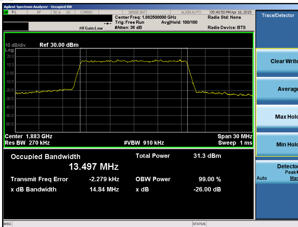
Plot 6-37. Occupied Bandwidth Plot (Band 25 – 15.0MHz QPSK – RB Size 75)
