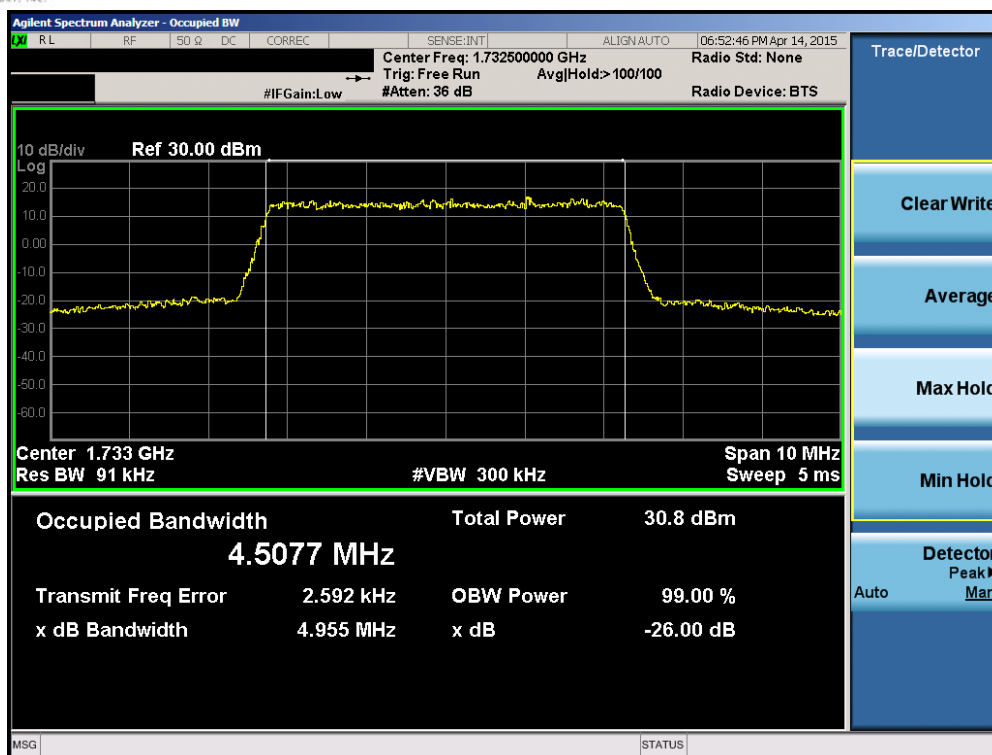
Plot 6-21. Occupied Bandwidth Plot (Band 4 – 5.0MHz QPSK – RB Size 25)
