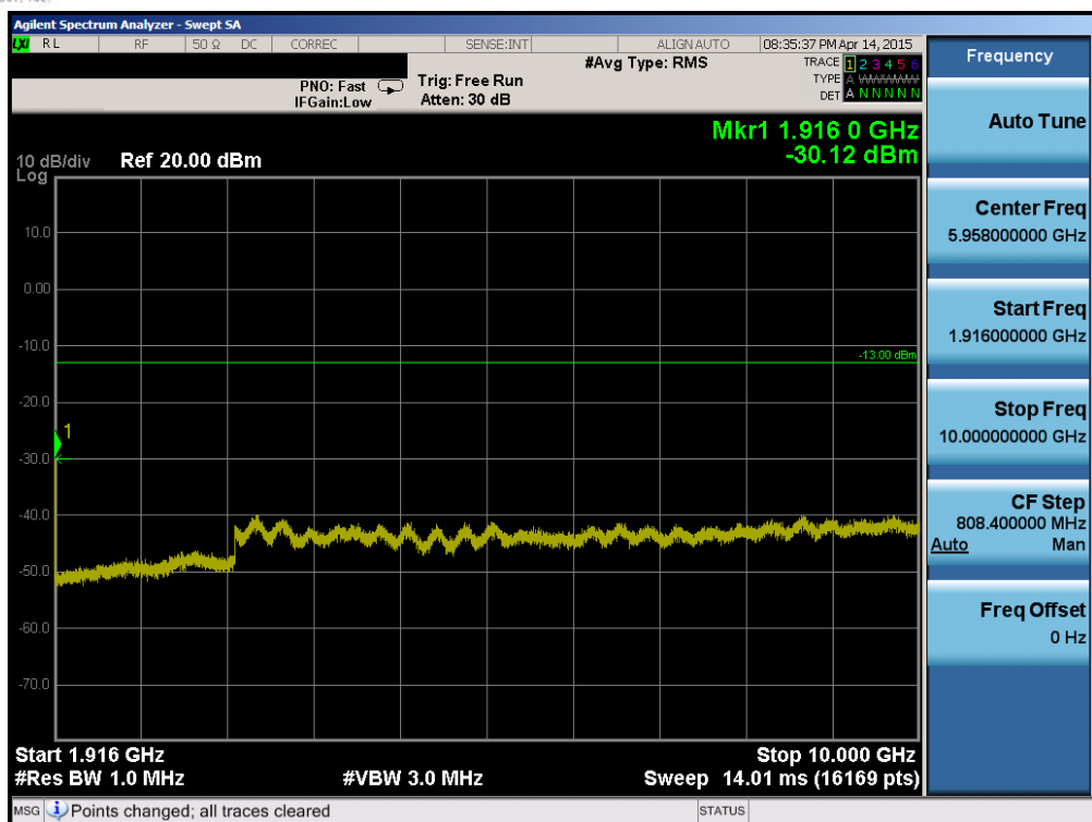
Plot 6-75. Conducted Spurious Plot (Band 25 – 10.0MHz QPSK – RB Size 1, RB Offset 0 – High Channel)
