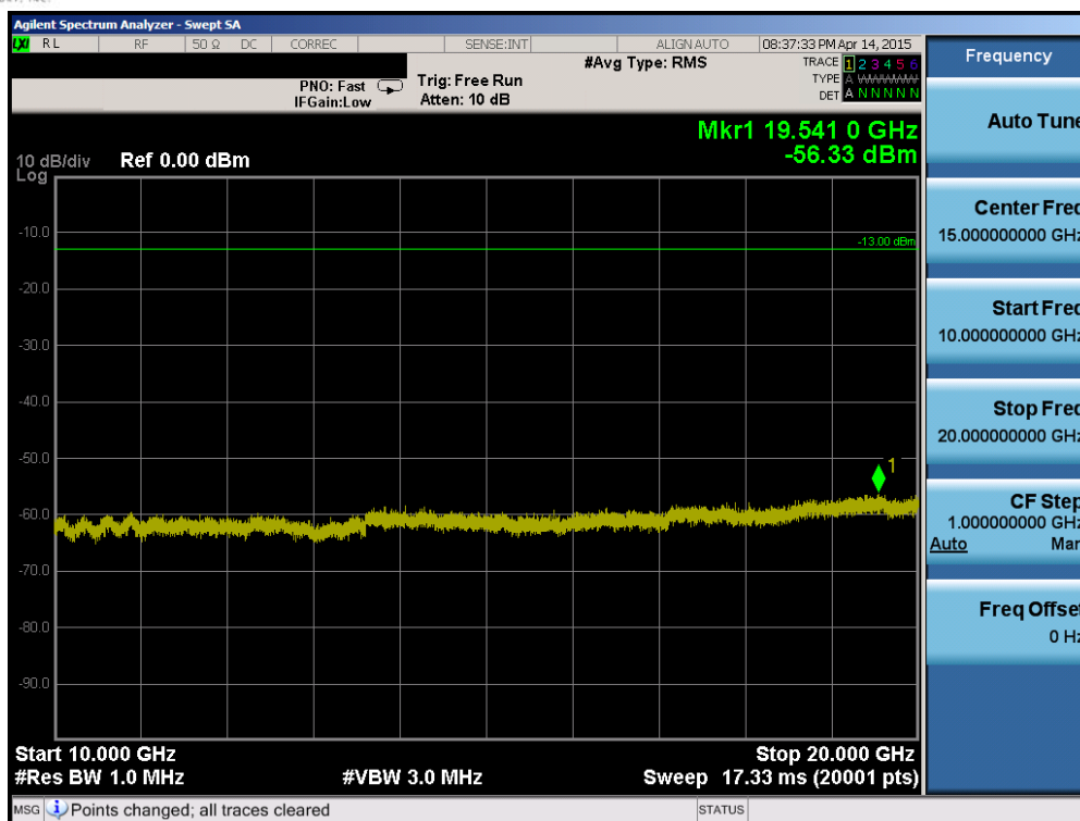
Plot 6-73. Conducted Spurious Plot (Band 25 – 10.0MHz QPSK – RB Size 1, RB Offset 0 – Mid Channel)
