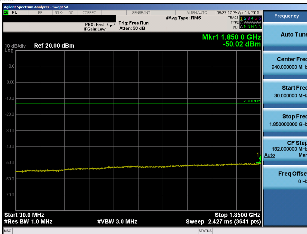
Plot 6-71. Conducted Spurious Plot (Band 25 – 10.0MHz QPSK – RB Size 1, RB Offset 0 – Mid Channel)
