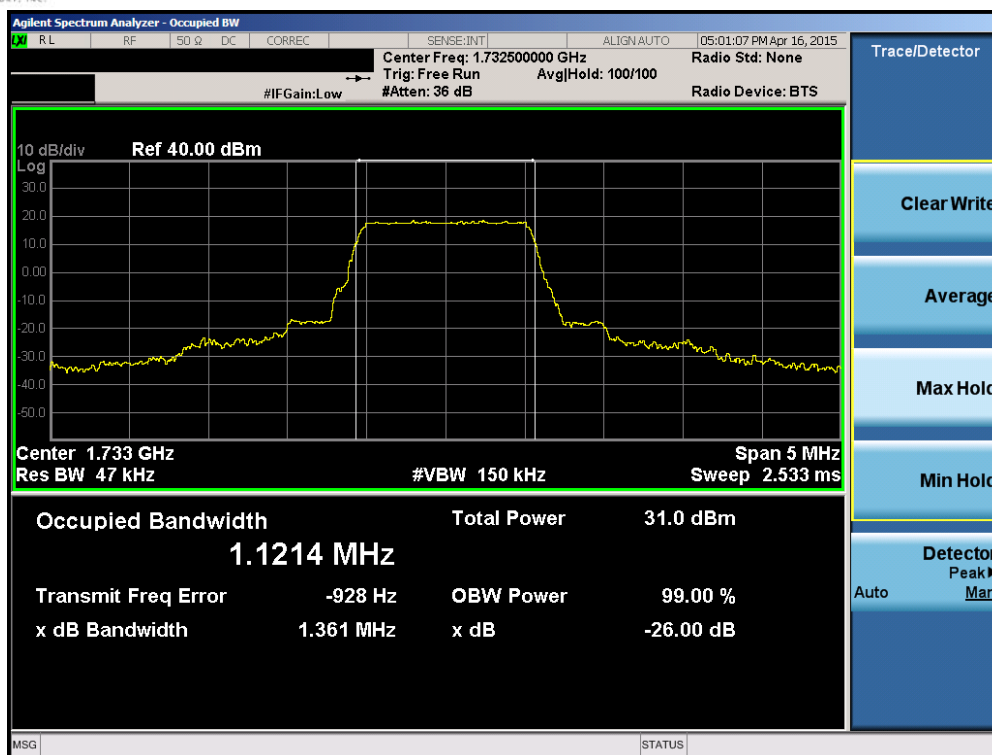
Plot 6-17. Occupied Bandwidth Plot (Band 4 – 1.4MHz QPSK – RB Size 6)
