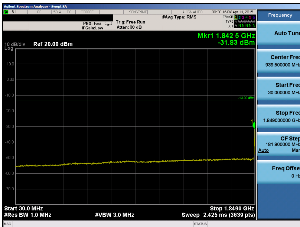
Plot 6-68. Conducted Spurious Plot (Band 25 – 10.0MHz QPSK – RB Size 1, RB Offset 0– Low Channel)
