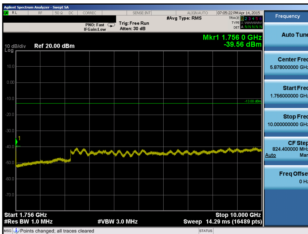
Plot 6-66. Conducted Spurious Plot (Band 4 – 20.0MHz QPSK – RB Size 1, RB Offset 0 – High Channel)
