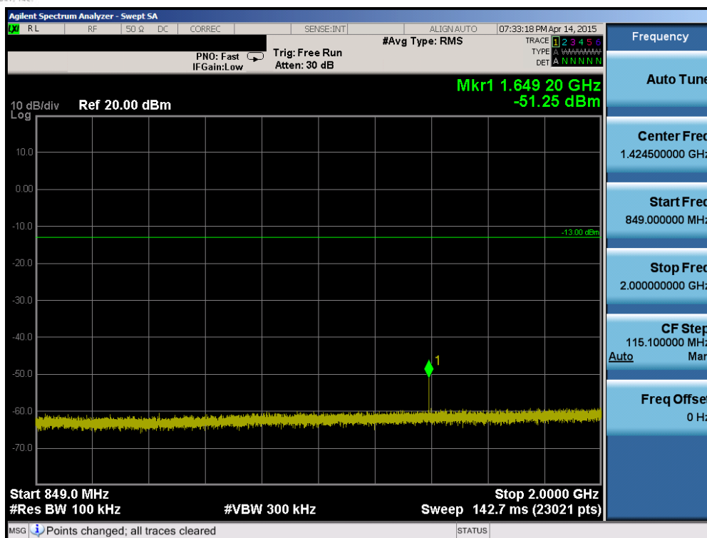
Plot 6-51. Conducted Spurious Plot (Band 5 – 10.0MHz QPSK – RB Size 1, RB Offset 0 – Low Channel)
