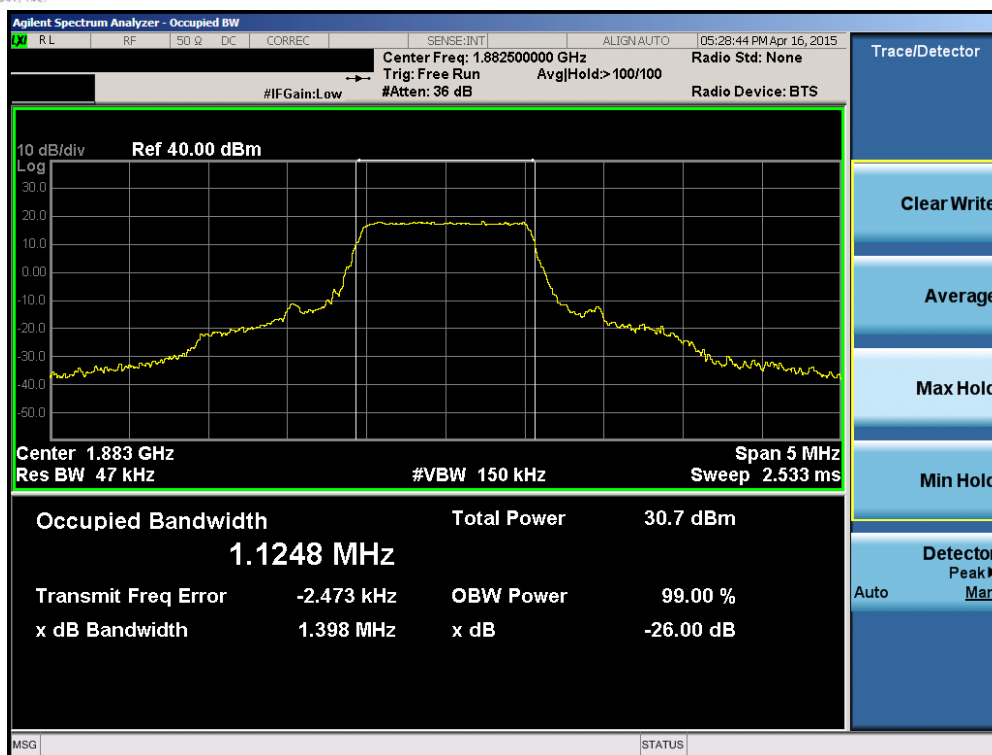
Plot 6-29. Occupied Bandwidth Plot (Band 25 – 1.4MHz QPSK – RB Size 6)
