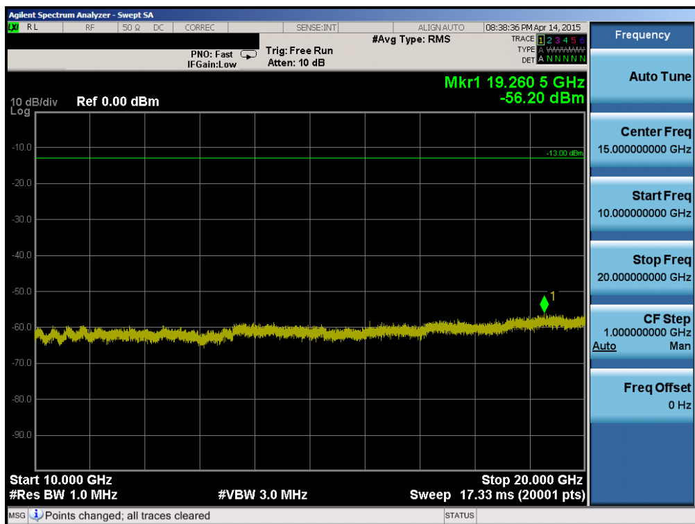
Plot 6-70. Conducted Spurious Plot (Band 25 – 10.0MHz QPSK – RB Size 1, RB Offset 0 – Low Channel)
