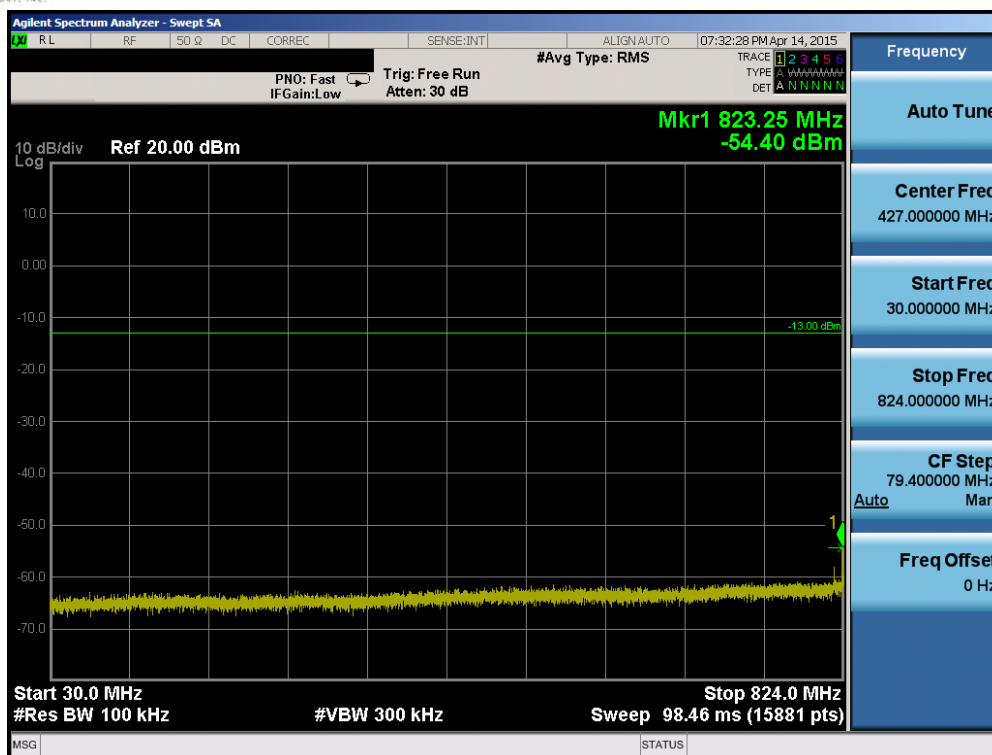
Plot 6-53. Conducted Spurious Plot (Band 5 – 10.0MHz QPSK – RB Size 1, RB Offset 0 – Mid Channel)
