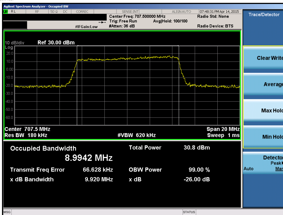
Plot 6-7. Occupied Bandwidth Plot (Band 12 – 10.0MHz QPSK – RB Size 50)
