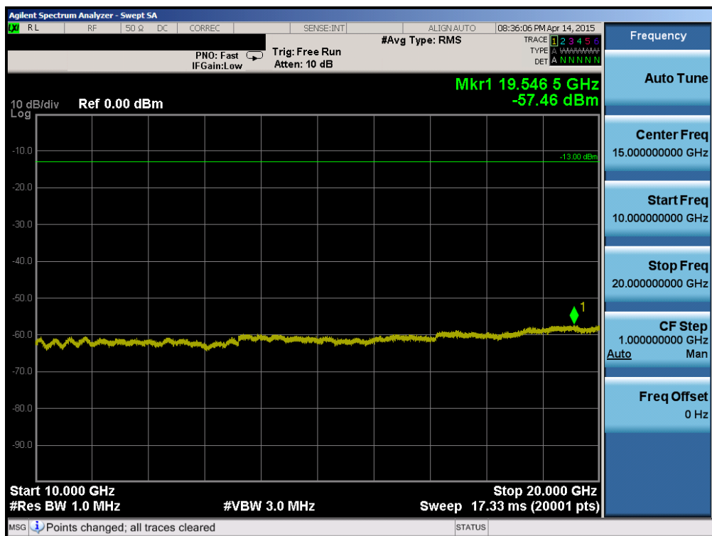
Plot 6-76. Conducted Spurious Plot (Band 25 – 10.0MHz QPSK – RB Size 1, RB Offset 0 – High Channel)
