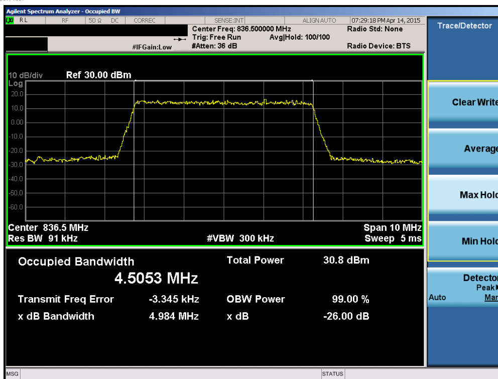
Plot 6-13. Occupied Bandwidth Plot (Band 5 – 5.0MHz QPSK – RB Size 25)
