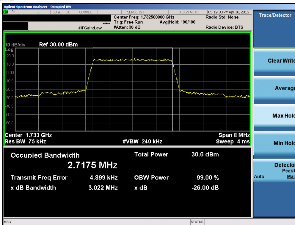
Plot 6-19. Occupied Bandwidth Plot (Band 4 – 3.0MHz QPSK – RB Size 15)
