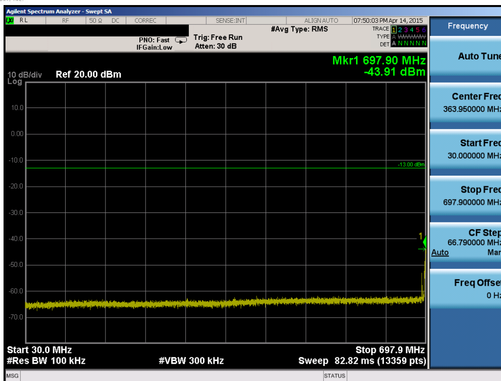
Plot 6-41. Conducted Spurious Plot (Band 12 – 10.0MHz QPSK – RB Size 1, RB Offset 0– Low Channel)
