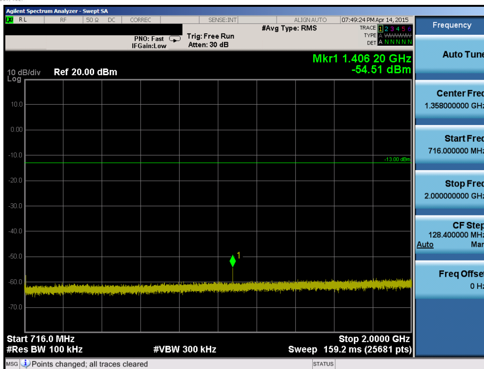
Plot 6-45. Conducted Spurious Plot (Band 12 – 10.0MHz QPSK – RB Size 1, RB Offset 0 – Mid Channel)
