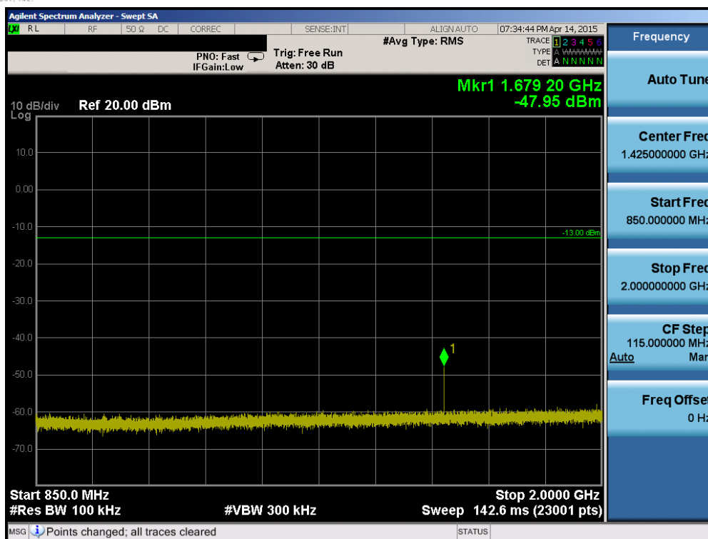
Plot 6-57. Conducted Spurious Plot (Band 5 – 10.0MHz QPSK – RB Size 1, RB Offset 0 – High Channel)
