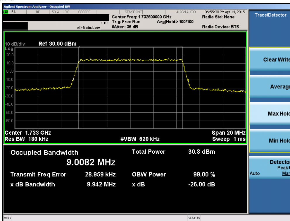
Plot 6-23. Occupied Bandwidth Plot (Band 4 – 10.0MHz QPSK – RB Size 50)
