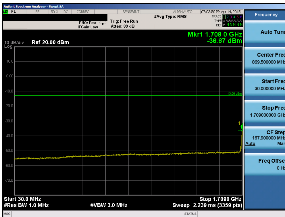
Plot 6-59. Conducted Spurious Plot (Band 4 – 20.0MHz QPSK – RB Size 1, RB Offset 0– Low Channel)
