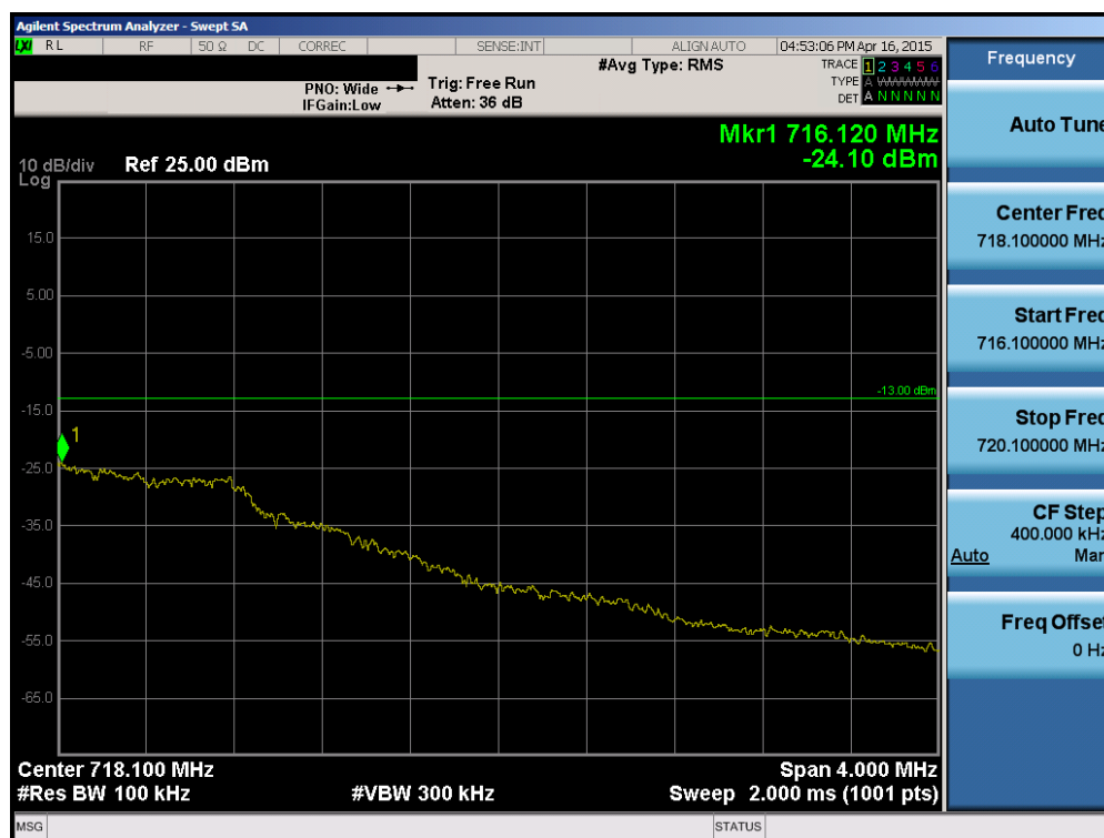
Plot 6-80. Upper Extended Band Edge Plot (Band 12 – 1.4MHz QPSK – RB Size 6)
