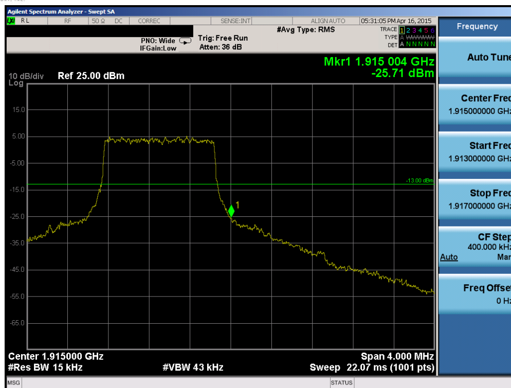
Plot 6-131. Upper Band Edge Plot (Band 25 – 1.4MHz QPSK – RB Size 6)
