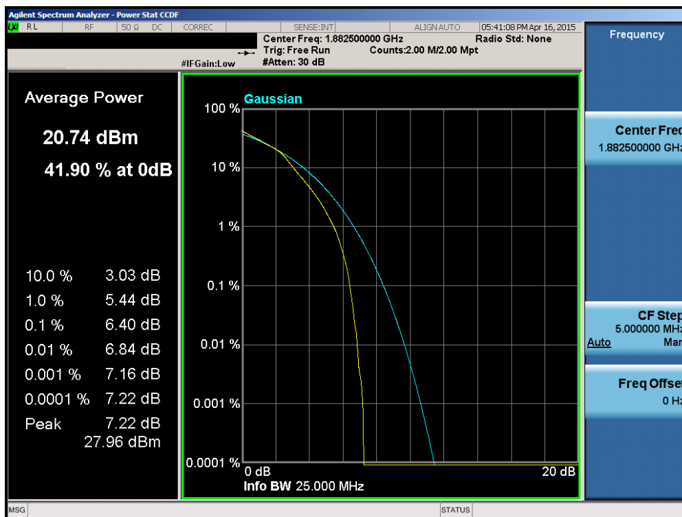
Plot 6-162. PAR Plot (Band 25 – 15.0MHz 16-QAM – RB Size 75)
