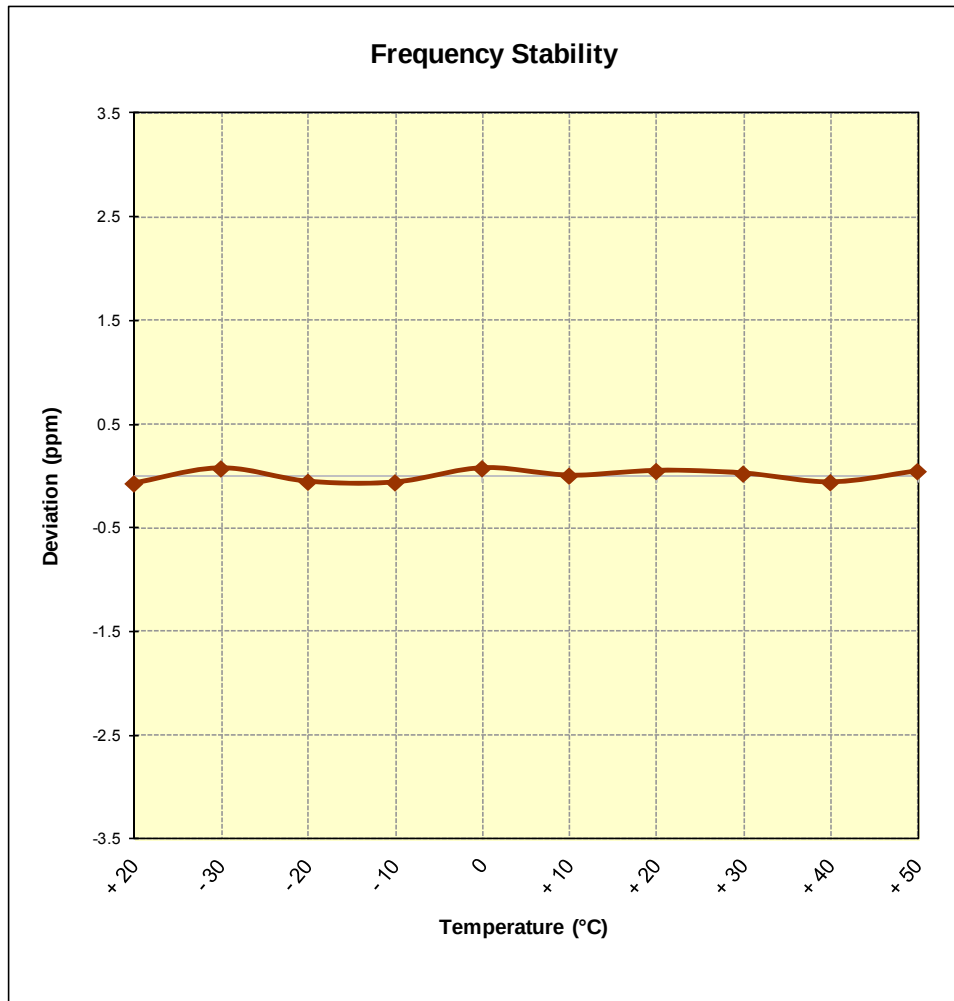
Figure 6-10. Frequency Stability Graph (Band 25)
