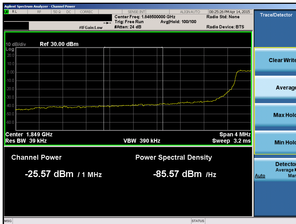
Plot 6-138. Lower Extended Band Edge Plot (Band 25 – 5.0MHz QPSK – RB Size 25)
