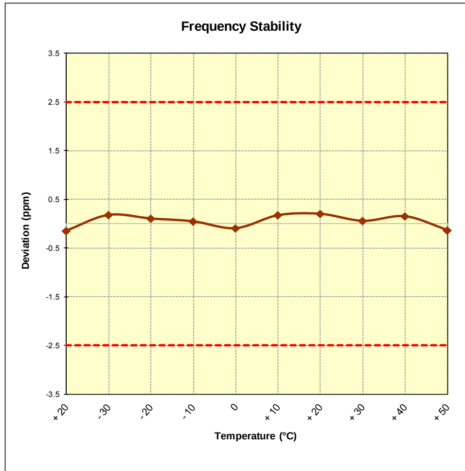
Figure 6-7. Frequency Stability Graph (Band 12)
