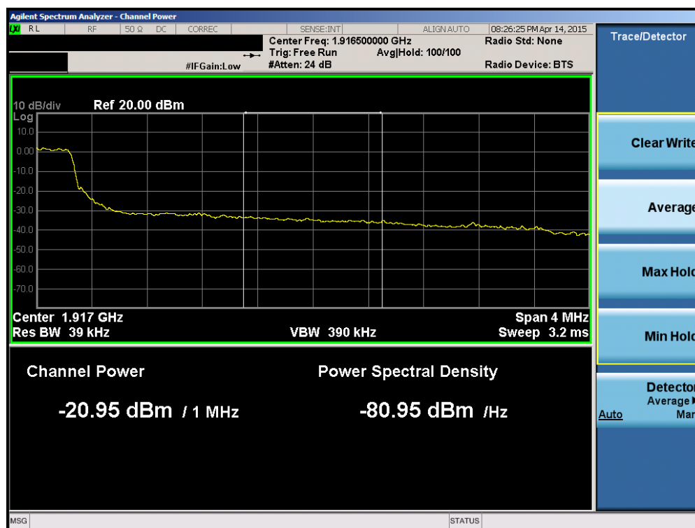
Plot 6-140. Upper Extended Band Edge Plot (Band 25 – 5.0MHz QPSK – RB Size 25)
