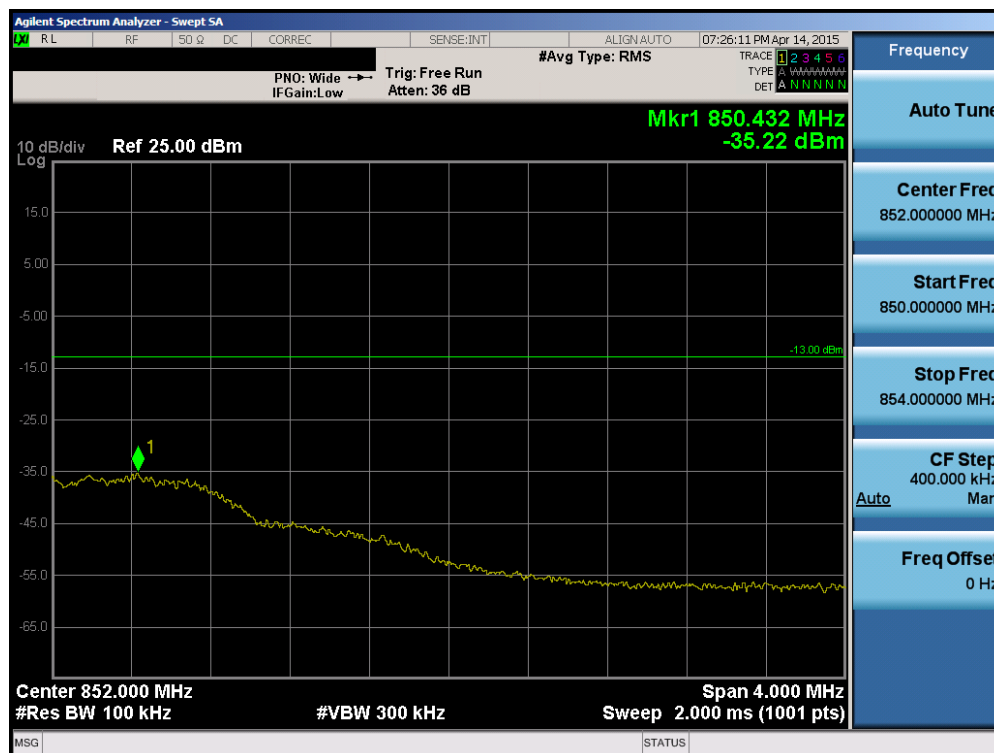
Plot 6-94. Upper Extended Band Edge Plot (Band 5 – 1.4MHz QPSK – RB Size 6)
