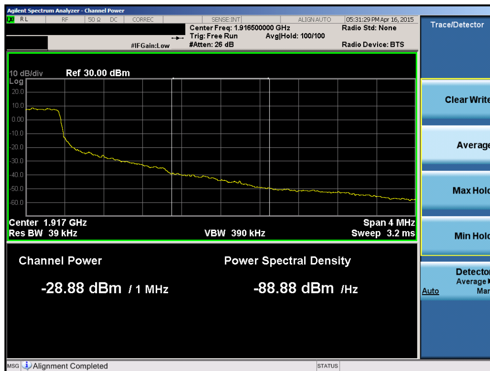
Plot 6-132. Upper Extended Band Edge Plot (Band 25 – 1.4MHz QPSK – RB Size 6)
