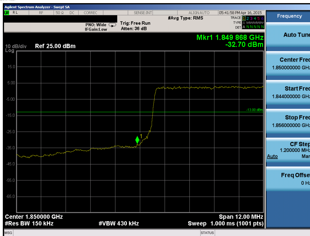
Plot 6-145. Lower Band Edge Plot (Band 25 – 15.0MHz QPSK – RB Size 75)
