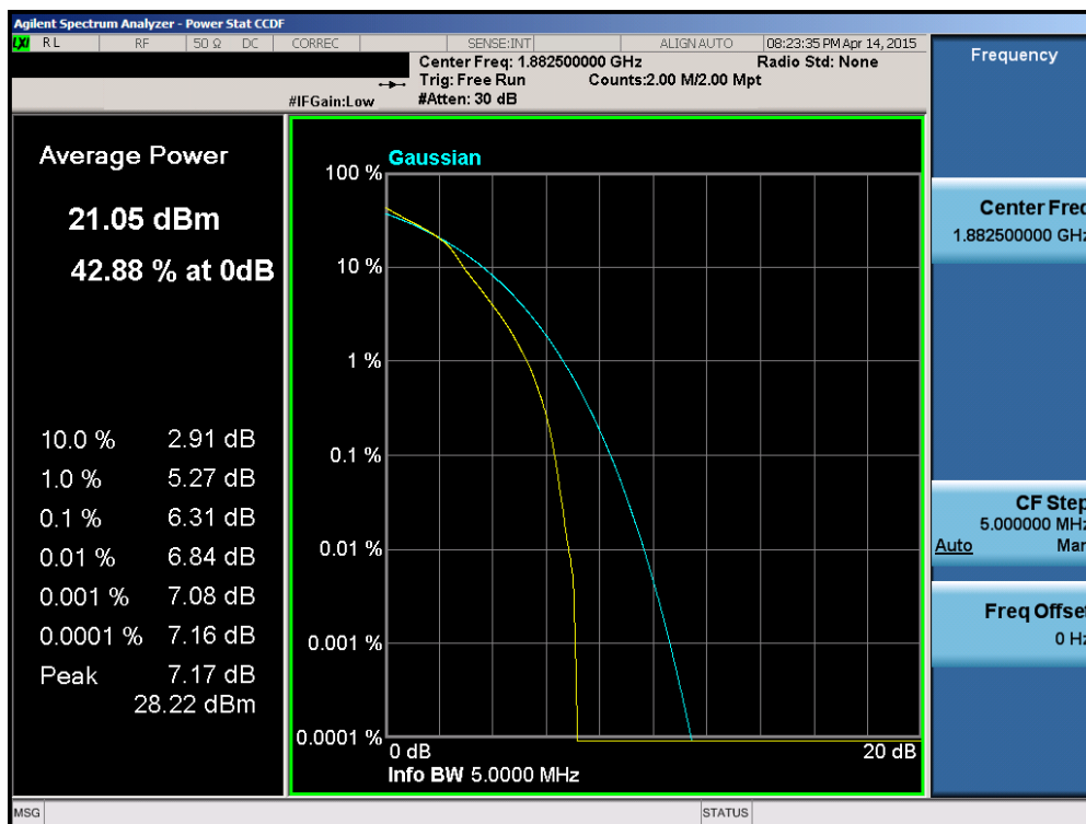
Plot 6-158. PAR Plot (Band 25 – 5.0MHz 16-QAM – RB Size 25)
