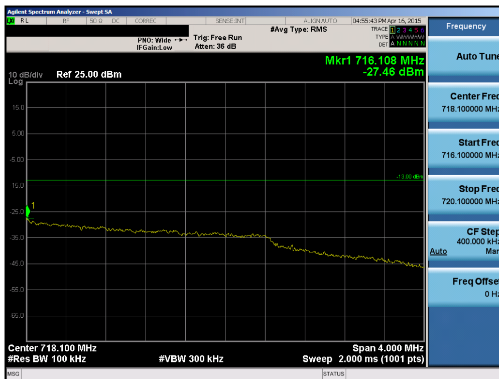
Plot 6-84. Upper Extended Band Edge Plot (Band 12 – 3.0MHz QPSK – RB Size 15)
