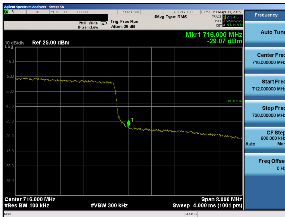
Plot 6-90. Upper Band Edge Plot (Band 12 – 10.0MHz QPSK – RB Size 50)
