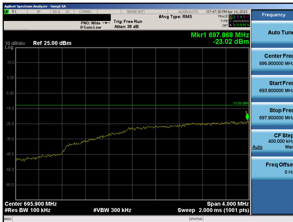
Plot 6-86. Lower Extended Band Edge Plot (Band 12 – 5.0MHz QPSK – RB Size 25)
