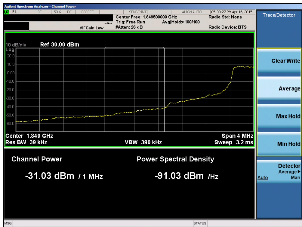
Plot 6-130. Lower Extended Band Edge Plot (Band 25 – 1.4MHz QPSK – RB Size 6)
