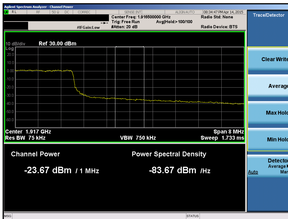
Plot 6-144. Upper Extended Band Edge Plot (Band 25 – 10.0MHz QPSK – RB Size 50)
