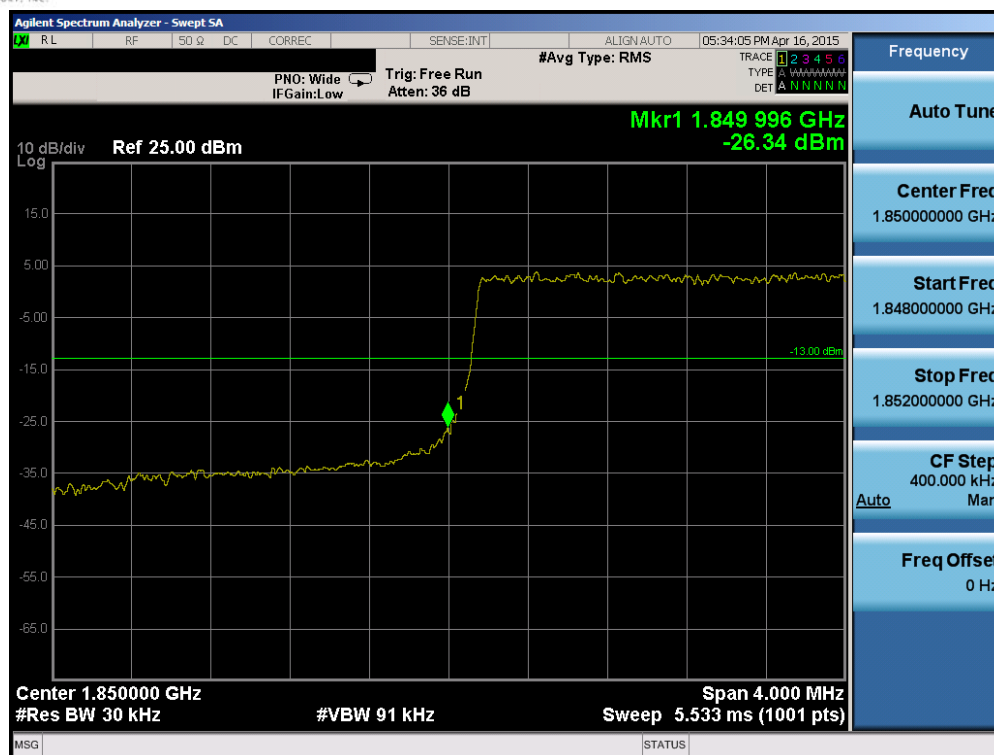
Plot 6-133. Lower Band Edge Plot (Band 25 – 3.0MHz QPSK – RB Size 15)
