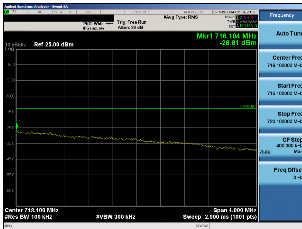
Plot 6-88. Upper Extended Band Edge Plot (Band 12 – 5.0MHz QPSK – RB Size 25)
