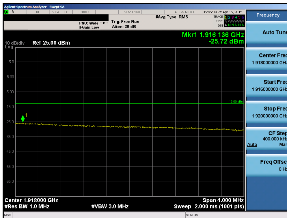
Plot 6-152. Upper Extended Band Edge Plot (Band 25 – 20.0MHz QPSK – RB Size 100)
