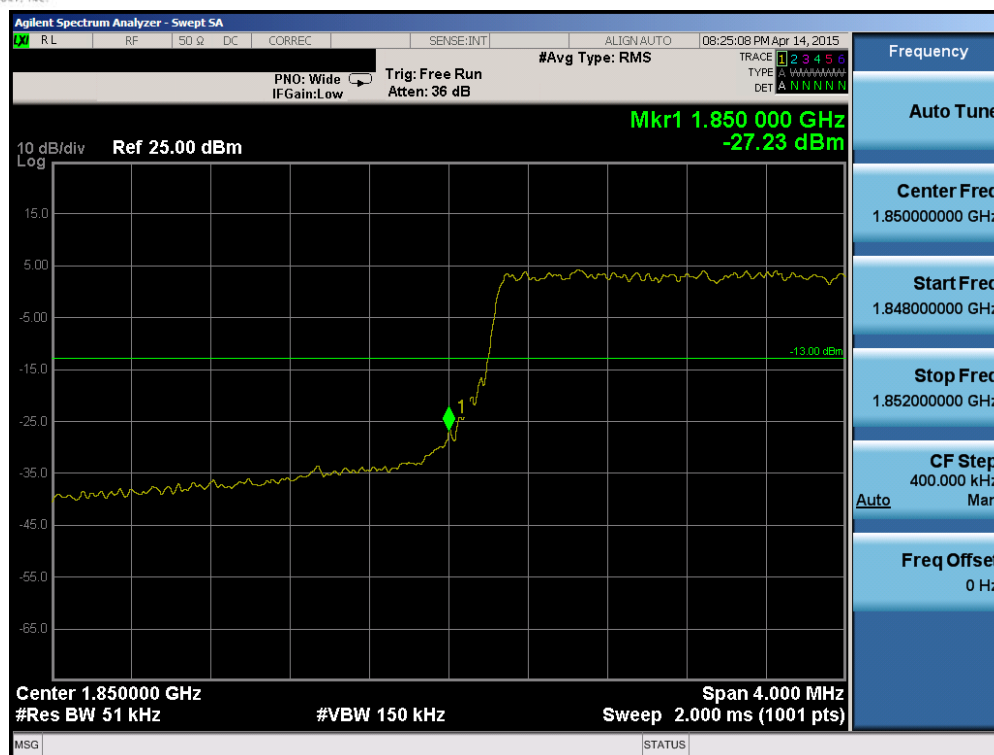
Plot 6-137. Lower Band Edge Plot (Band 25 – 5.0MHz QPSK – RB Size 25)
