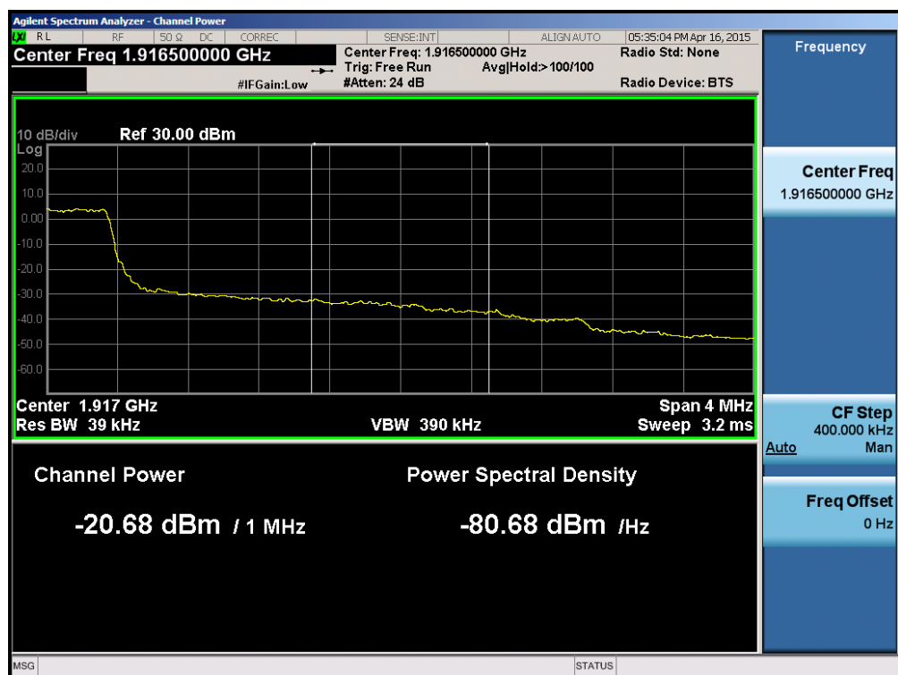
Plot 6-136. Upper Extended Band Edge Plot (Band 25 – 3.0MHz QPSK – RB Size 15)
