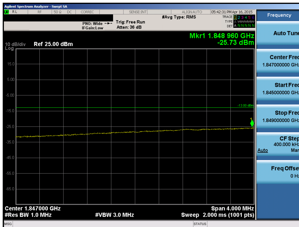
Plot 6-146. Lower Extended Band Edge Plot (Band 25 – 15.0MHz QPSK – RB Size 75)
