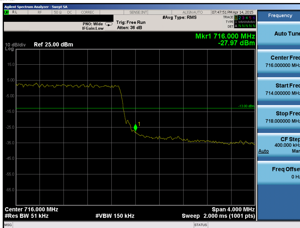
Plot 6-87. Upper Band Edge Plot (Band 12 – 5.0MHz QPSK – RB Size 25)
