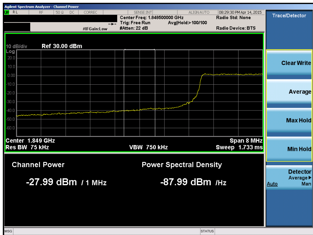
Plot 6-142. Lower Extended Band Edge Plot (Band 25 – 10.0MHz QPSK – RB Size 50)
