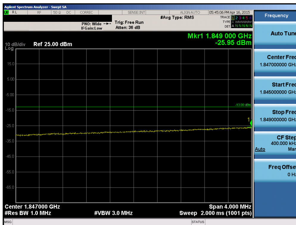
Plot 6-150. Lower Extended Band Edge Plot (Band 25 – 20.0MHz QPSK – RB Size 100)
