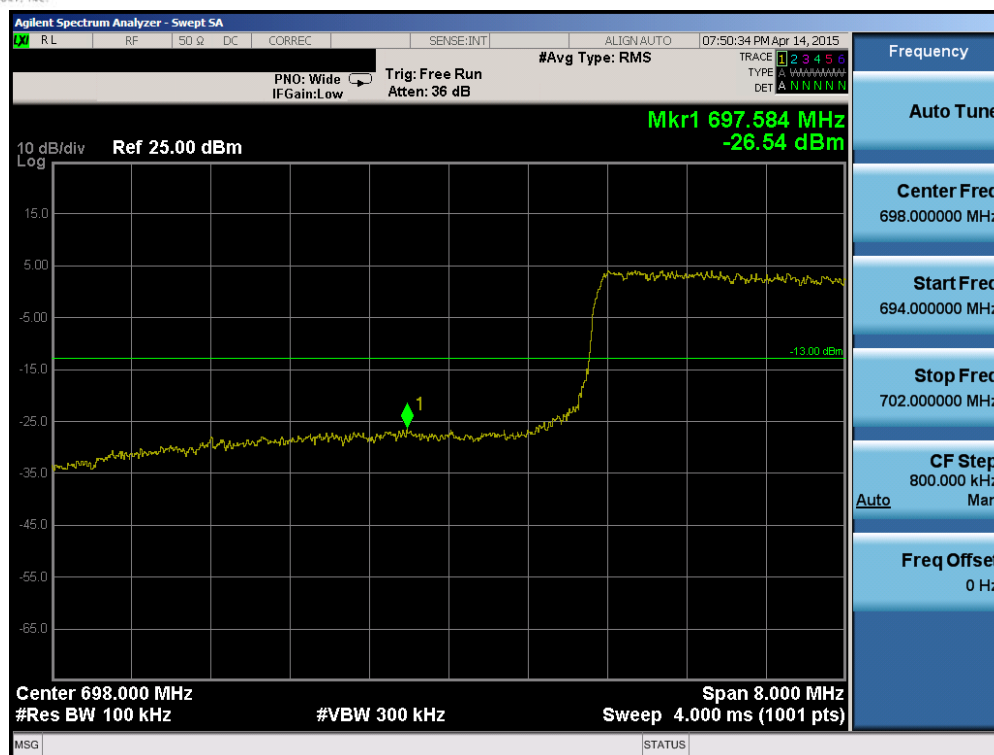
Plot 6-89. Lower Band Edge Plot (Band 12 – 10.0MHz QPSK – RB Size 50)
