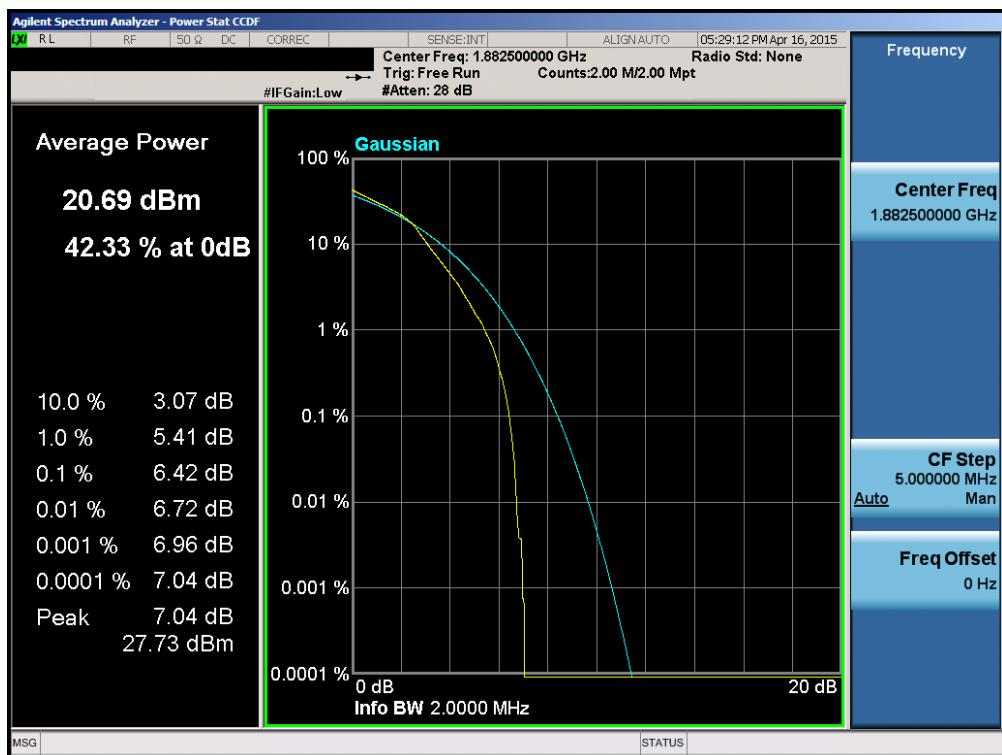
Plot 6-154. PAR Plot (Band 25 – 1.4MHz 16-QAM – RB Size 6)
