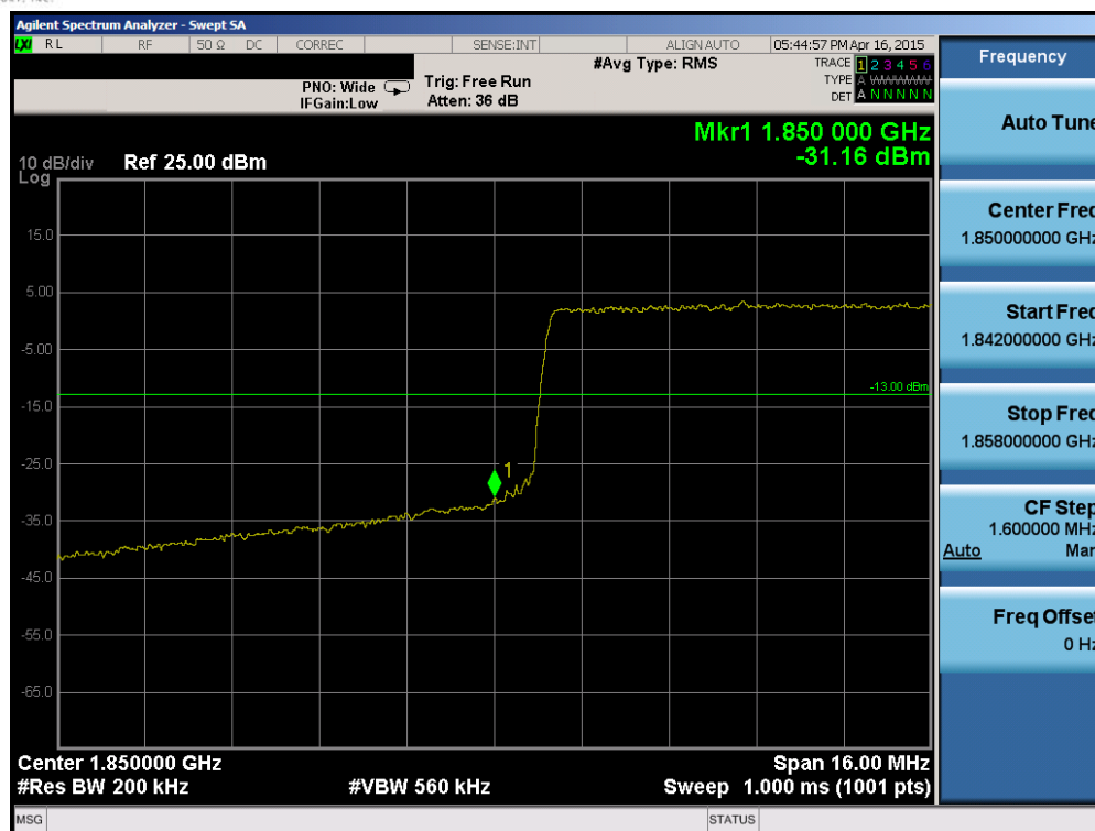
Plot 6-149. Lower Band Edge Plot (Band 25 – 20.0MHz QPSK – RB Size 100)
