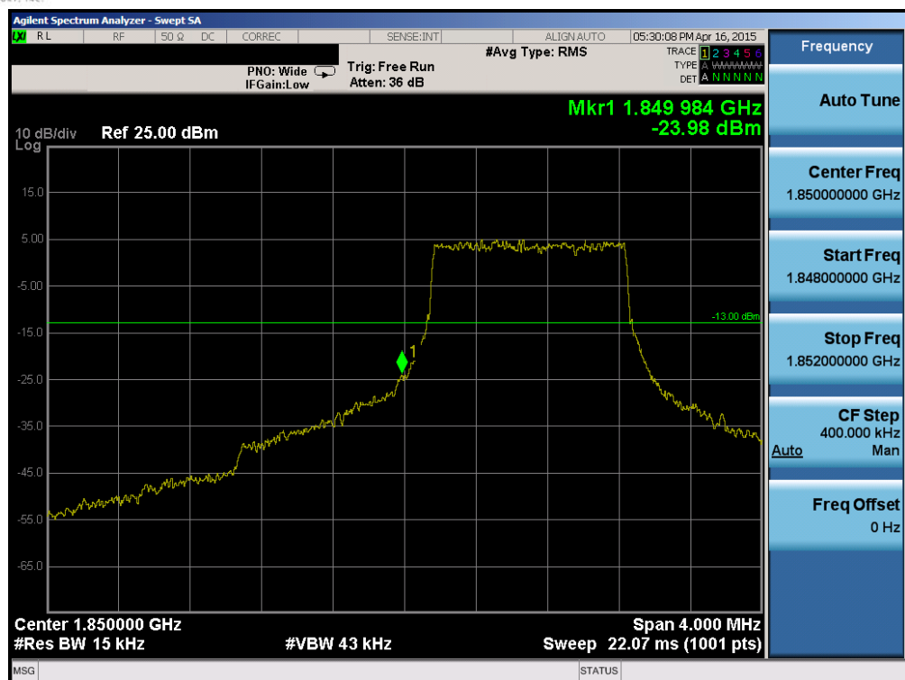
Plot 6-129. Lower Band Edge Plot (Band 25 – 1.4MHz QPSK – RB Size 6)
