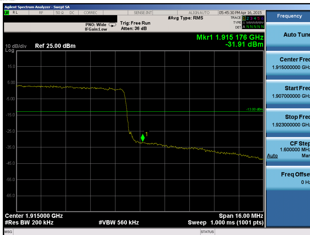
Plot 6-151. Upper Band Edge Plot (Band 25 – 20.0MHz QPSK – RB Size 100)
