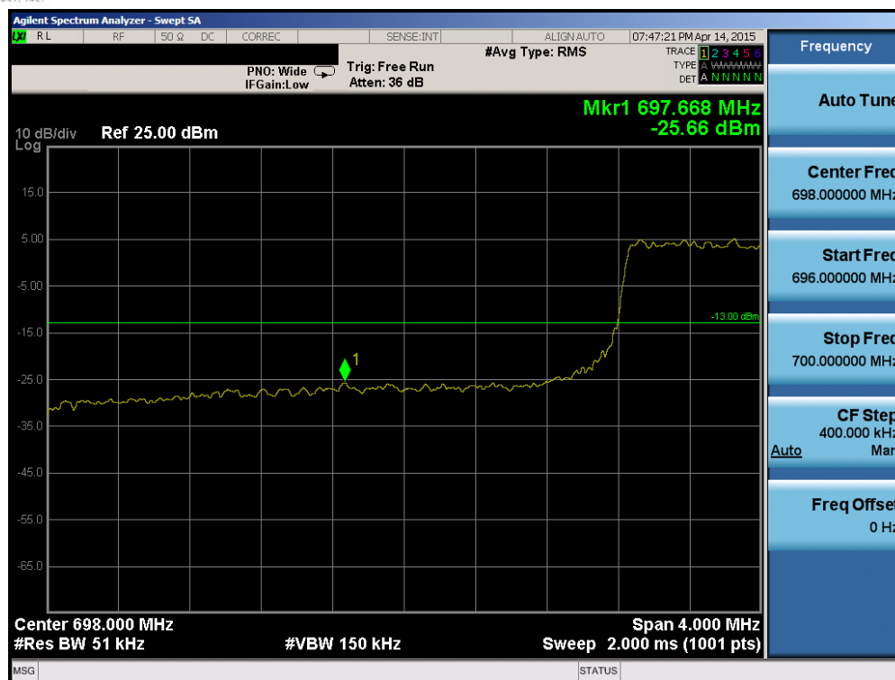
Plot 6-85. Lower Band Edge Plot (Band 12 – 5.0MHz QPSK – RB Size 25)
