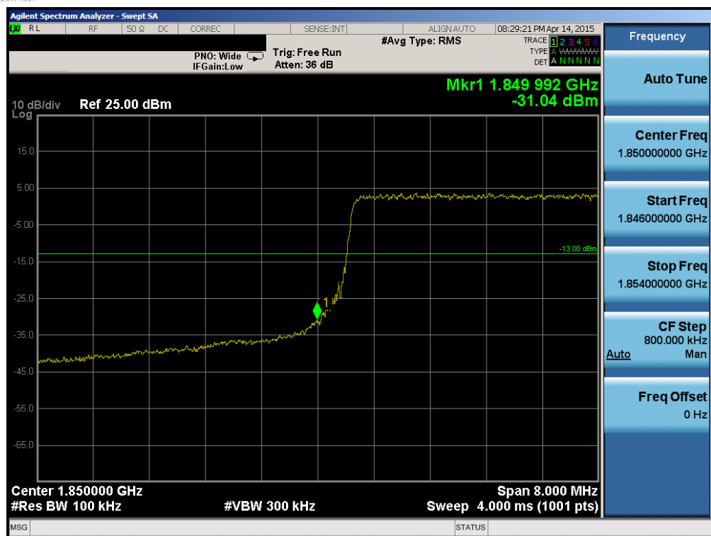
Plot 6-141. Lower Band Edge Plot (Band 25 – 10.0MHz QPSK – RB Size 50)
