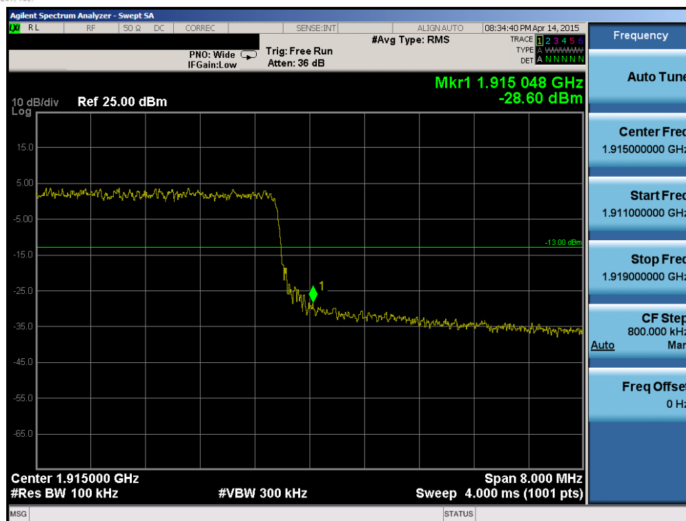
Plot 6-143. Upper Band Edge Plot (Band 25 – 10.0MHz QPSK – RB Size 50)
