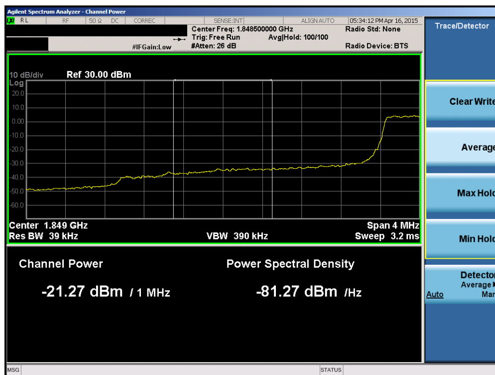
Plot 6-134. Lower Extended Band Edge Plot (Band 25 – 3.0MHz QPSK – RB Size 15)
