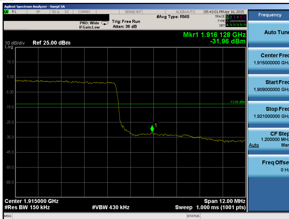
Plot 6-147. Upper Band Edge Plot (Band 25 – 15.0MHz QPSK – RB Size 75)
