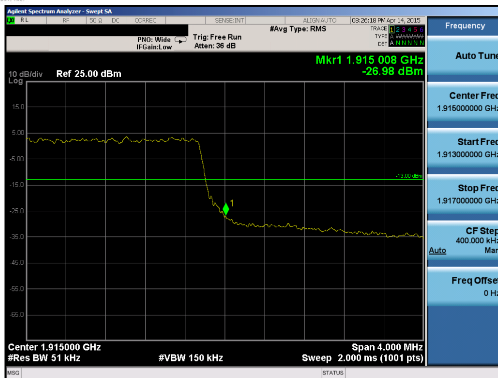
Plot 6-139. Upper Band Edge Plot (Band 25 – 5.0MHz QPSK – RB Size 25)
