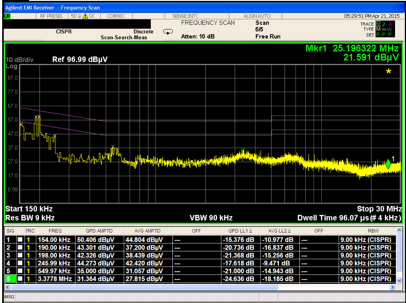
Plot 7-2. Line Conducted Plot (LN)
