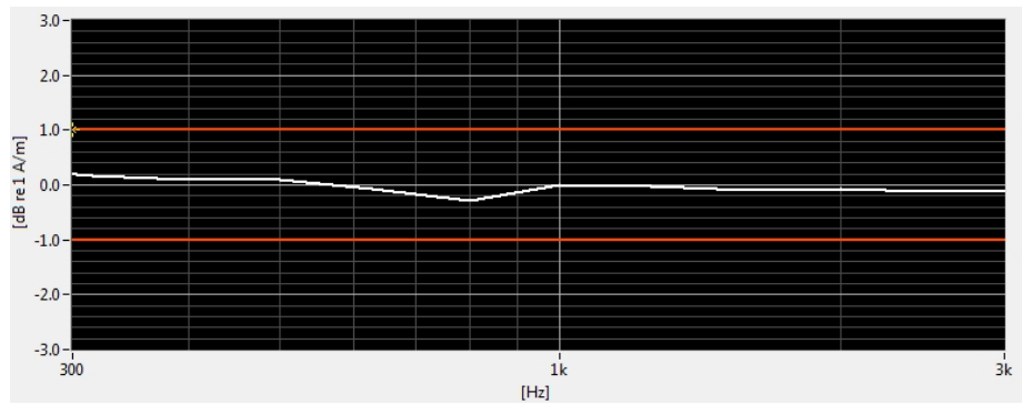
Figure 6-3 Helmholtz Coil Validation for Frequency Response
