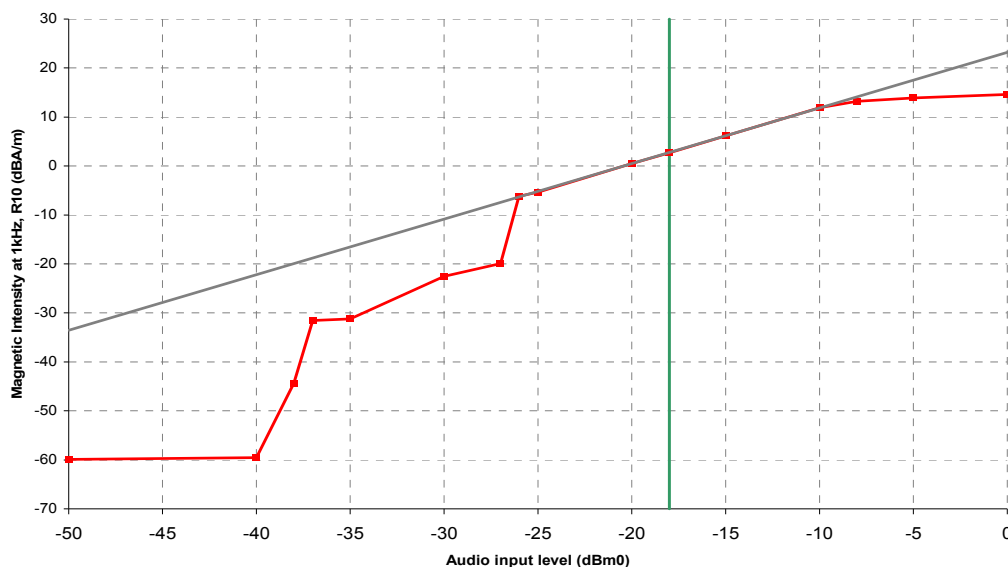
CDMA2000 Pure Tone suppression characterization (example)
