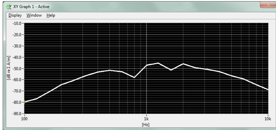
Figure 6-2 Worst-case ABM2 Plot for CDMA
