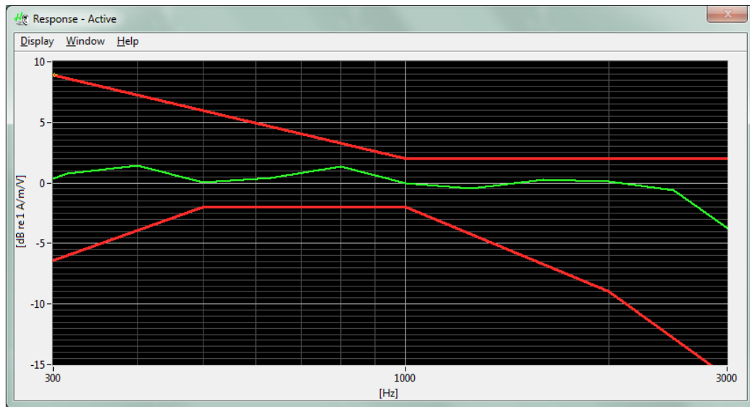
Figure 6-1 Axial Frequency Response
