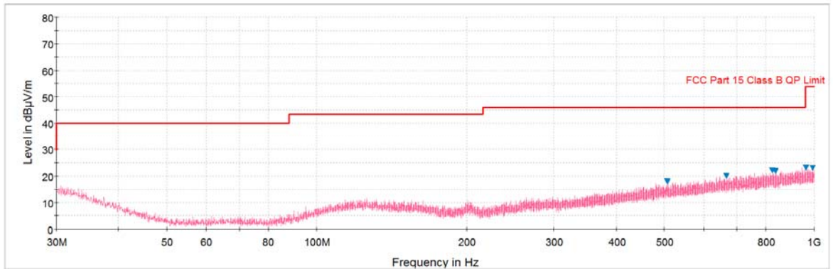
Plot 6-43. Radiated Spurious Plot below 1GHz (Pol. H)
