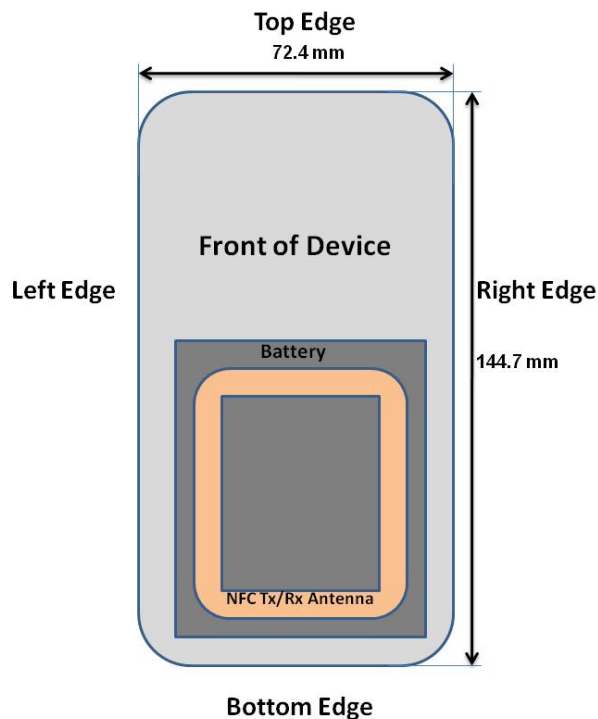
Figure F-2 NFC Antenna Locations
