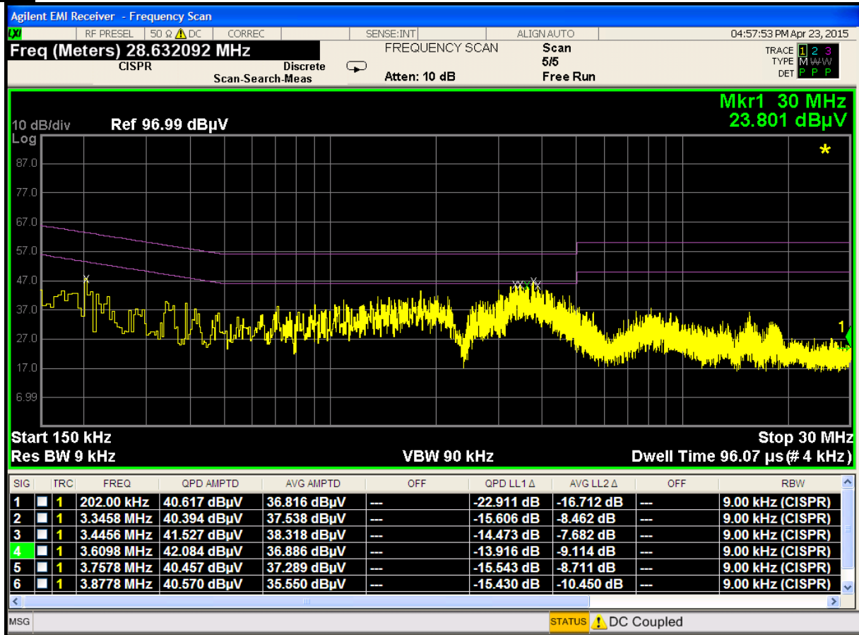
Plot 6-54. Line-Conducted Test Plot (L1)
