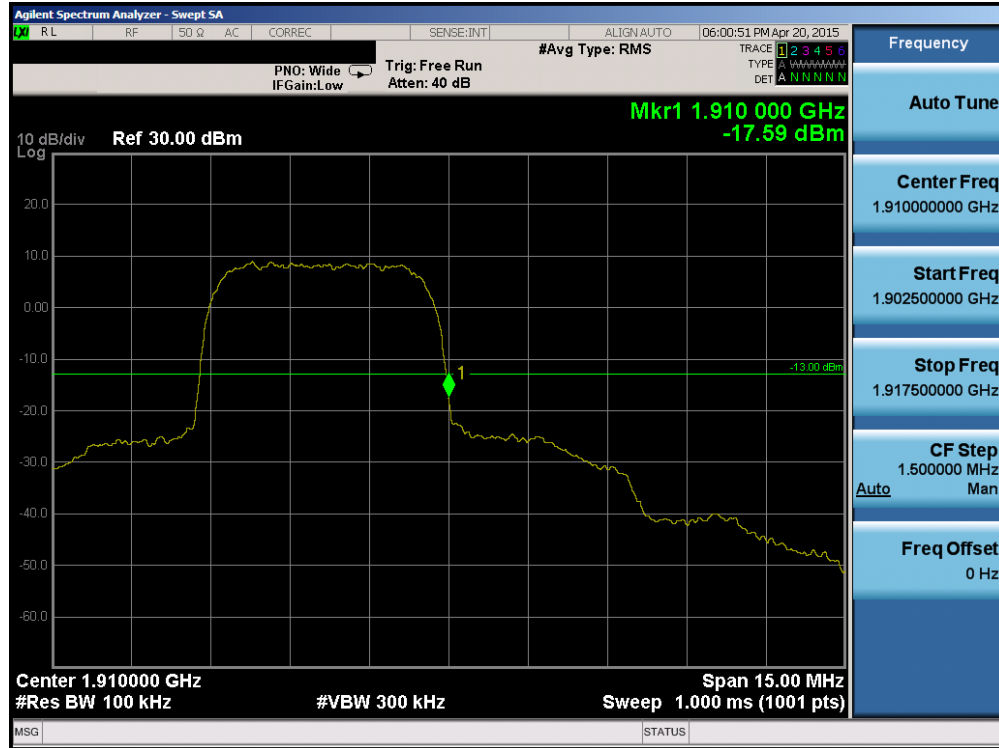
Plot 6-67. Band Edge Plot (PCS WCDMA Mode – Ch. 9538)
