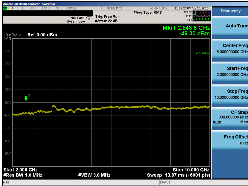
Plot 6-67. Conducted Spurious Plot (Band 5 – 1.4MHz QPSK – RB Size 1, RB Offset 0 – High Channel)
