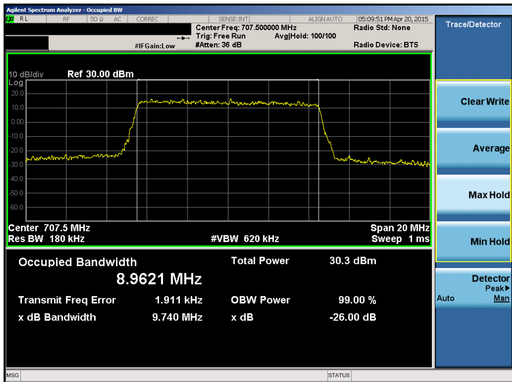
Plot 6-8. Occupied Bandwidth Plot (Band 12/17 – 10.0MHz 16-QAM – RB Size 50)
