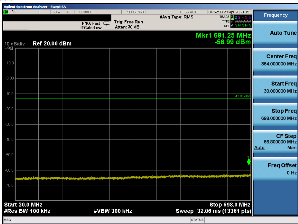
Plot 6-47. Conducted Spurious Plot (Band 12 – 1.4MHz QPSK – RB Size 1, RB Offset 0 – High Channel)
