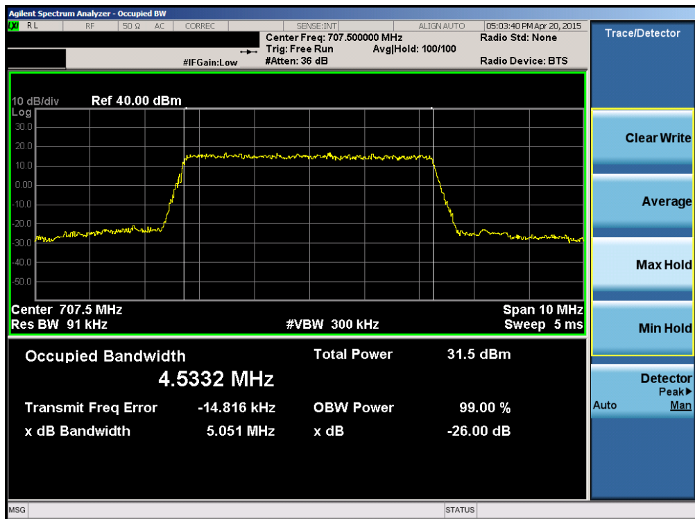
Plot 6-6. Occupied Bandwidth Plot (Band 12/17 – 5.0MHz 16-QAM – RB Size 25)
