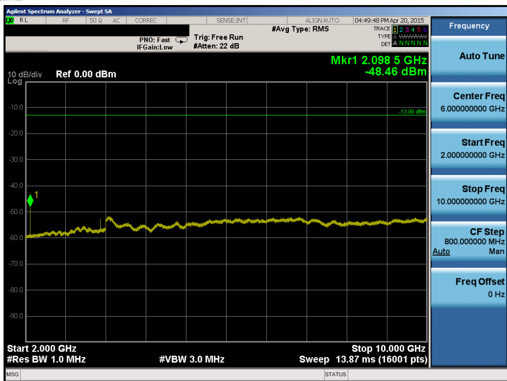
Plot 6-43. Conducted Spurious Plot (Band 12 – 1.4MHz QPSK – RB Size 1, RB Offset 0 – Low Channel)
