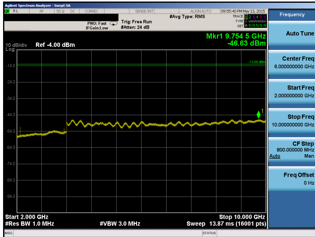
Plot 6-52. Conducted Spurious Plot (Band 17 – 10MHz QPSK – RB Size 1, RB Offset 0 – Low Channel)
