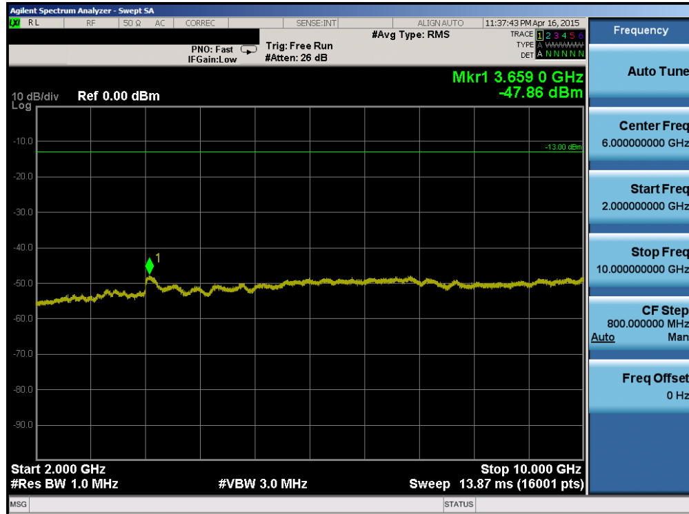
Plot 6-61. Conducted Spurious Plot (Band 5 – 1.4MHz QPSK – RB Size 1, RB Offset 0 – Low Channel)
