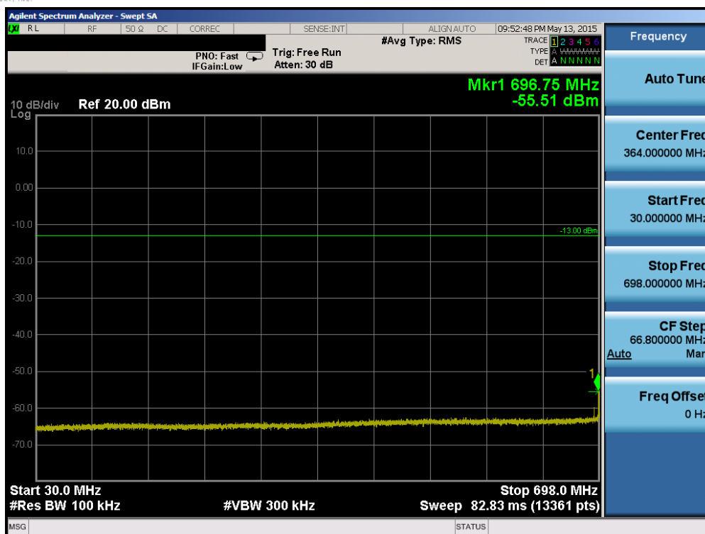
Plot 6-53. Conducted Spurious Plot (Band 17 – 10MHz QPSK – RB Size 1, RB Offset 0 – Mid Channel)
