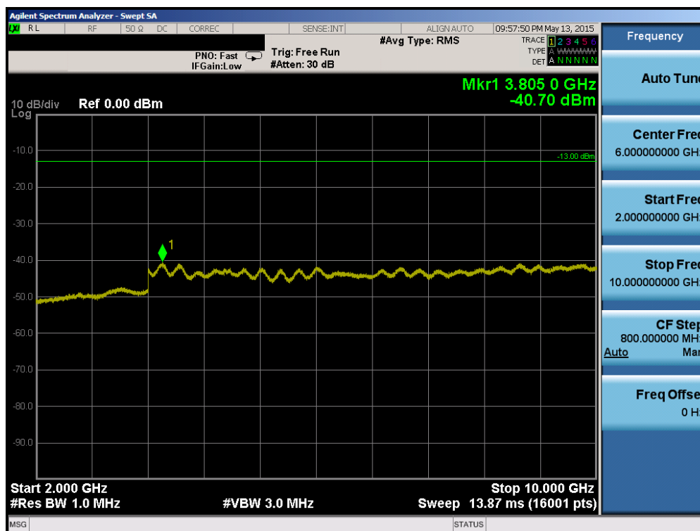
Plot 6-58. Conducted Spurious Plot (Band 17 – 10MHz QPSK – RB Size 1, RB Offset 0 – High Channel)
