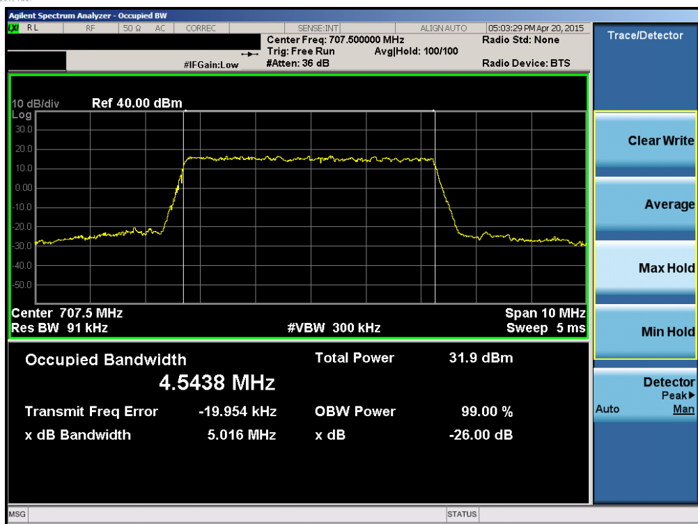
Plot 6-5. Occupied Bandwidth Plot (Band 12/17 – 5.0MHz QPSK – RB Size 25)
