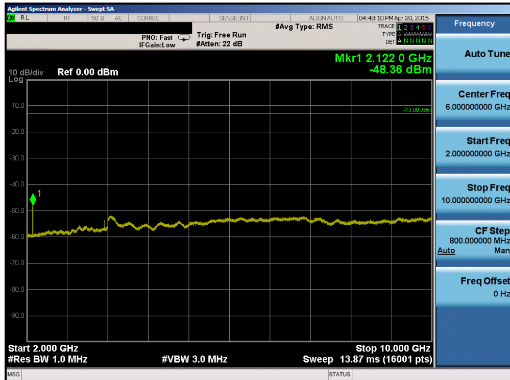
Plot 6-46. Conducted Spurious Plot (Band 12 – 1.4MHz QPSK – RB Size 1, RB Offset 0 – Mid Channel)
