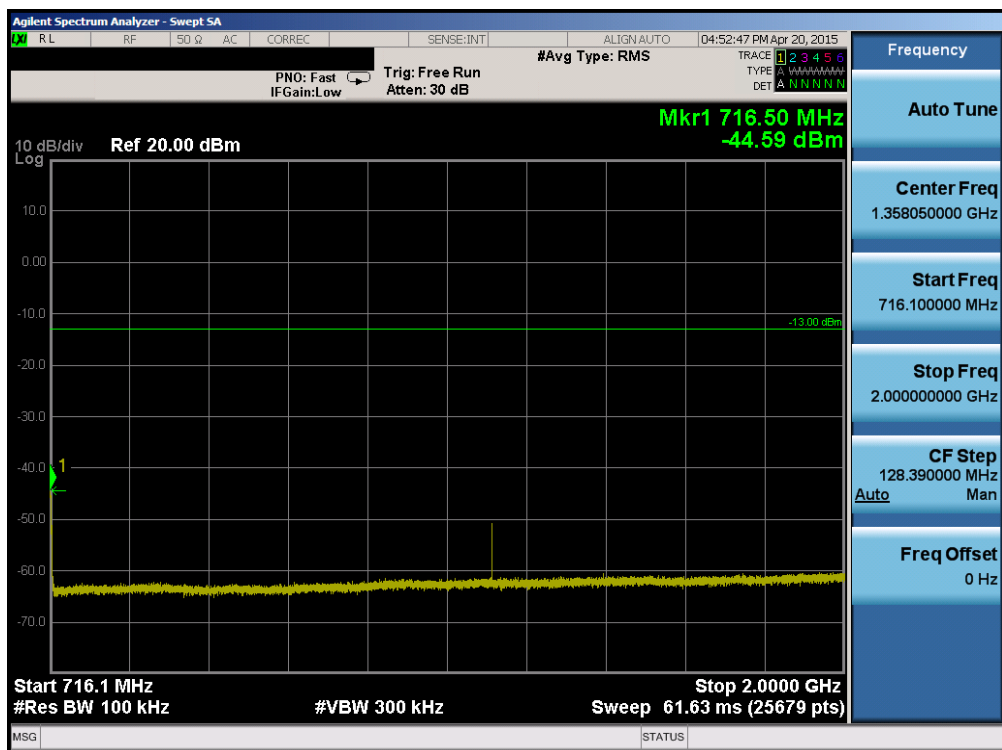
Plot 6-48. Conducted Spurious Plot (Band 12 – 1.4MHz QPSK – RB Size 1, RB Offset 0 – High Channel)
