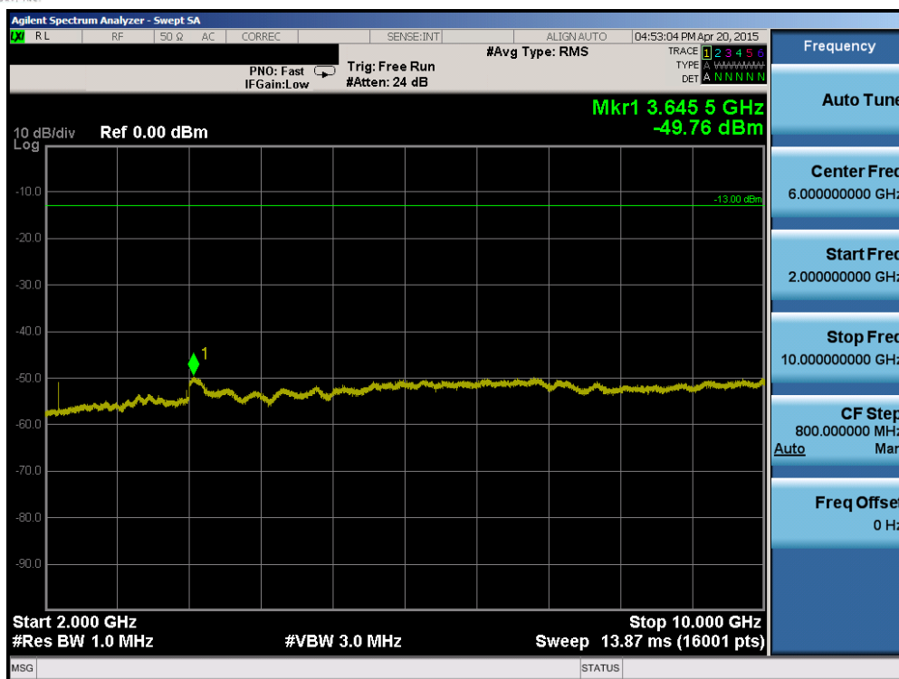
Plot 6-49. Conducted Spurious Plot (Band 12 – 1.4MHz QPSK – RB Size 1, RB Offset 0 – High Channel)
