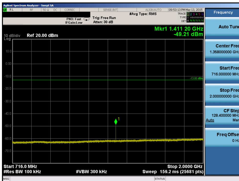
Plot 6-54. Conducted Spurious Plot (Band 17 – 10MHz QPSK – RB Size 1, RB Offset 0 – Mid Channel)
