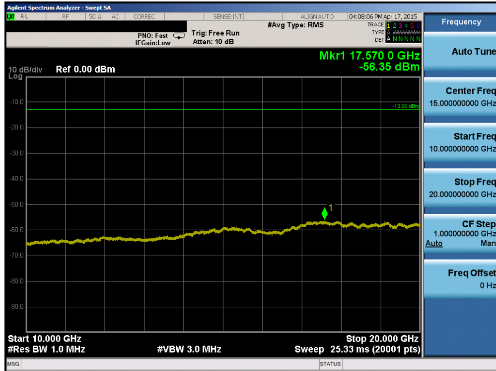
Plot 6-79. Conducted Spurious Plot (Band 2 – 5.0MHz QPSK – RB Size 1, RB Offset 0 – Low Channel)
