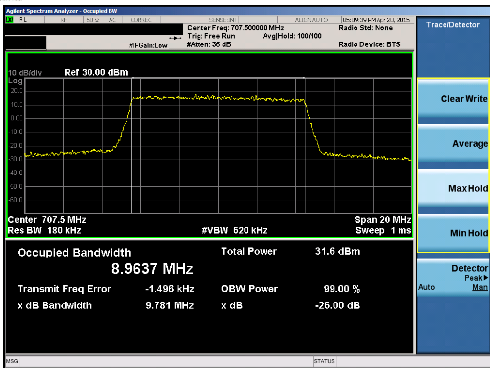
Plot 6-7. Occupied Bandwidth Plot (Band 12/17 – 10.0MHz QPSK – RB Size 50)
