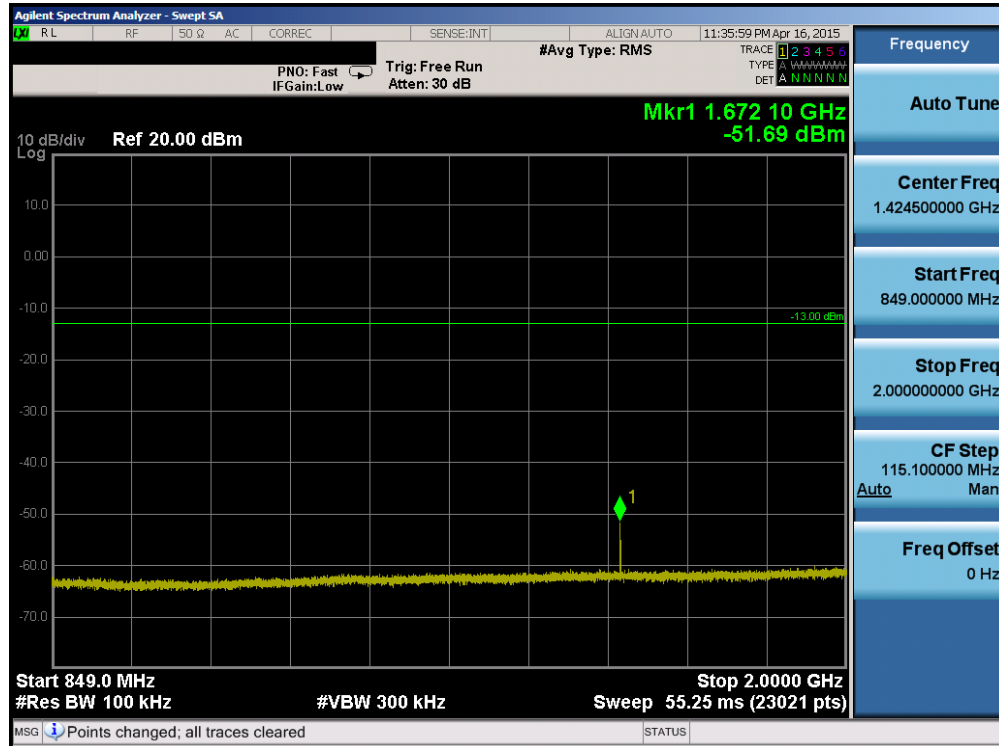
Plot 6-63. Conducted Spurious Plot (Band 5 – 1.4MHz QPSK – RB Size 1, RB Offset 0 – Mid Channel)
