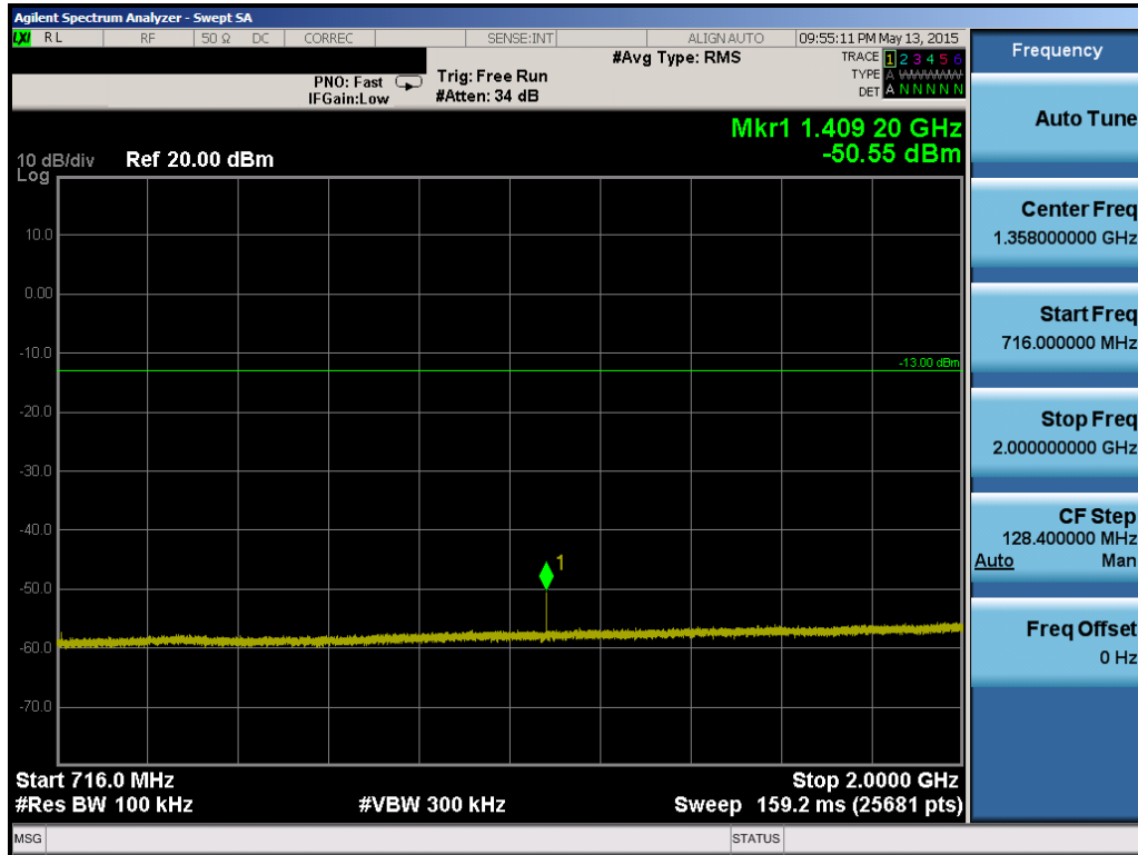
Plot 6-51. Conducted Spurious Plot (Band 17 – 10MHz QPSK – RB Size 1, RB Offset 0 – Low Channel)
