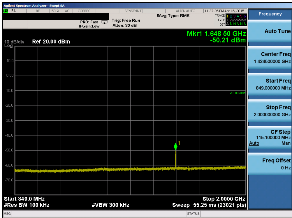
Plot 6-60. Conducted Spurious Plot (Band 5 – 1.4MHz QPSK – RB Size 1, RB Offset 0 – Low Channel)
