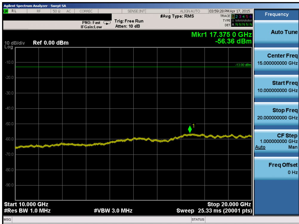
Plot 6-82. Conducted Spurious Plot (Band 2 – 5.0MHz QPSK – RB Size 1, RB Offset 0 – Mid Channel)
