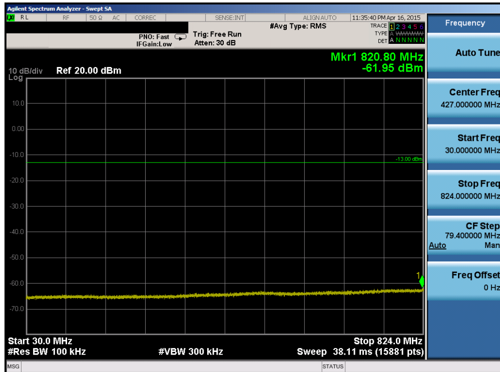
Plot 6-62. Conducted Spurious Plot (Band 5 – 1.4MHz QPSK – RB Size 1, RB Offset 0 – Mid Channel)
