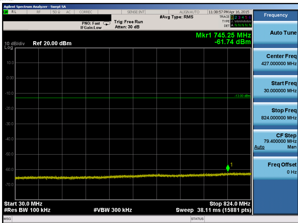
Plot 6-65. Conducted Spurious Plot (Band 5 – 1.4MHz QPSK – RB Size 1, RB Offset 0 – High Channel)
