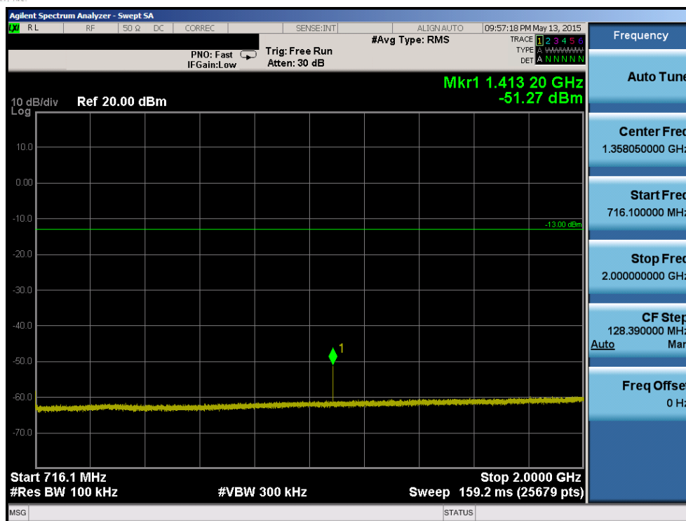
Plot 6-57. Conducted Spurious Plot (Band 17 – 10MHz QPSK – RB Size 1, RB Offset 0 – High Channel)
