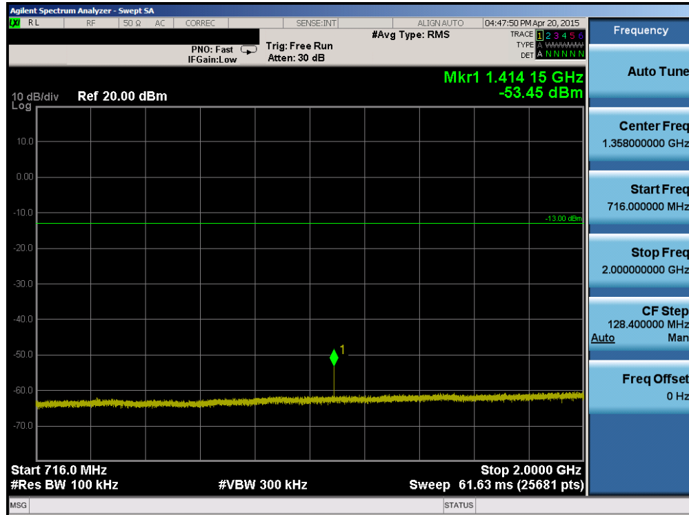
Plot 6-45. Conducted Spurious Plot (Band 12 – 1.4MHz QPSK – RB Size 1, RB Offset 0 – Mid Channel)
