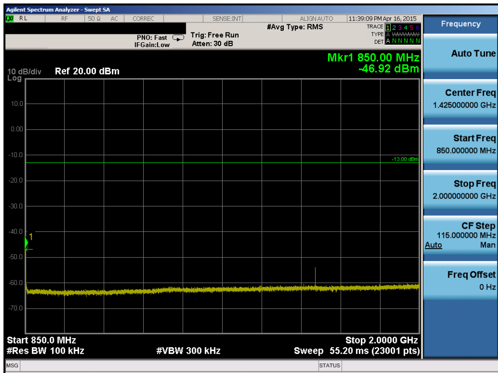
Plot 6-66. Conducted Spurious Plot (Band 5 – 1.4MHz QPSK – RB Size 1, RB Offset 0 – High Channel)
