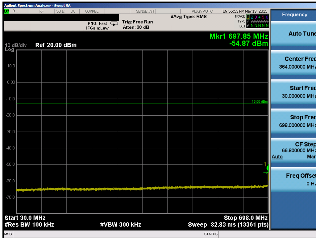
Plot 6-56. Conducted Spurious Plot (Band 17 – 10MHz QPSK – RB Size 1, RB Offset 0 – High Channel)
