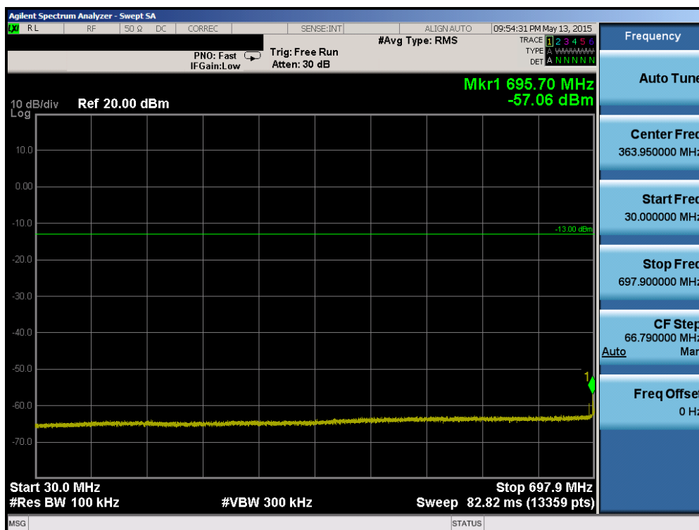
Plot 6-50. Conducted Spurious Plot (Band 17 – 10MHz QPSK – RB Size 1, RB Offset 0 – Low Channel)
