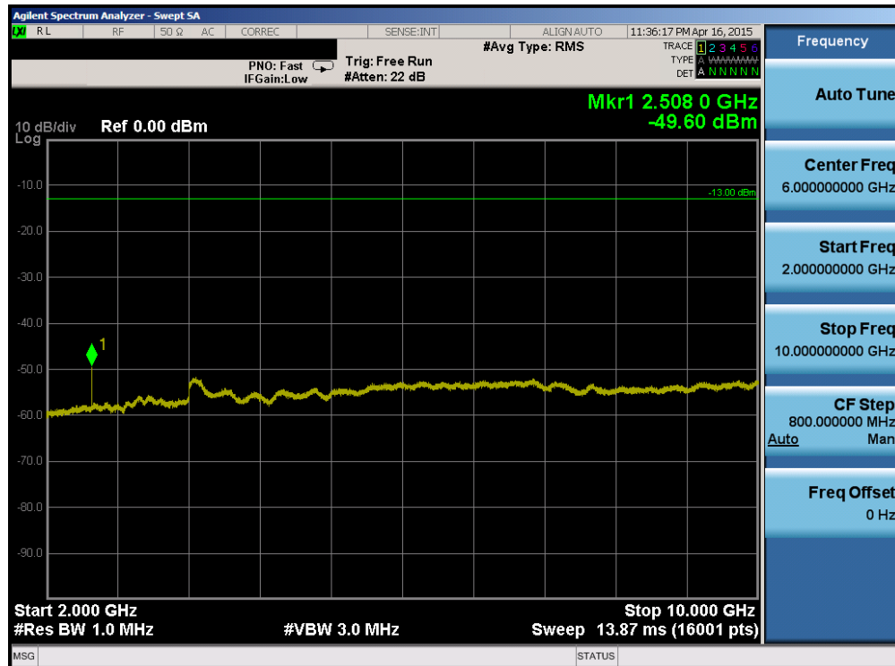
Plot 6-64. Conducted Spurious Plot (Band 5 – 1.4MHz QPSK – RB Size 1, RB Offset 0 – Mid Channel)
