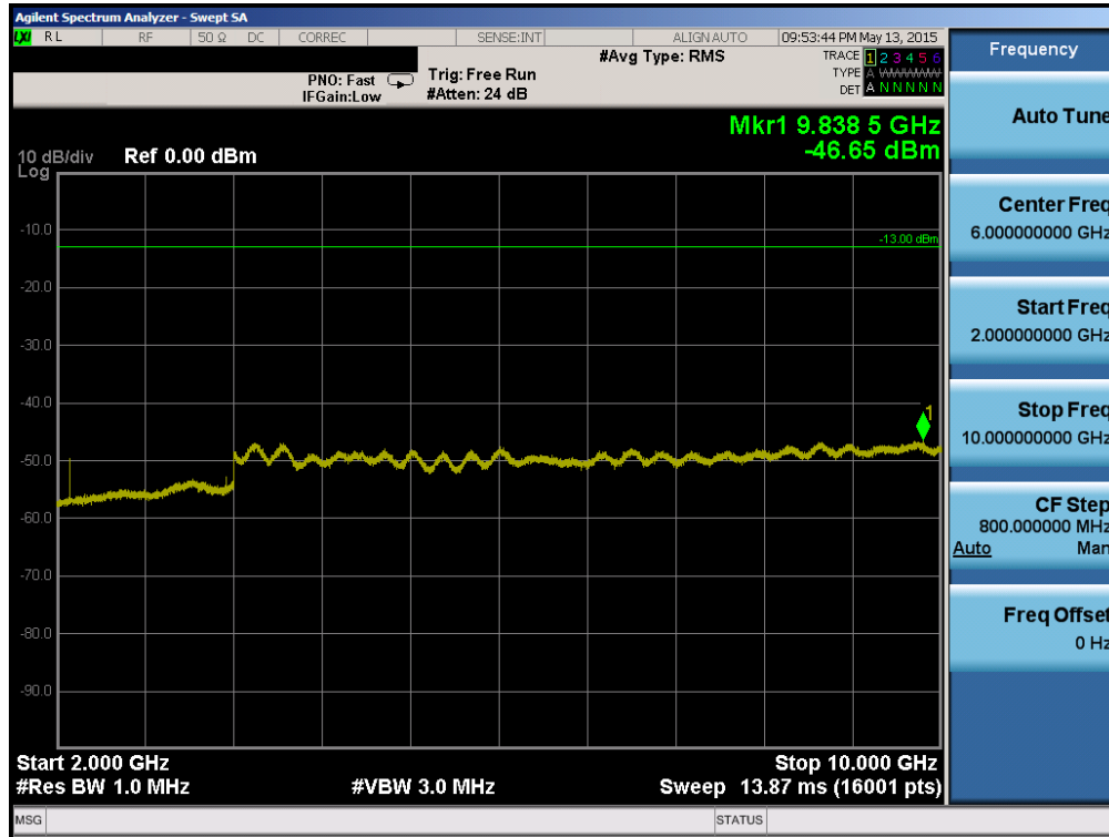
Plot 6-55. Conducted Spurious Plot (Band 17 – 10MHz QPSK – RB Size 1, RB Offset 0 – Mid Channel)
