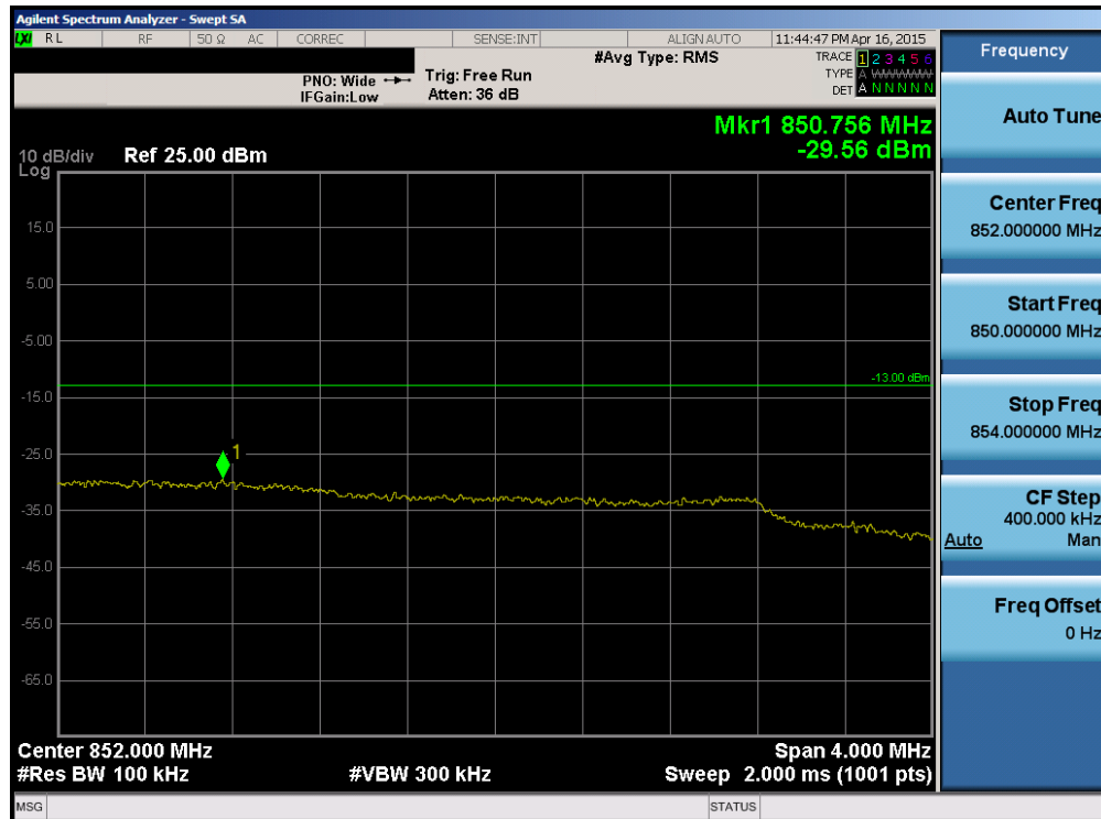
Plot 6-108. Upper Extended Band Edge Plot (Band 5 - 5.0MHz QPSK - RB Size 25)
