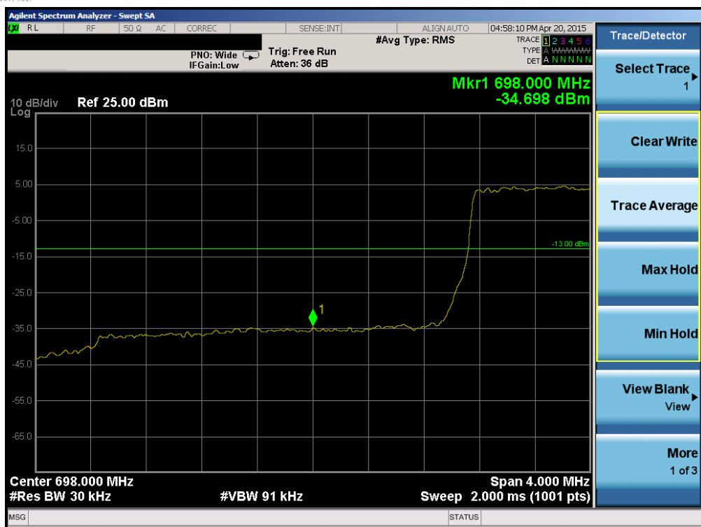
Plot 6-87. Lower Band Edge Plot (Band 12 – 3.0MHz QPSK – RB Size 15)
