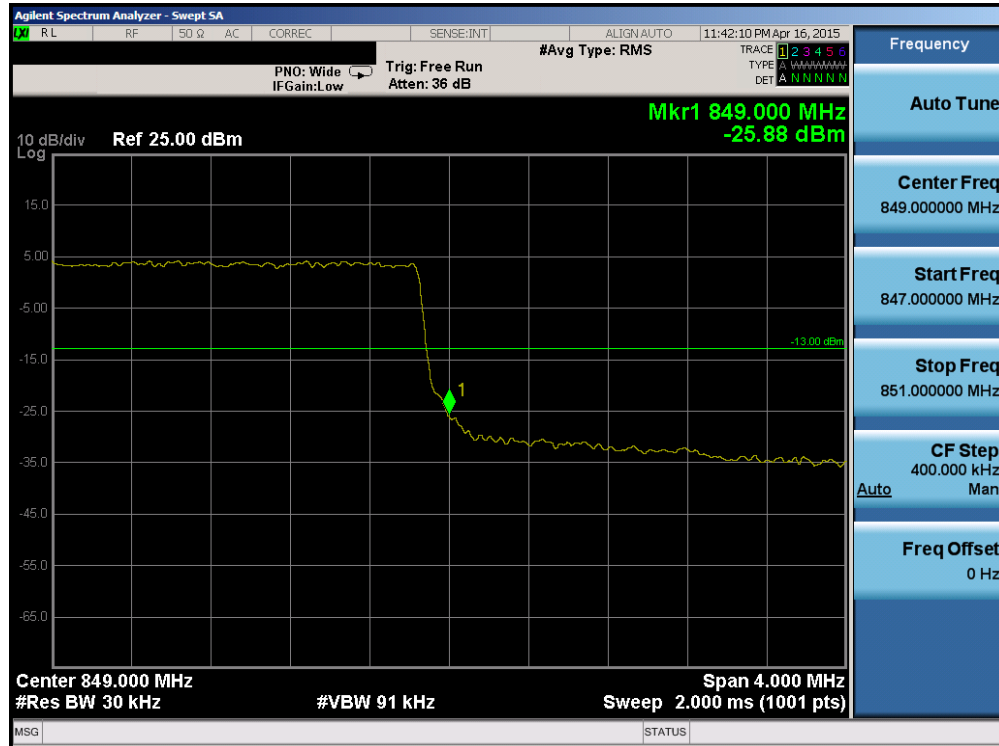
Plot 6-103. Upper Band Edge Plot (Band 5 - 3.0MHz QPSK - RB Size 15)
