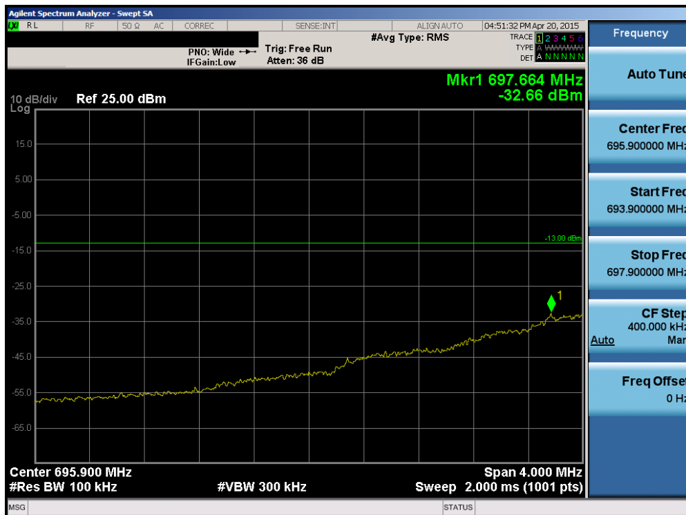
Plot 6-84. Lower Extended Band Edge Plot (Band 12 – 1.4MHz QPSK – RB Size 6)
