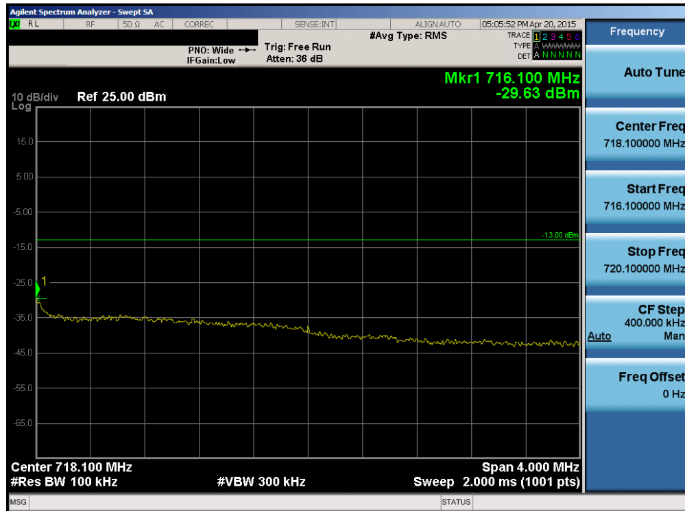
Plot 6-94. Upper Extended Band Edge Plot (Band 12/17 – 5.0MHz QPSK – RB Size 25)
