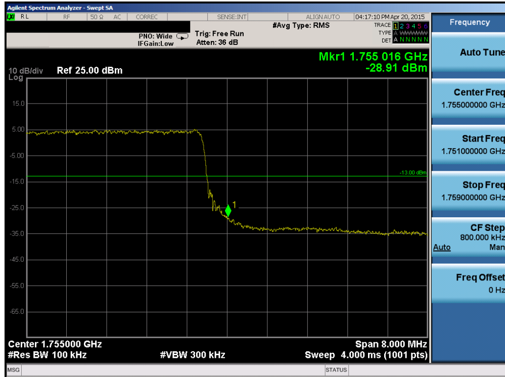
Plot 6-125. Upper Band Edge Plot (Band 4 – 10.0MHz QPSK – RB Size 50)
