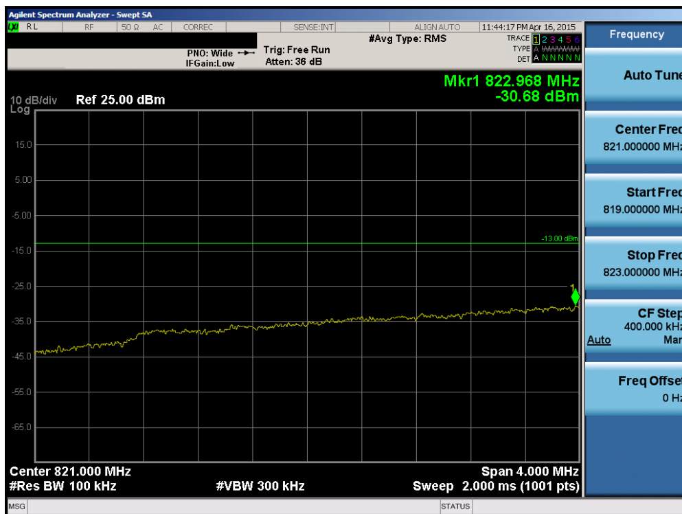
Plot 6-106. Lower Extended Band Edge Plot (Band 5 – 5.0MHz QPSK – RB Size 25)
