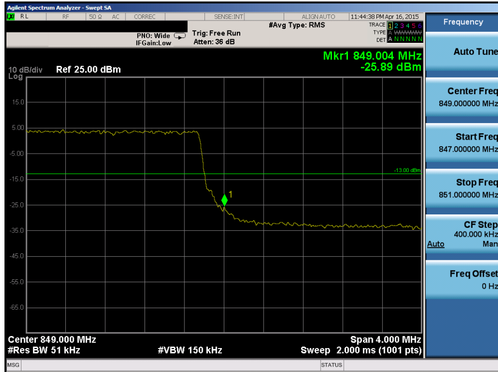
Plot 6-107. Upper Band Edge Plot (Band 5 - 5.0MHz QPSK - RB Size 25)
