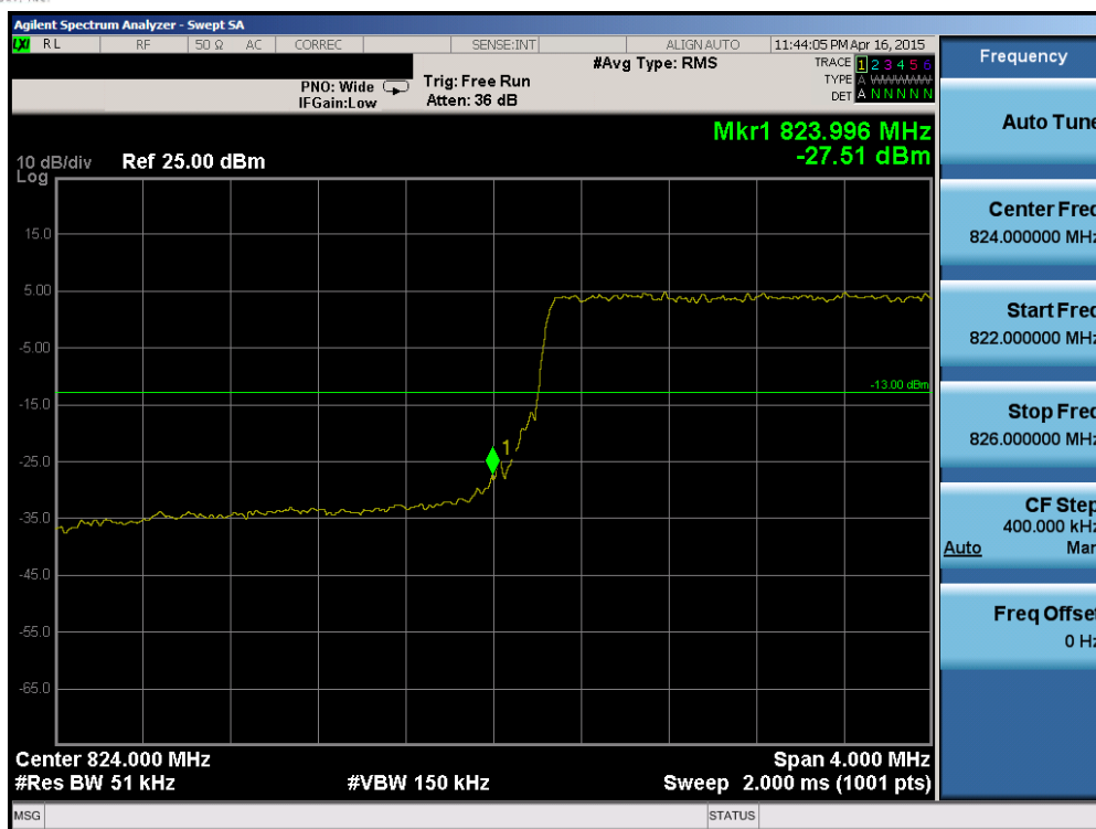
Plot 6-105. Lower Band Edge Plot (Band 5 – 5.0MHz QPSK – RB Size 25)
