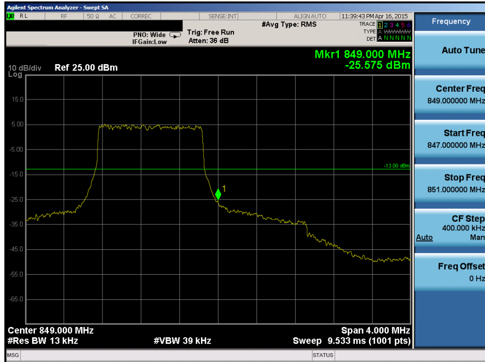
Plot 6-99. Upper Band Edge Plot (Band 5 – 1.4MHz QPSK – RB Size 6)
