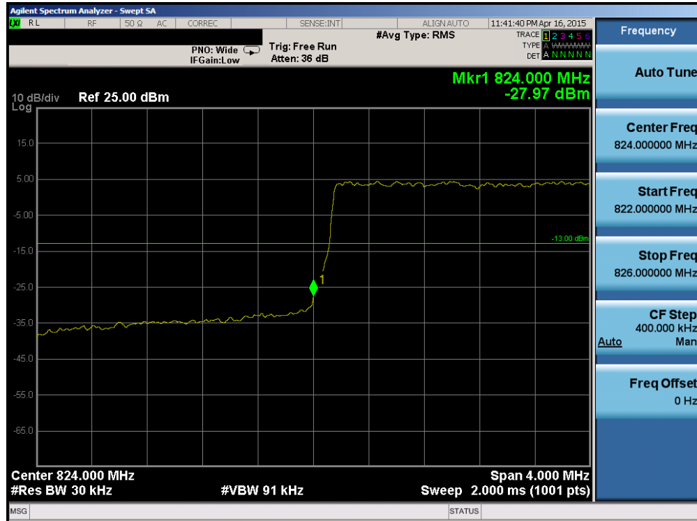
Plot 6-101. Lower Band Edge Plot (Band 5 – 3.0MHz QPSK – RB Size 15)
