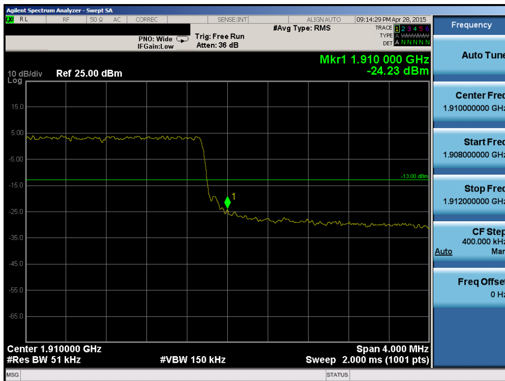
Plot 6-145. Upper Band Edge Plot (Band 2 – 5.0MHz QPSK – RB Size 25)
