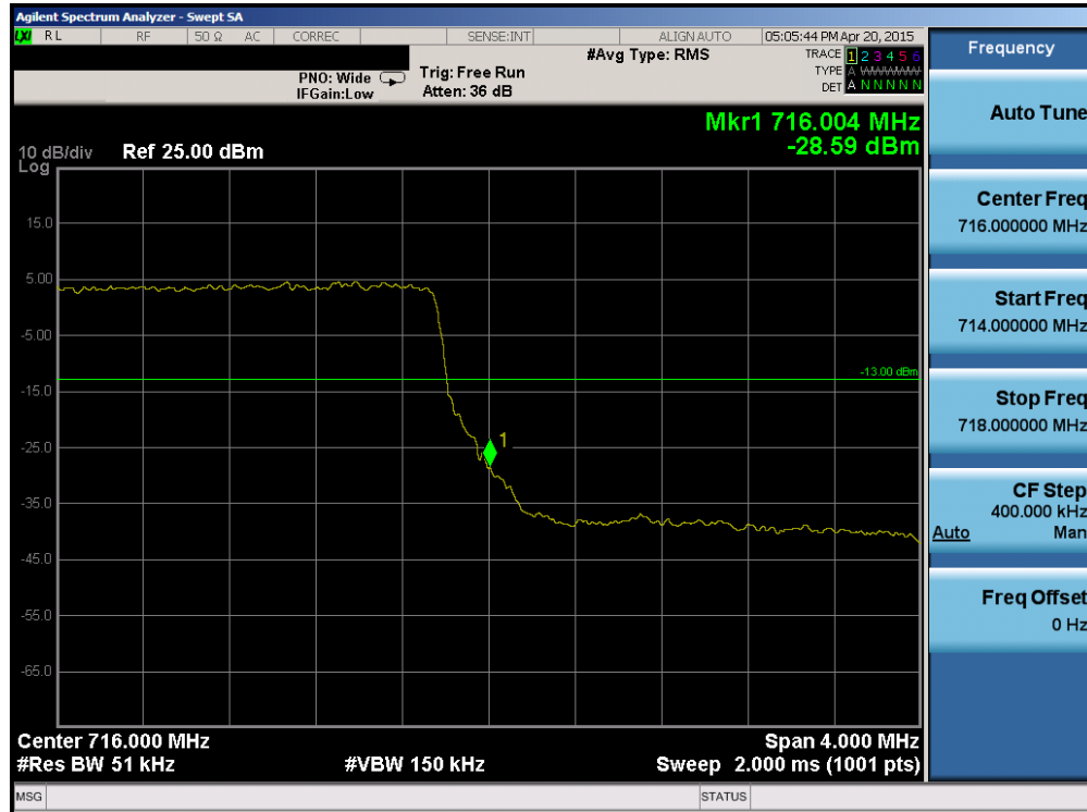
Plot 6-93. Upper Band Edge Plot (Band 12/17 – 5.0MHz QPSK – RB Size 25)
