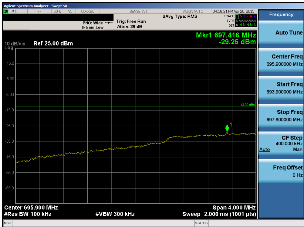
Plot 6-88. Lower Extended Band Edge Plot (Band 12 – 3.0MHz QPSK – RB Size 15)
