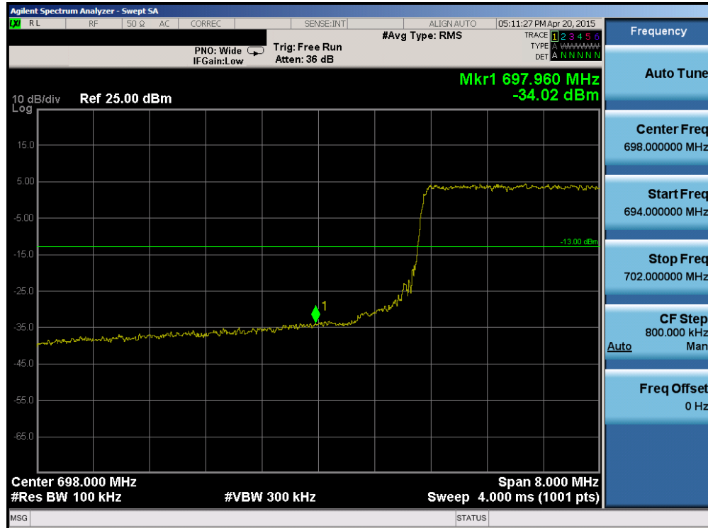
Plot 6-95. Lower Band Edge Plot (Band 12/17 – 10.0MHz QPSK – RB Size 50)
