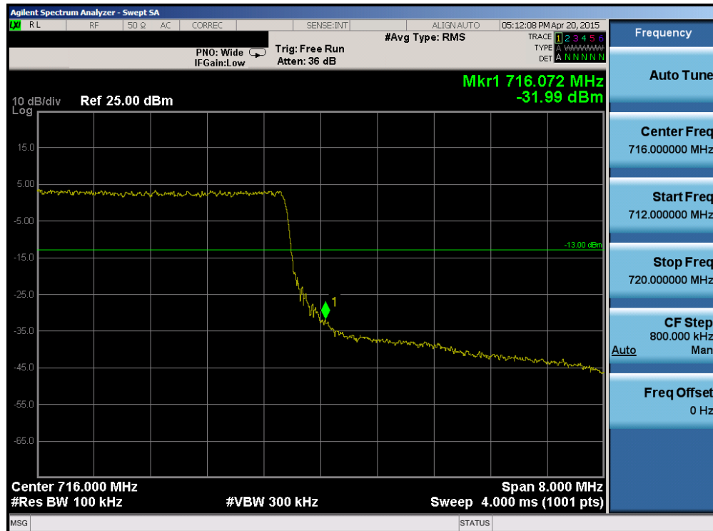
Plot 6-96. Upper Band Edge Plot (Band 12/17 – 10.0MHz QPSK – RB Size 50)
