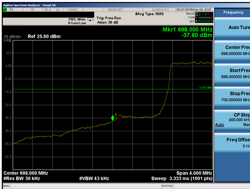
Plot 6-83. Lower Band Edge Plot (Band 12 – 1.4MHz QPSK – RB Size 6)
