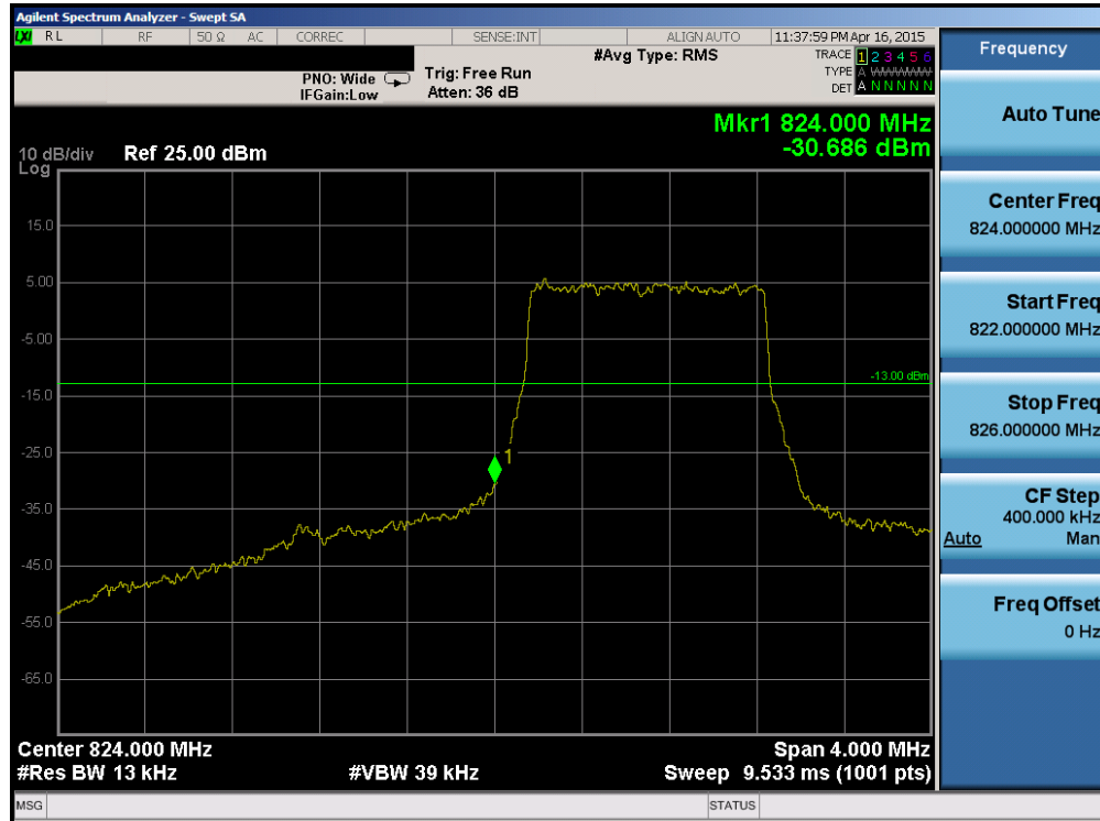
Plot 6-97. Lower Band Edge Plot (Band 5 – 1.4MHz QPSK – RB Size 6)
