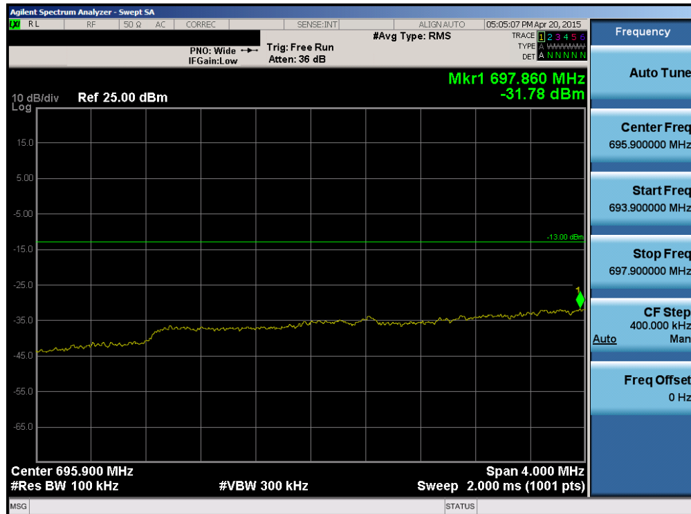
Plot 6-92. Lower Extended Band Edge Plot (Band 12/17 – 5.0MHz QPSK – RB Size 25)
