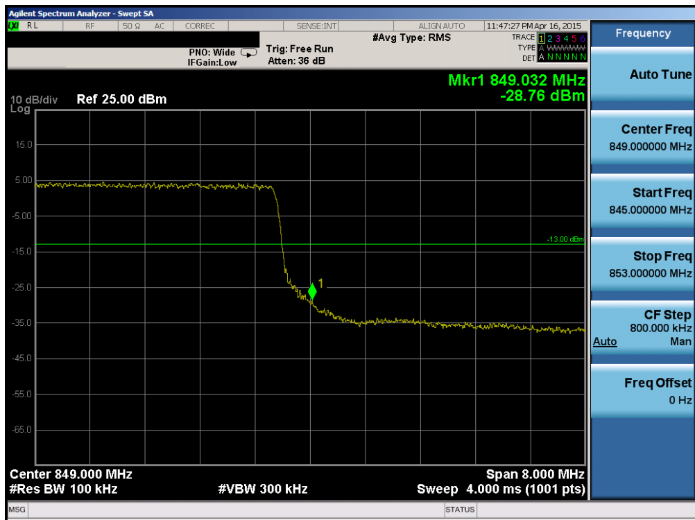
Plot 6-110. Upper Band Edge Plot (Band 5 – 10.0MHz QPSK – RB Size 50)
