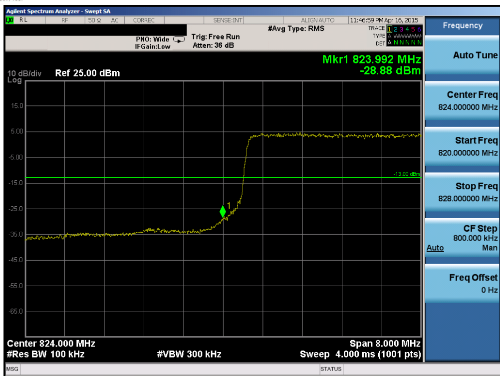
Plot 6-109. Lower Band Edge Plot (Band 5 – 10.0MHz QPSK – RB Size 50)
