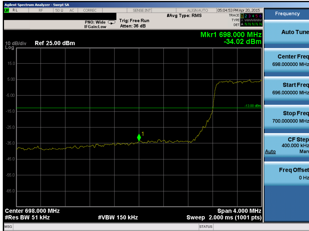
Plot 6-91. Lower Band Edge Plot (Band 12/17 – 5.0MHz QPSK – RB Size 25)
